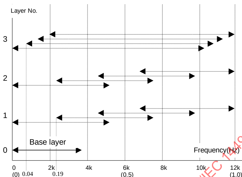
Figure 4.30 – Example of adaptive active band selection. (Sampling_Frequency=24kHz, Total bitrate=40kbit/s(8+8+8+16kbps) In this case, q_{\text{sample}} = 0.43 , \text{bias} = 0.19 for layer 1 and layer 2 q_{\text{sample}} = 0.87 , \text{bias} = 0.04 for layer 3)
