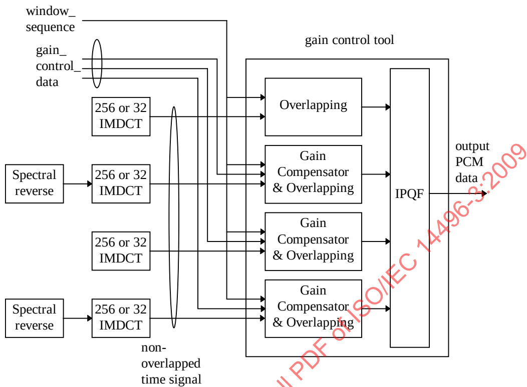
Figure 4.34 – Block diagram of gain control tool
