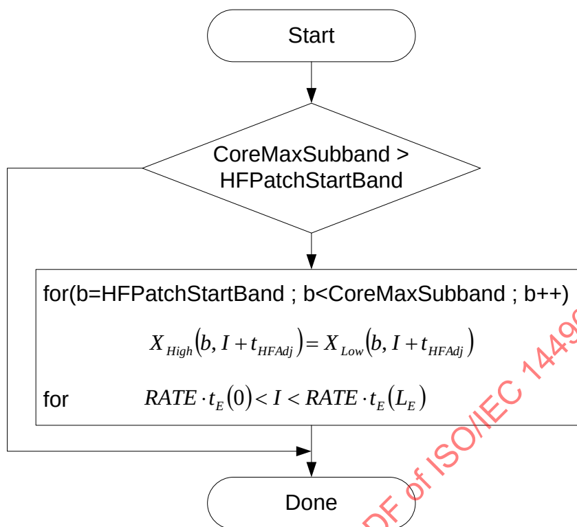
Figure 4.125 – Flowchart of HF-Overlap
