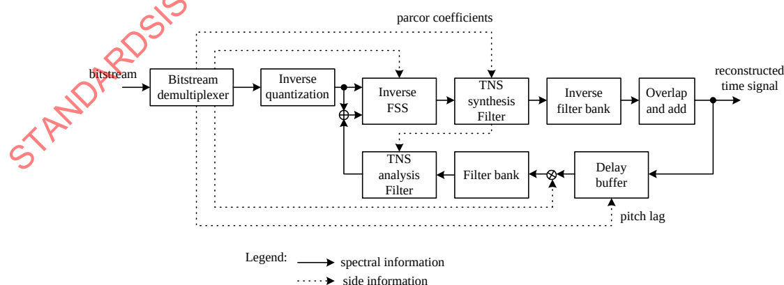
Figure 4.37 – Decoder structure
