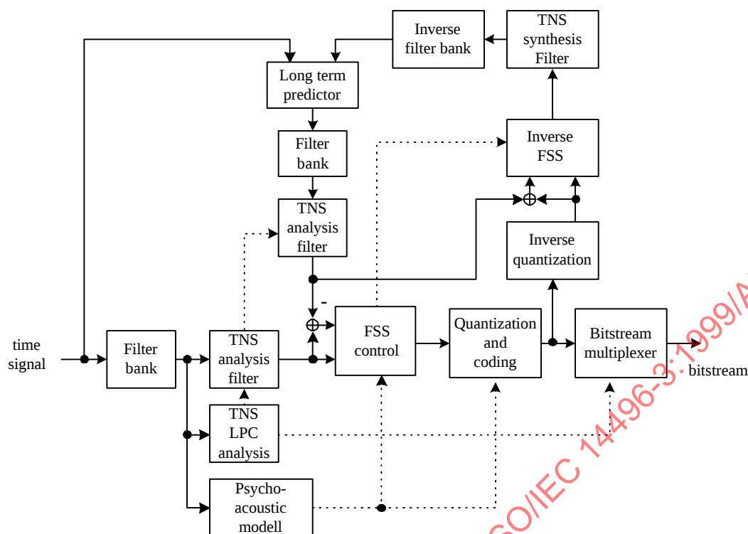
Figure 14: Encoder structure
