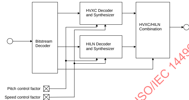
Figure 4: Block diagram of the integrated parametric decoder
