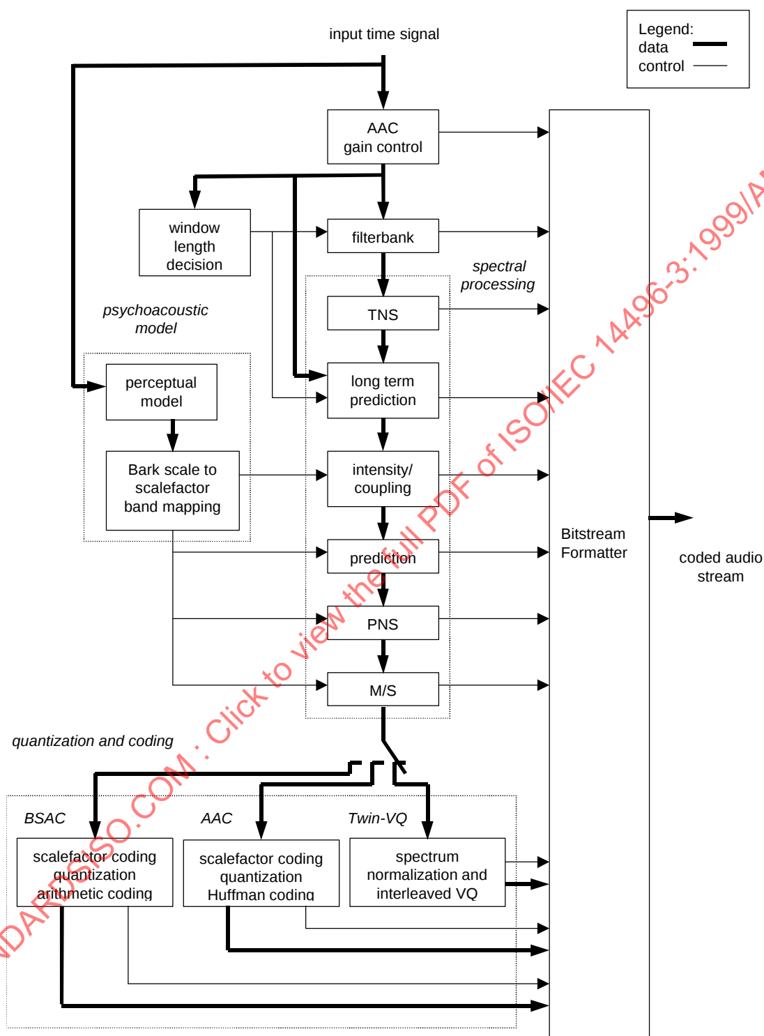
Figure 5: Block diagram of GA non scalable encoder
