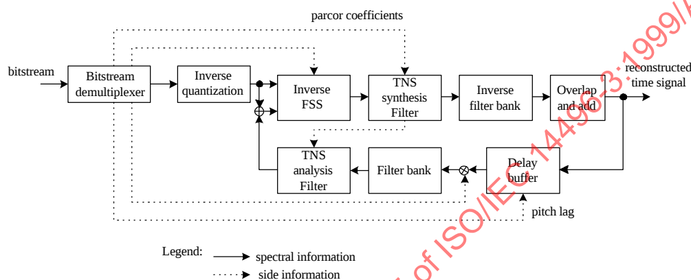
Figure 13: Decoder structure
