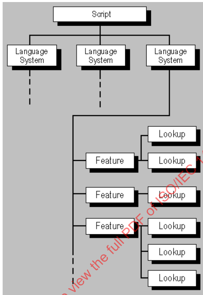
Figure 6.9 – The relationship of scripts, language systems, features, and lookups for substitution and positioning tables
