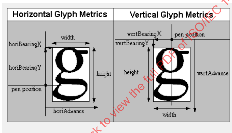
Figure 3 – Glyph metrics
