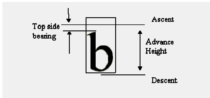
Figure 4 – Vertical Metrics
