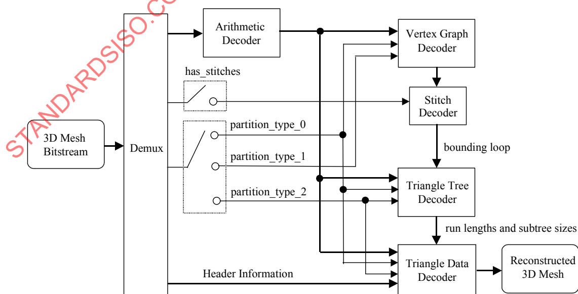
Figure V2 - 40 -- Block diagram of the Topological Surgery decoder
