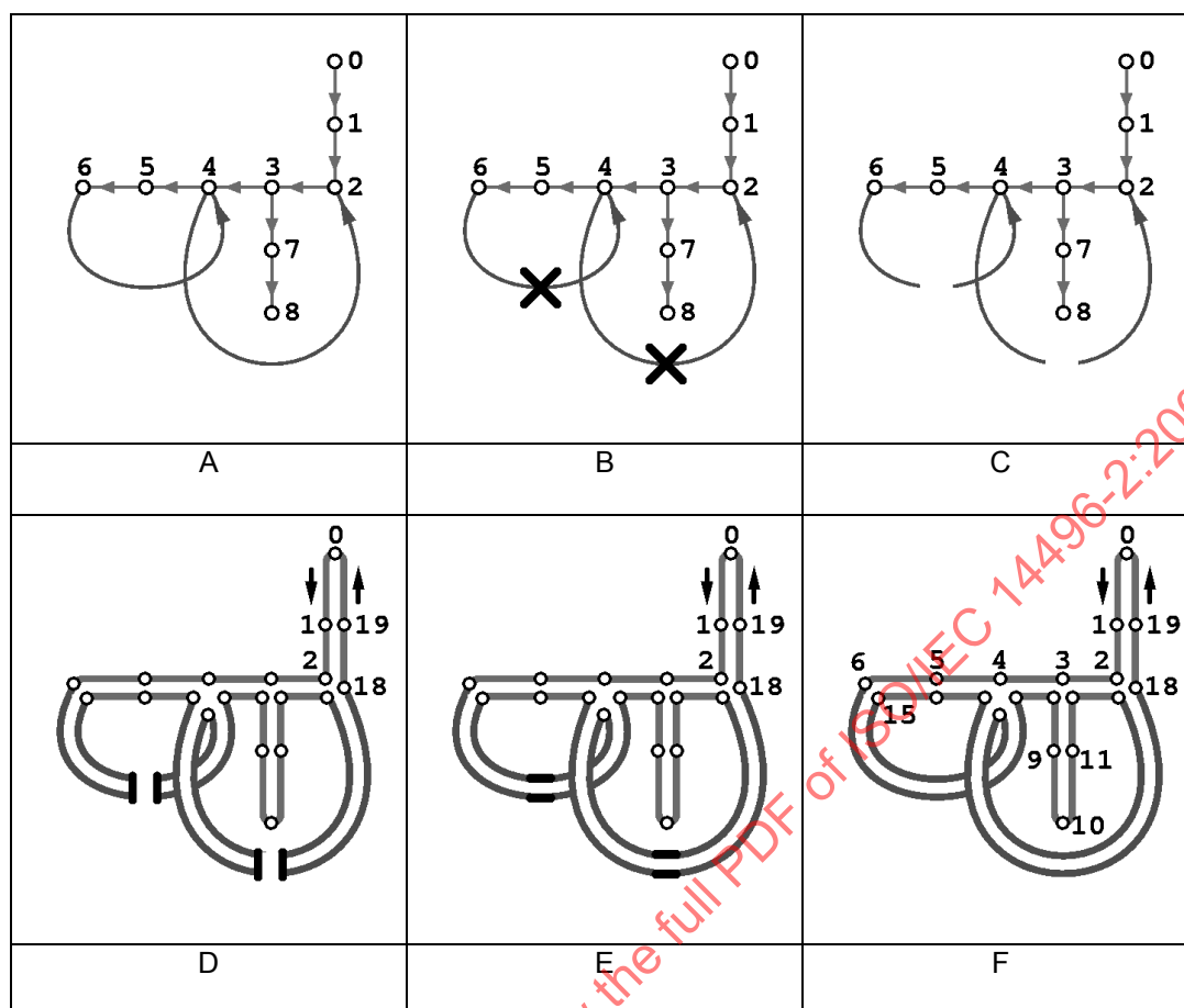
Figure V2 -46 -- Steps to build the bounding loop from the vertex graph.
