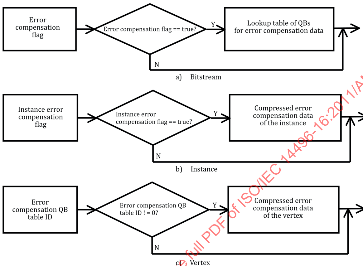
Figure Amd4.13 — Information related with error compensation
