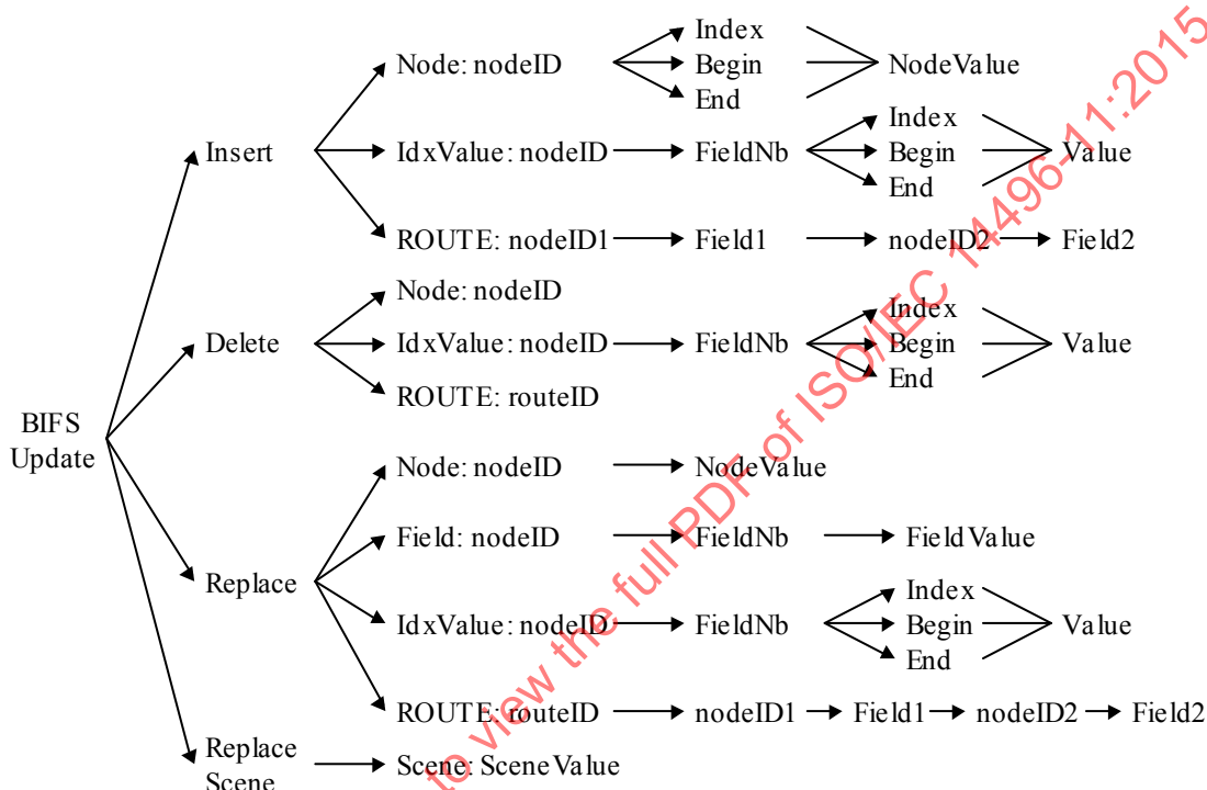
Figure 10 — BIFS-Command Types
