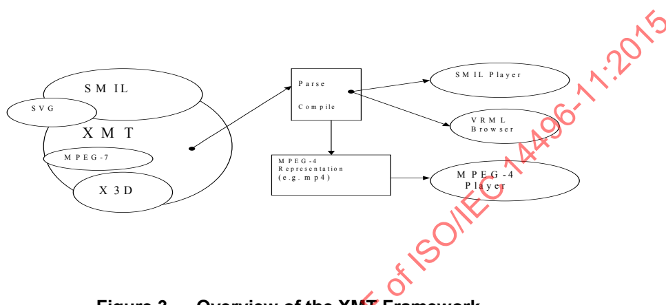
Figure 3 — Overview of the XMT Framework
