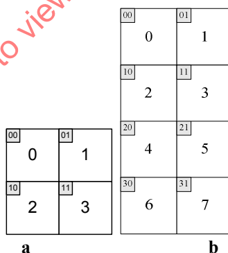
Figure 8-7 – Assignment of the indices of dcC to \text{chroma4x4BlkIdx} : (a) ChromaArrayType equal to 1, (b) ChromaArrayType equal to 2
