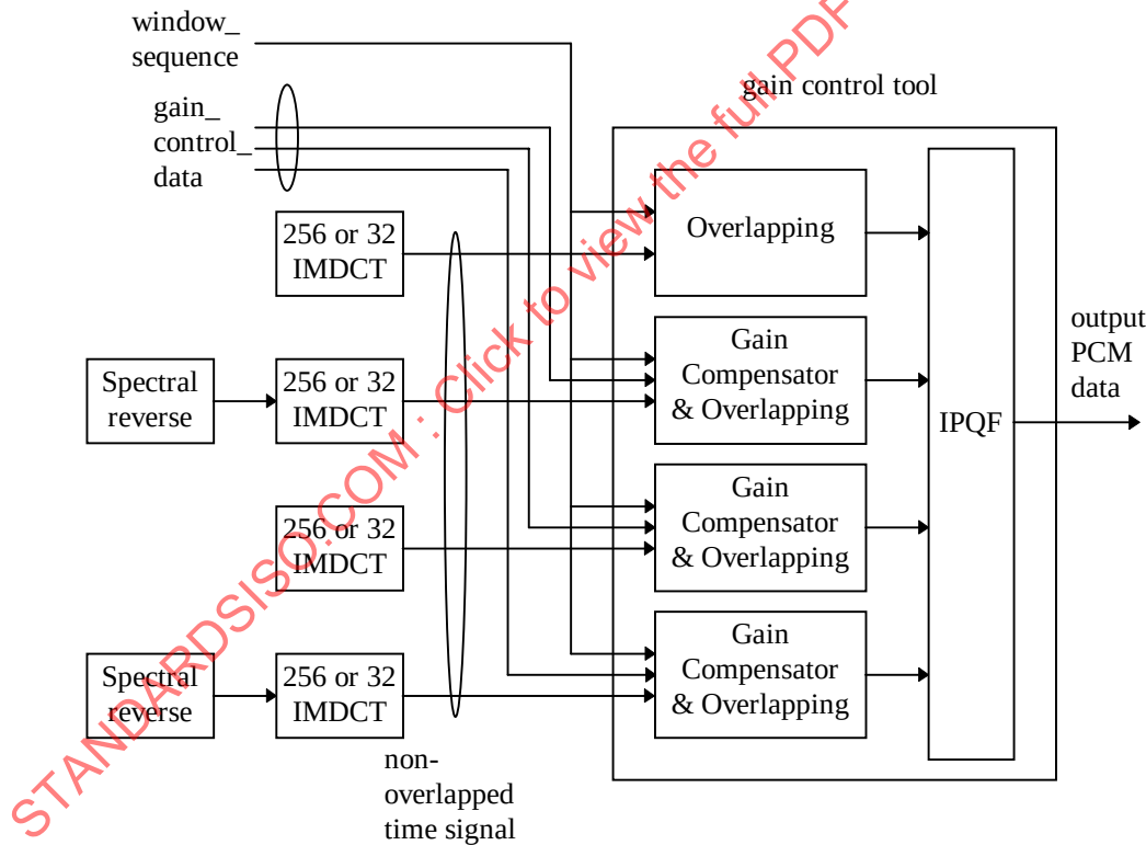
Figure 4.33 – Block diagram of gain control tool
