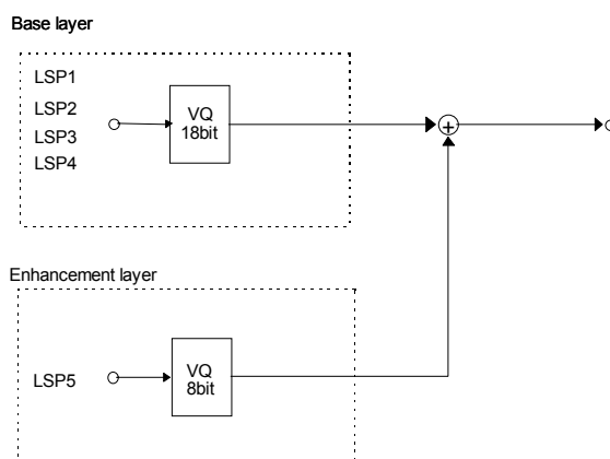
Figure 2.5 — LSP decoder
