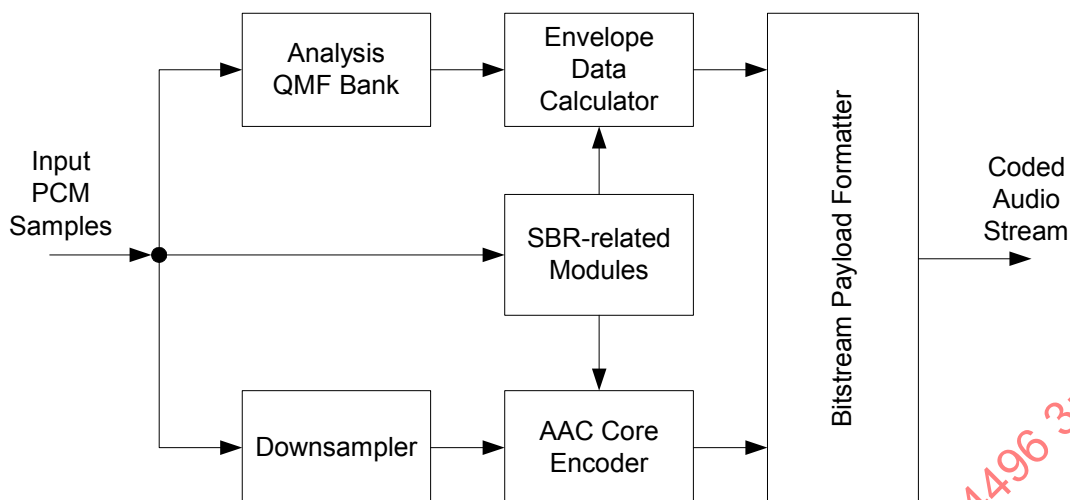
Figure 4.B.11 – Encoder overview
