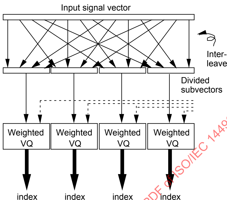
Figure 4.B.3 – Weighted interleaved vector quantization.
