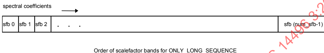
Figure 4.18 – Order of scalefactor bands for ONLY_LONG_SEQUENCE
