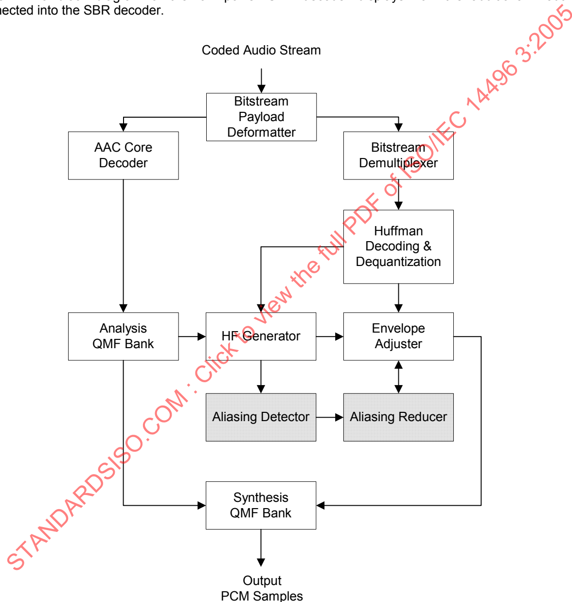
Figure 4.47 – Block diagram of the SBR low power decoder
