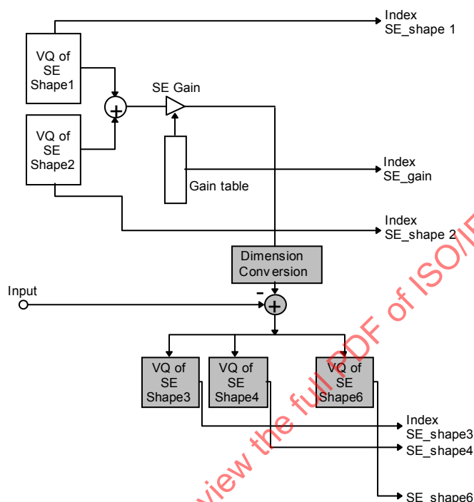
Figure 2.A.2 — Vector quantization of spectral envelope
