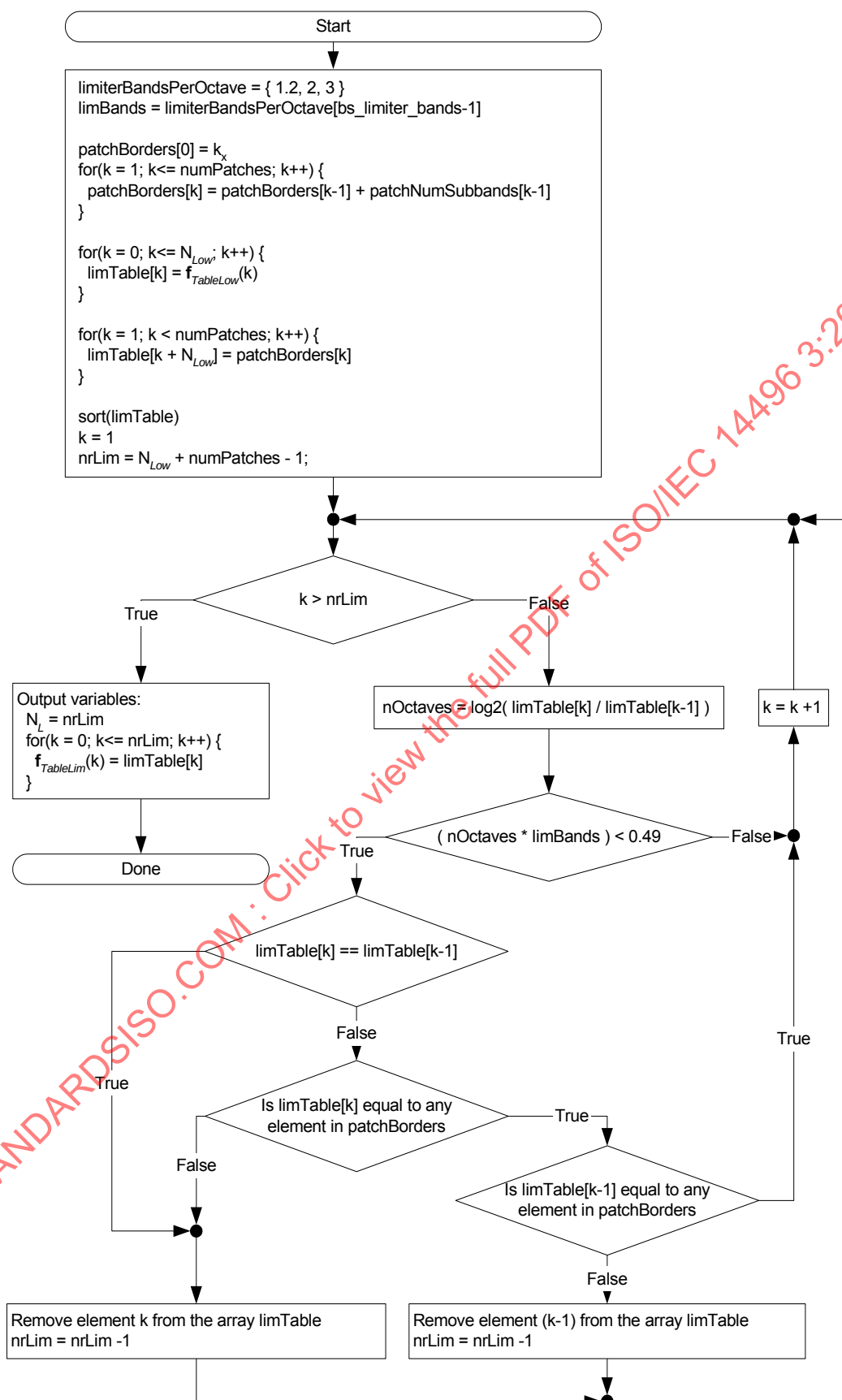
Figure 4.40 – Calculation of f_{\text{TableLim}} if \text{bs\_limiter\_bands} > 0
