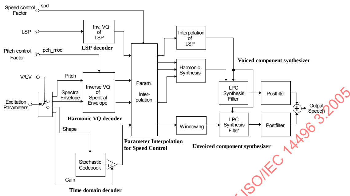
Figure 2.2 — Block diagram of the HVXC decoder
