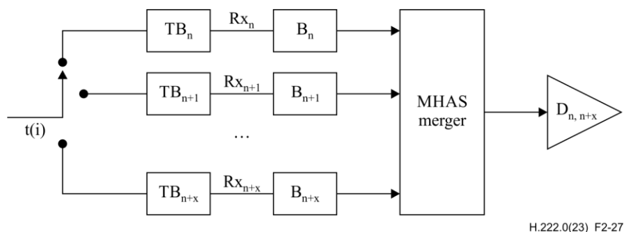
Figure 2-27 – Transport stream system target decoder for multiple audio elementary streams
