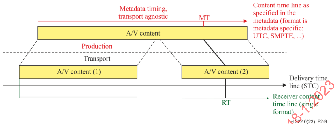
Figure 2-9 – Timing model for delivery of content and metadata
