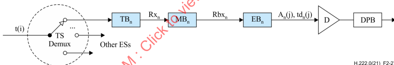
Figure 2-27 – T-STD model extensions for single layer VVC
