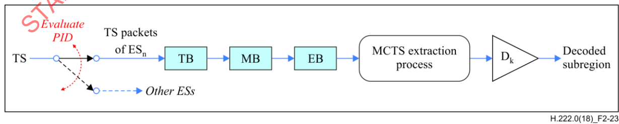
Figure 2-23 – T-STD model extension for transport of HEVC tiles in a common ES ignoring AF descriptors
