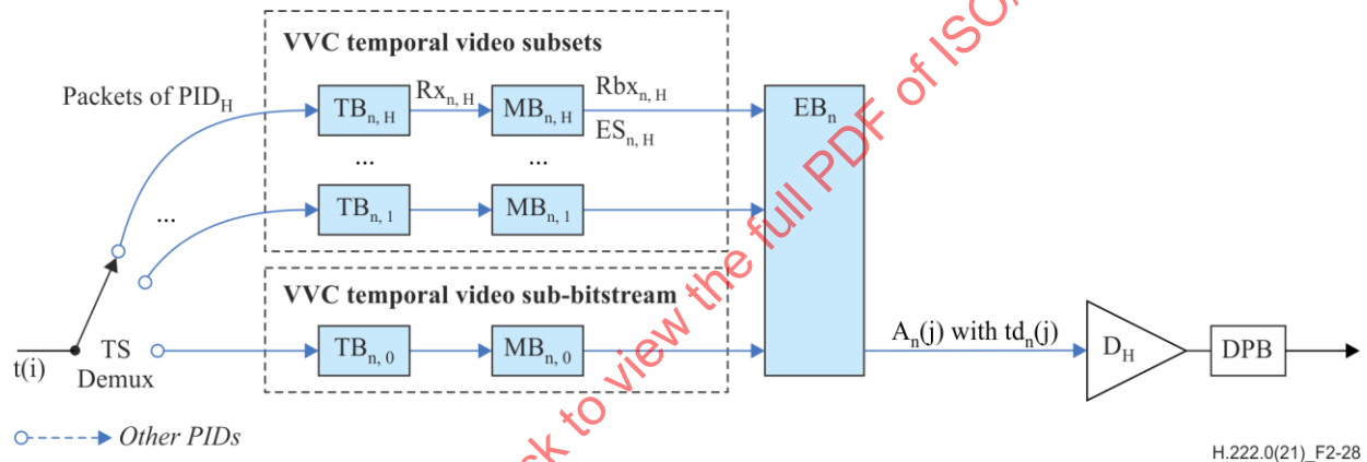
Figure 2-28 – T-STD model extensions for layered transport of VVC temporal video subsets
