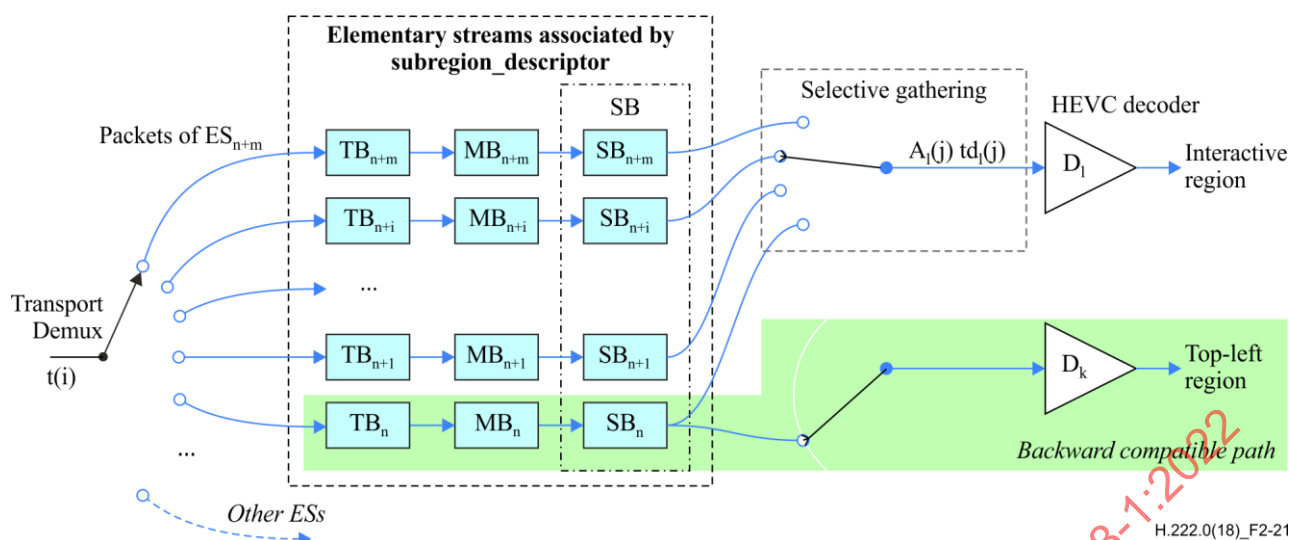
Figure 2-21 – T-STD model extensions for transport of HEVC tiles through individual ESs
