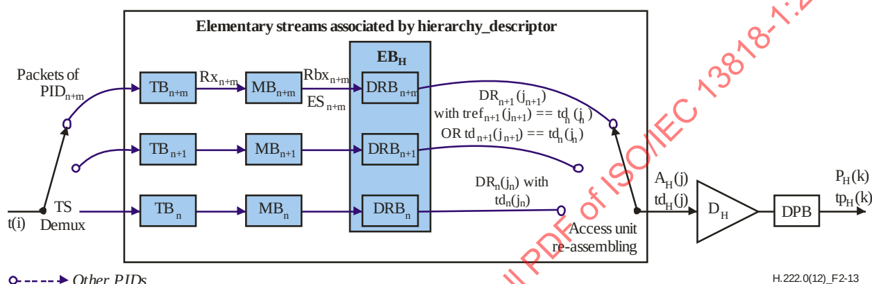
Figure 2-13 – T-STD model extensions for Rec. ITU-T H.264 | ISO/IEC 14496-10 Video with scalable video sub-bitstreams
