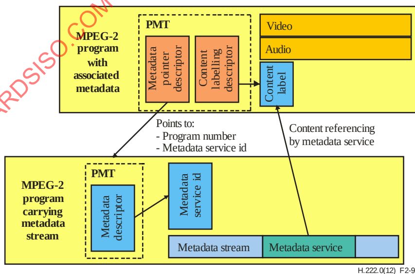
Figure 2-9 – Metadata signalling and referencing
