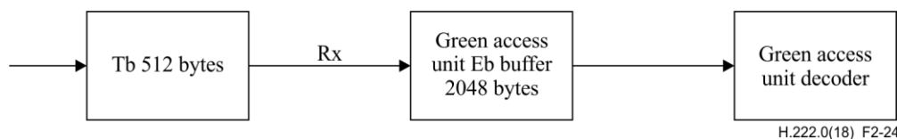
Figure 2-24 – T-STD model extension for green access units
