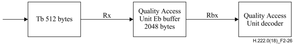
Figure 2-26 – Quality Access Unit decoder processing model
