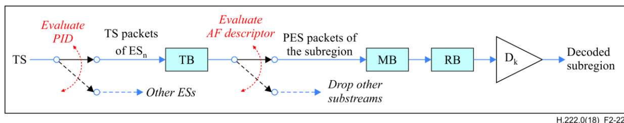
Figure 2-22 – T-STD model extensions for transport of HEVC tiles in a common ES using AF descriptors
