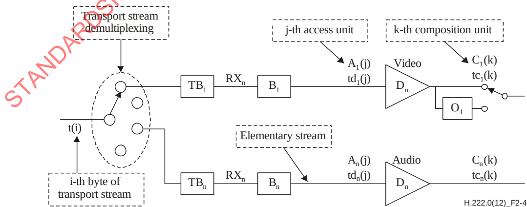
Figure 2-4 – T-STD model extensions for individual ISO/IEC 14496 elementary streams
