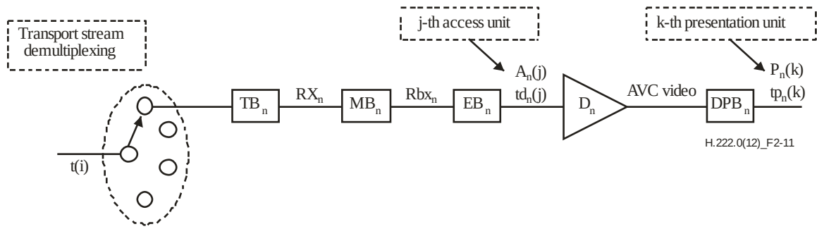
Figure 2-11 – T-STD model extensions for Rec. ITU-T H.264 | ISO/IEC 14496-10 video
