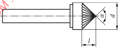
Figure 1 — Hardmetal burr, styles J and K
