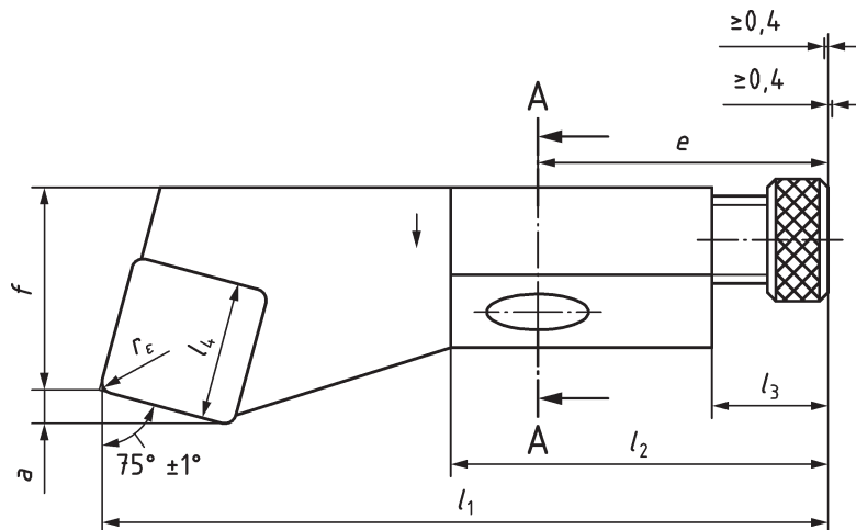
Figure 2 — Style R with height h_1 = 10 mm, 12 mm, 16 mm and 20 mm with square indexable insert
