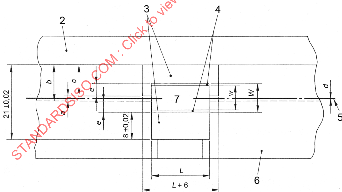
b) Exchange ledges/spacers for the mould in Figure 2
