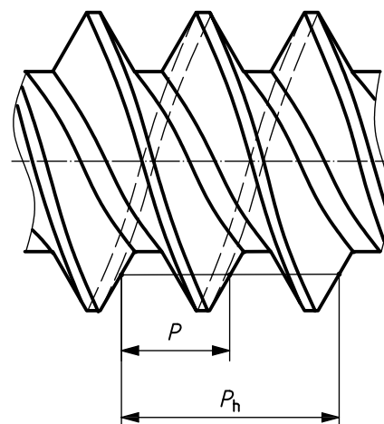
Figure 7 — Two-start right-hand external thread
