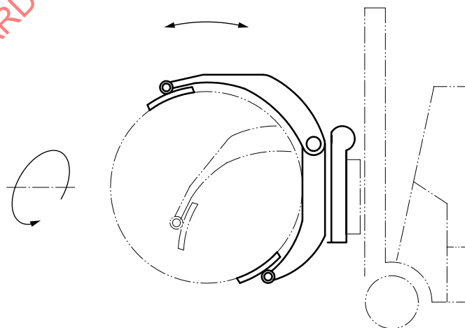
Figure 21 — Rotating roll clamp Figure 21 — Pince à rouleaux rotative
