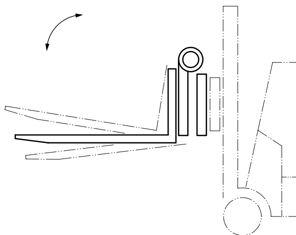
Figure 28 — Tilting carriage Figure 28 — Tablier porte-fourche inclinable
