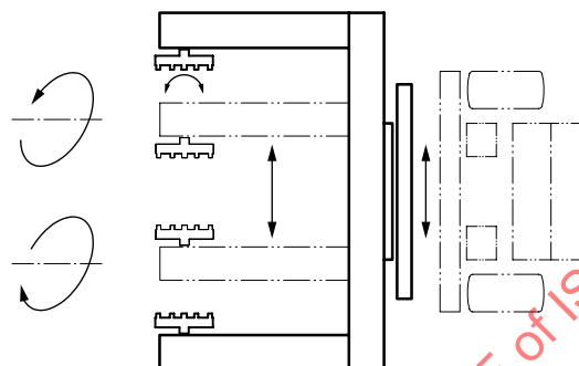
Figure 22 — Tyre manipulator Figure 22 — Manipulateur de pneu
