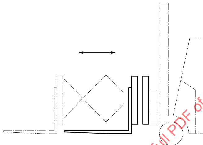
Figure 27 — Reach attachment Figure 27 — Accessoire rétractable
