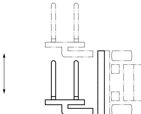
Figure 34 — Side loading attachment Figure 34 — Accessoire à prise latérale
