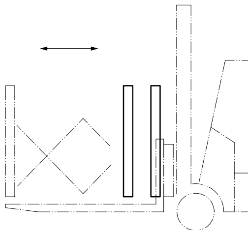
Figure 25 — Push attachment Figure 25 — Pousseur de charge
