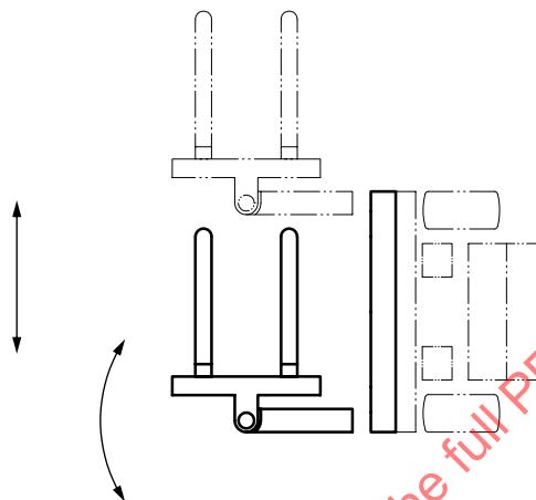
Figure 33 — Three way attachment Figure 33 — Accessoire tri-directionnel
