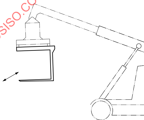
Figure 41 — Container handler fork attachment
