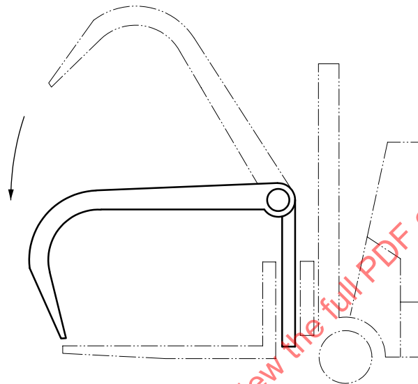
Figure 30 — Log grapple Figure 30 — Pince à grumes
