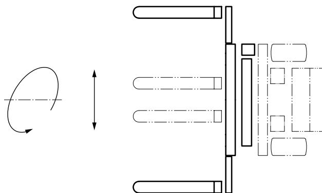
Figure 19 — Rotating fork clamp
