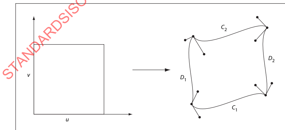
Figure 28 – Coordinate Mapping from a Unit Square to a Four-sided Coons Patch
