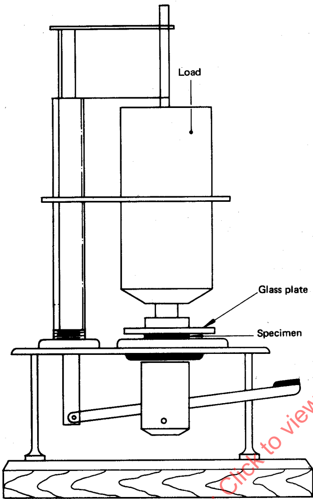
FIGURE 1 — Loading device for use in consistency determination
