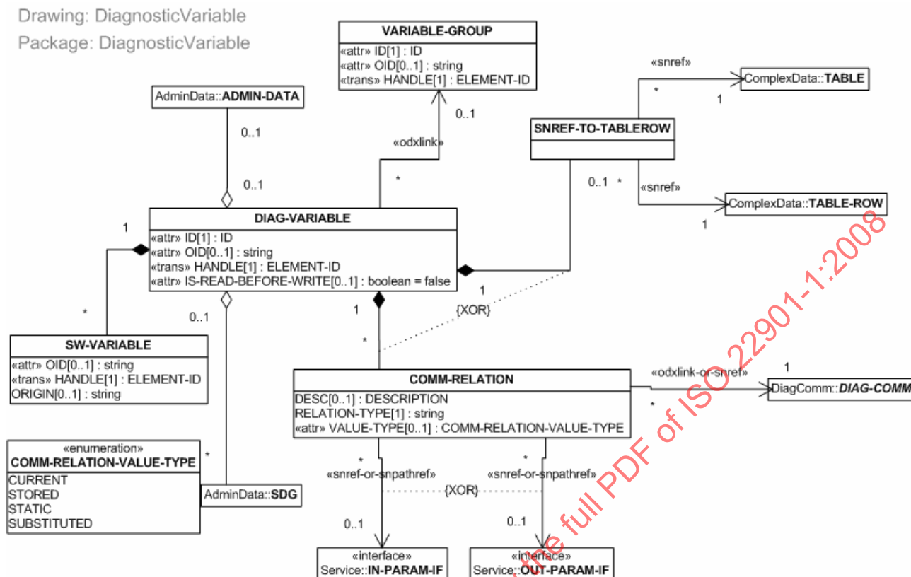
Figure 116 — UML representation of diagnostic variable
