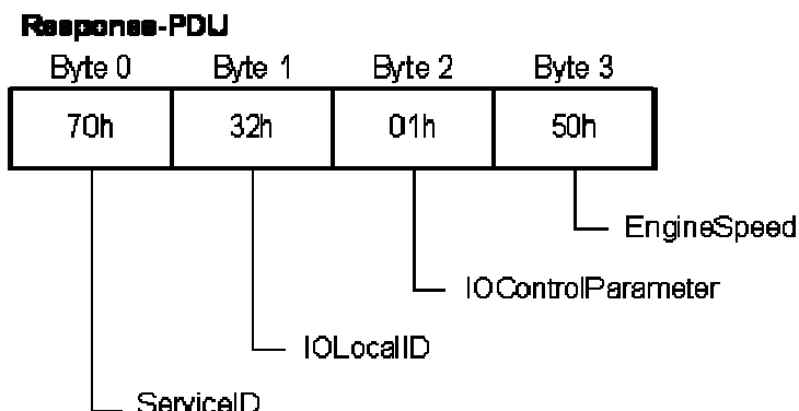
Figure 135 — Response of service 0x30 in ISO 14230
