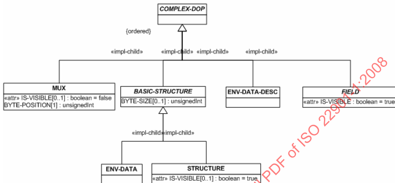
Figure 95 — UML representation of complex data
