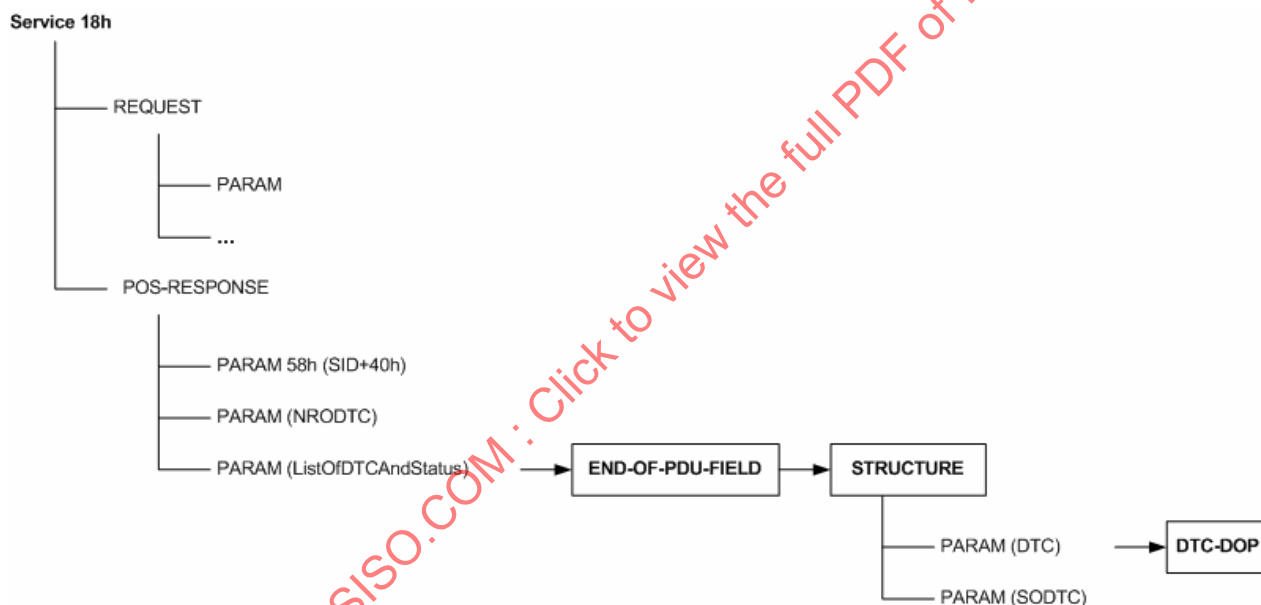
Figure 88 — Structure of service ReadDiagnosticTroubleCodesByStatus (0x18) of ISO 14230-3
