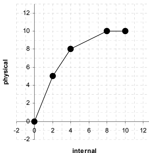
Figure 84 — COMPU-METHOD of type tab interpolated
