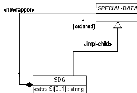
Figure 188 — UML representation of no wrapper element
