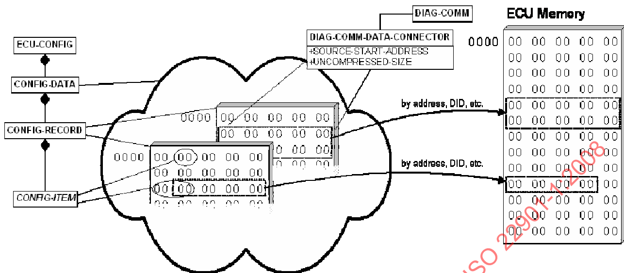
Figure 161 — ECU configuration overview 24)
