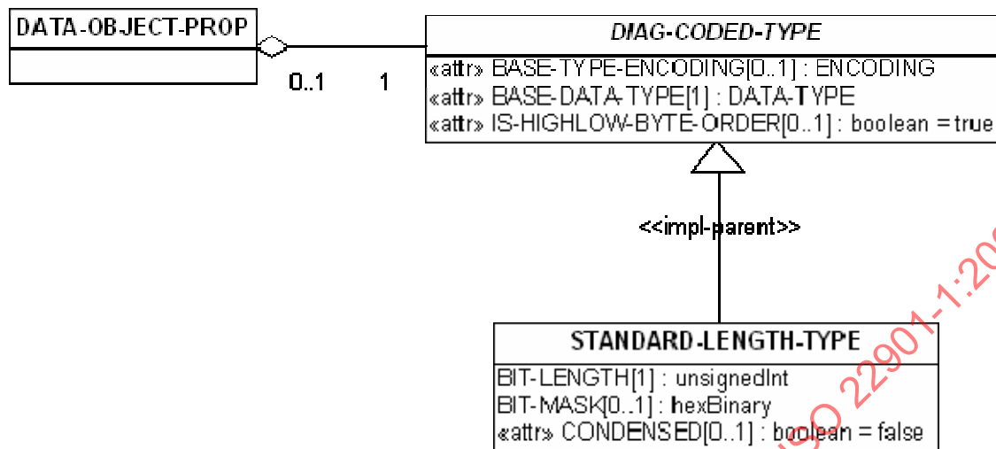
Figure 183 — UML representation of parent generalization
