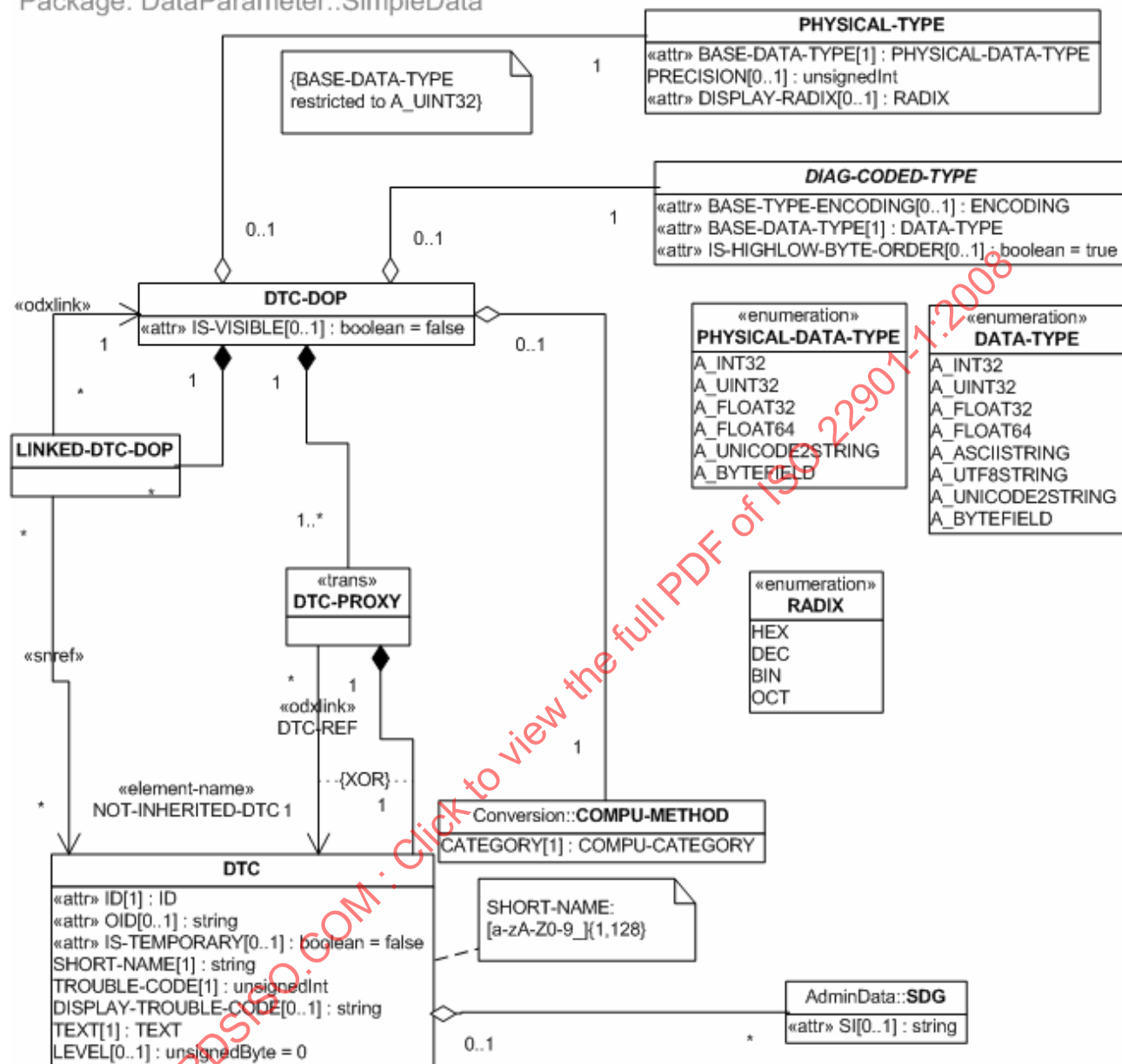
Figure 87 — UML representation of DTC data object property
