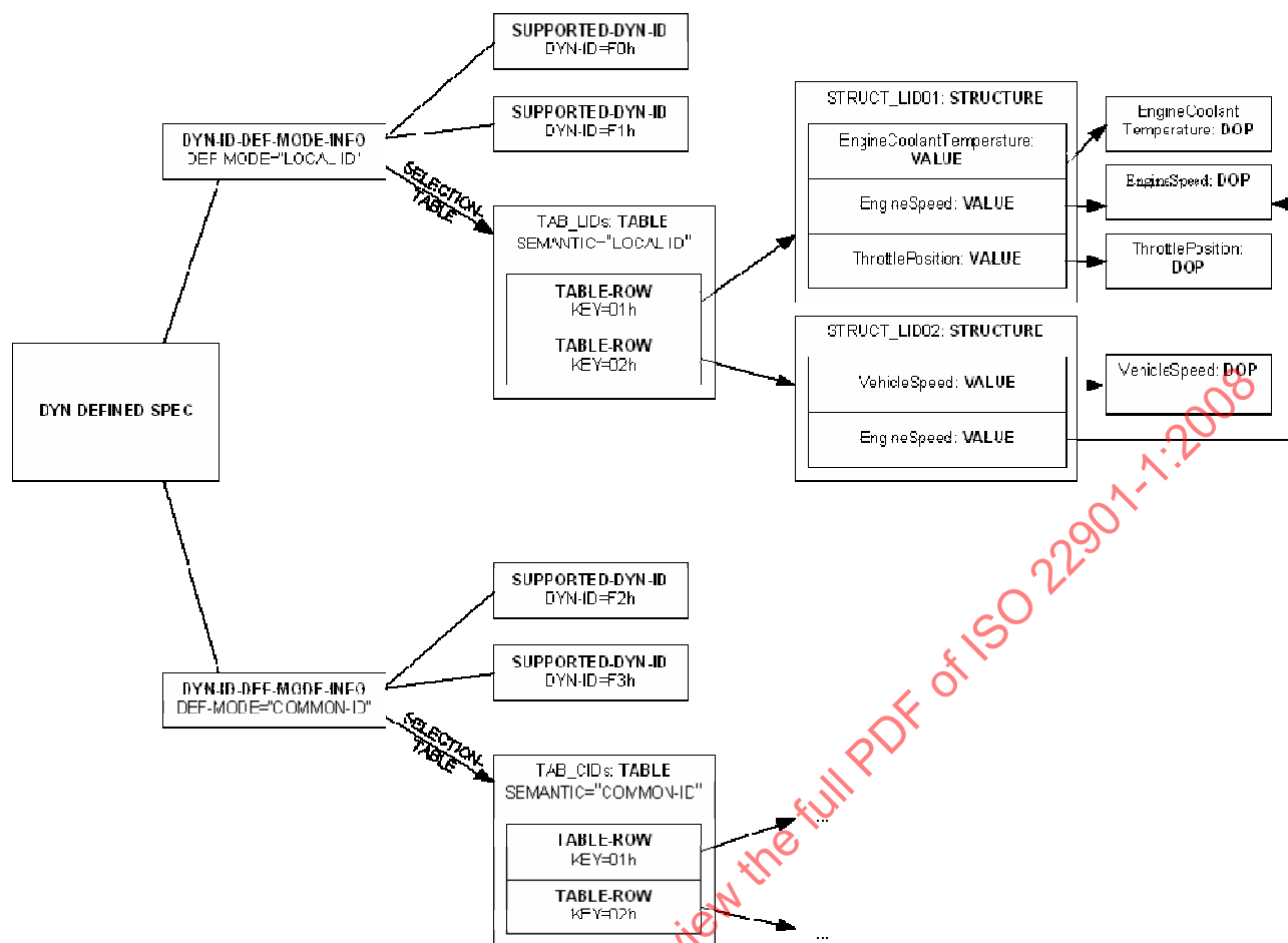
Figure 137 — Example of DYN-DEFINED-SPEC
