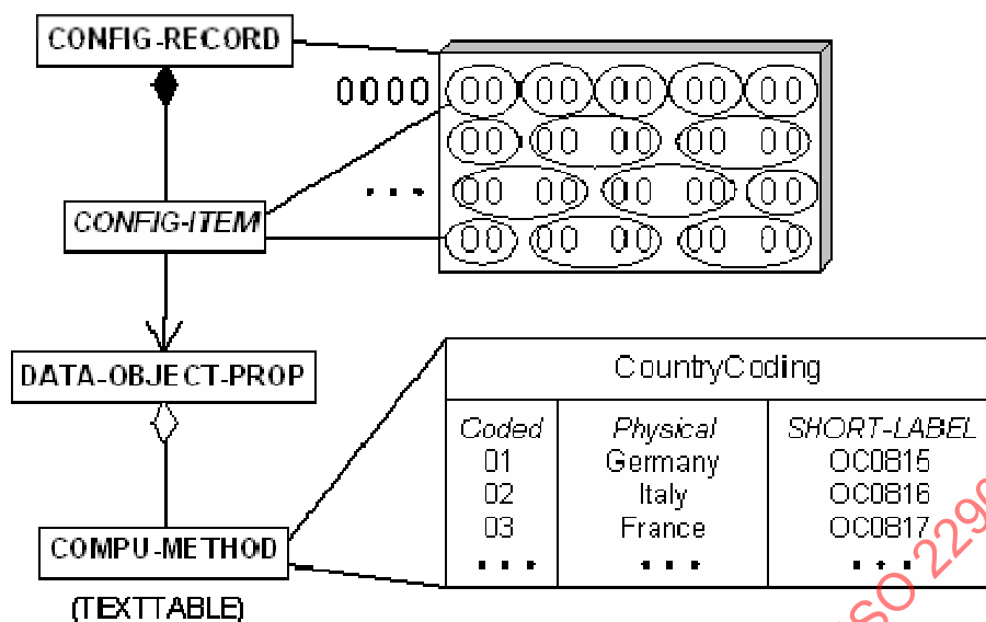
Figure 163 — Using CONFIG-ITEMs illustrates above description.
