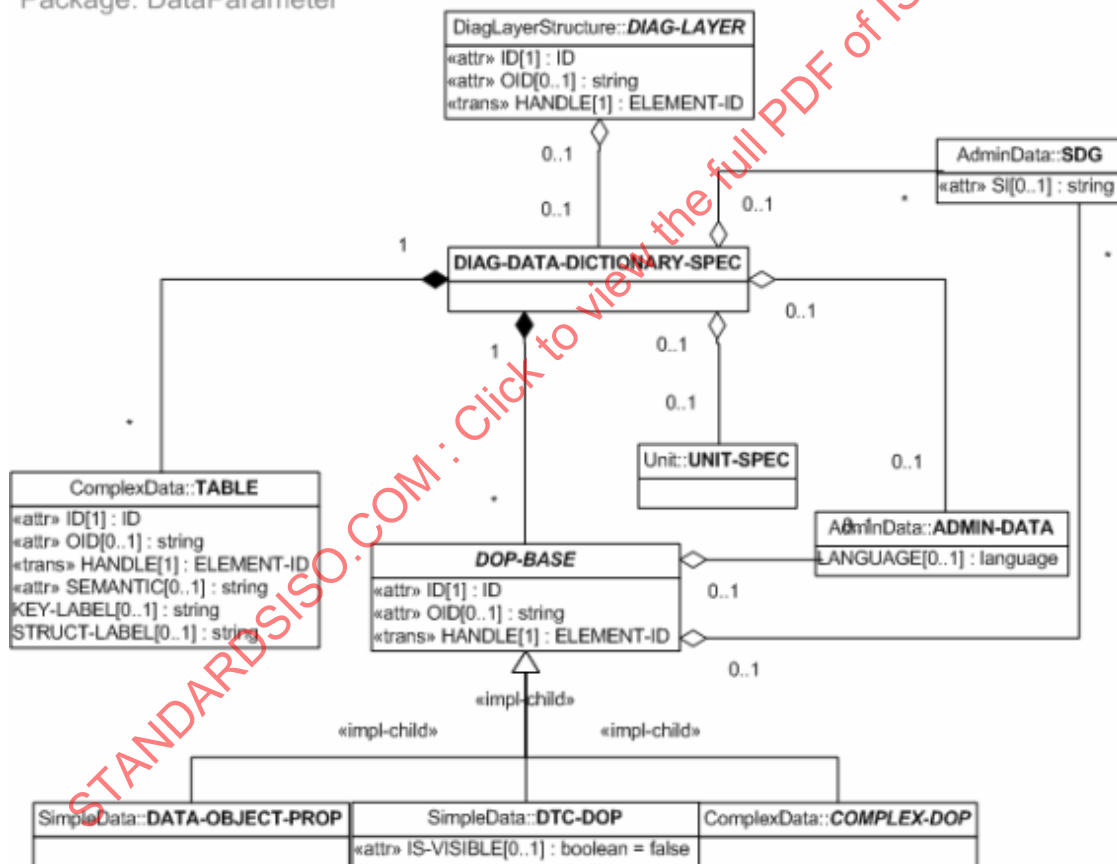
Figure 62 — UML representation of data parameter overview
