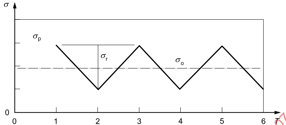
c) Transformed notch stress (effect of elasto-plastic behaviour)
