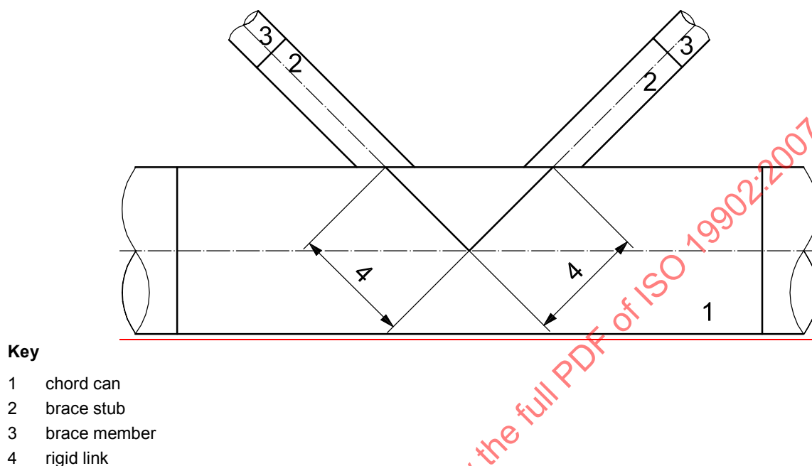
Figure 12.3-2 — Definition of member rigid links
