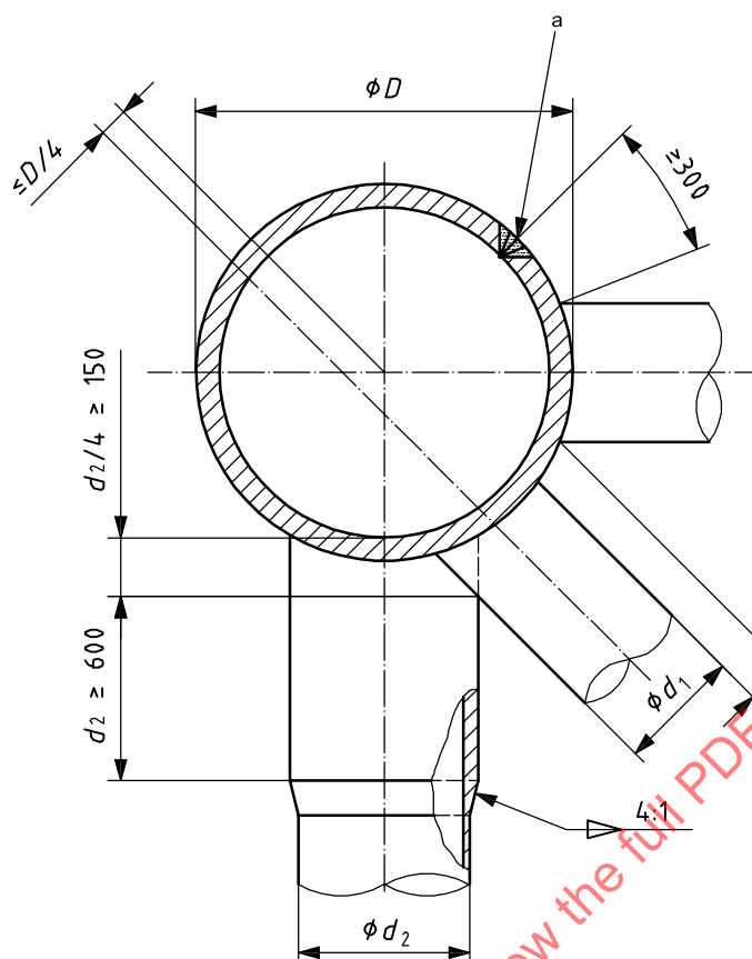
Figure 14.2-4 — Out-of-plane joint detailing
