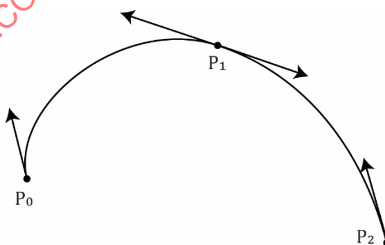
Figure 3 — Hermite Spline
