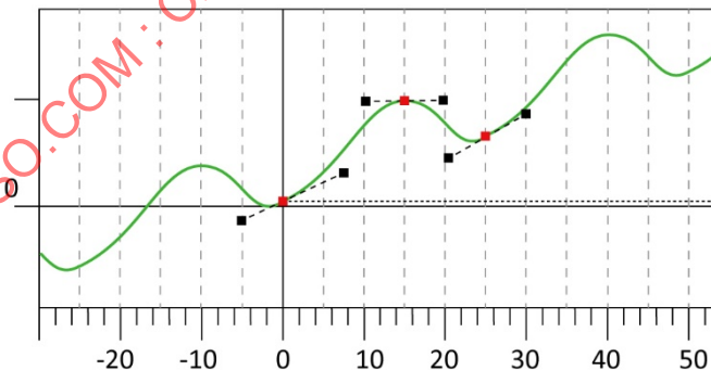
Figure 16 — CYCLE_RELATIVE behaviour
