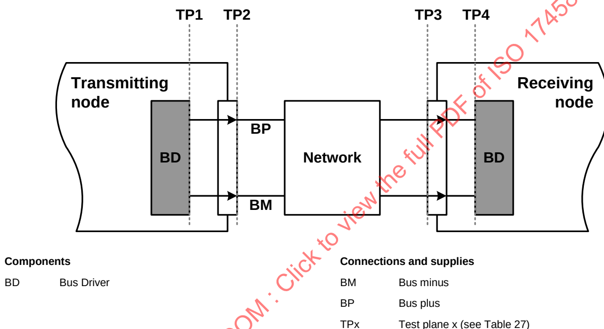
Figure 28 — Planes at the nodes (analog signals)
