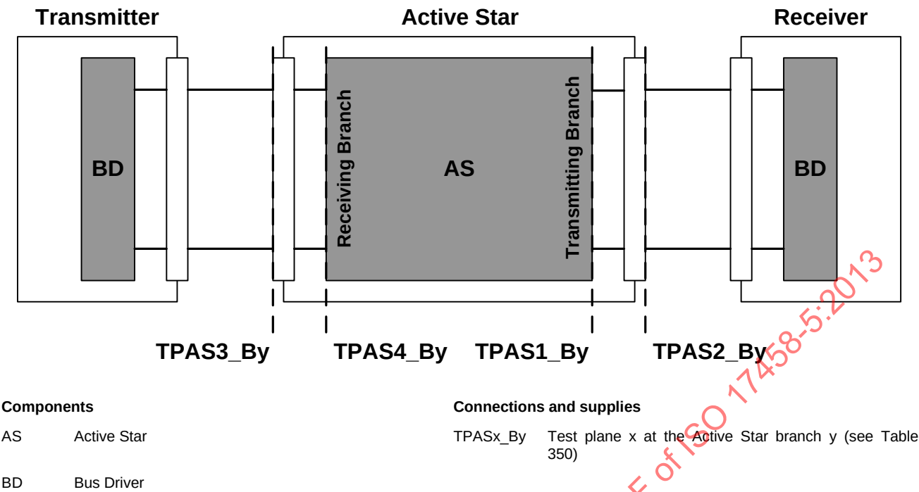
Figure 54 — Test planes at the Active Star for analog signals
