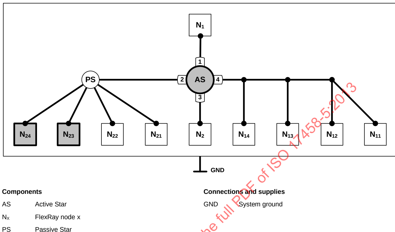
Figure 14 — Location of ground shift
