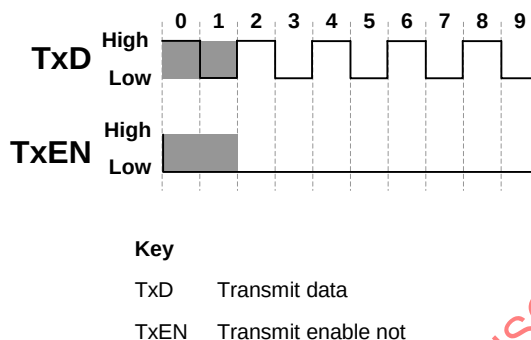
Figure 32 — Test pattern for data signal 50-50
