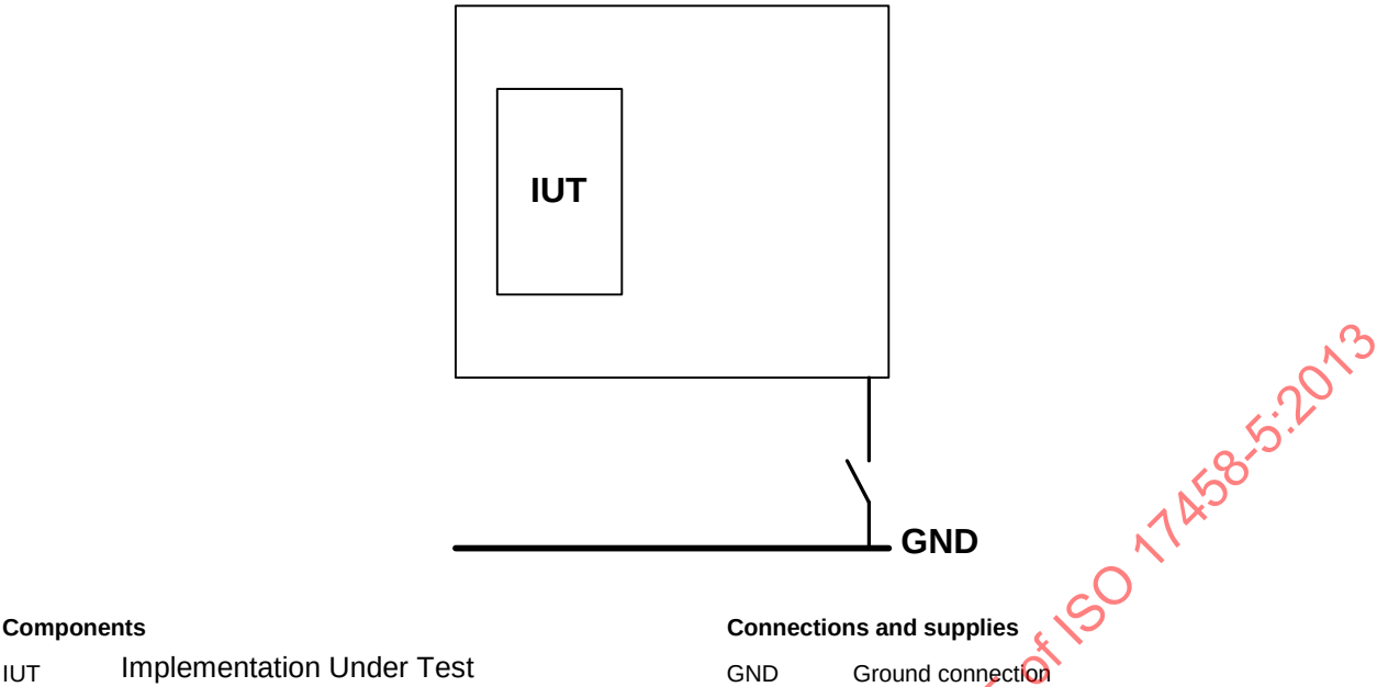
Figure 23 — Failures of bus wires BP and BM (FL19 to FL25)
