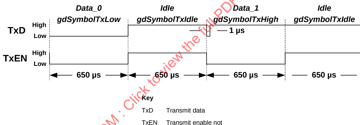
Figure 37 — Pattern for current measurement of bus wires
