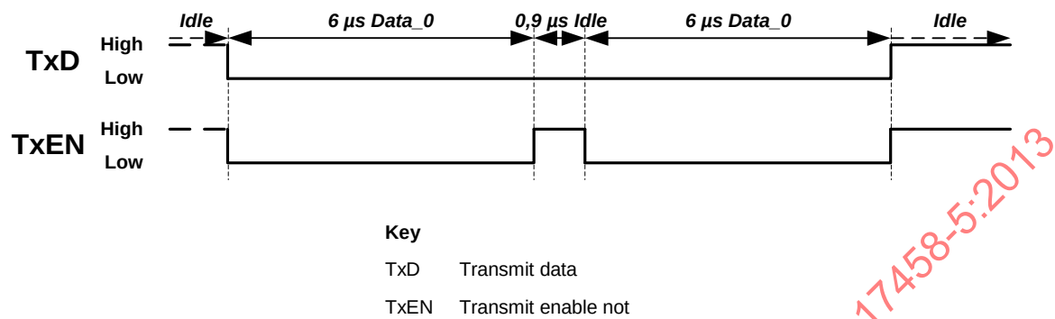
Figure 38 — Test pattern for non suitable wakeup short idle phase
