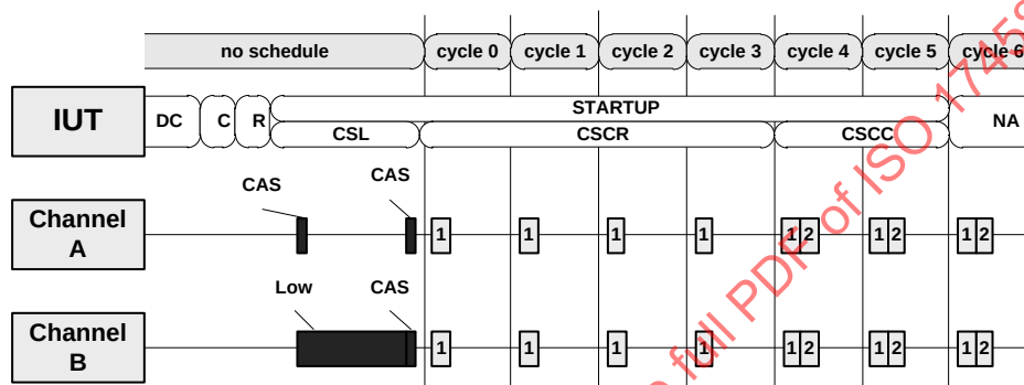
Figure 108 — CAS reception (DC) in POC:coldstart listen – LT's CAS on channel A
