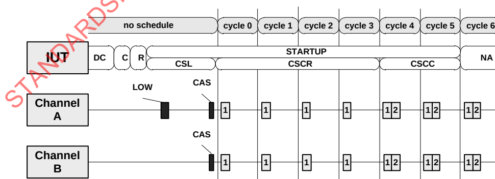
Figure 103 — CE start in POC:coldstart listen – low phase on channel A
