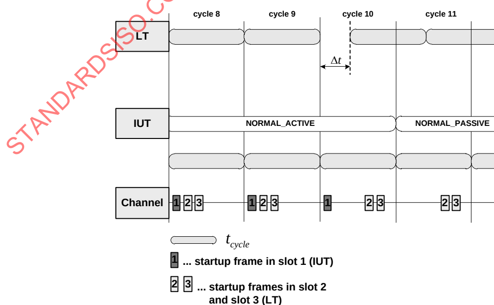
Figure 43 — Deviation outside bounds (halt not allowed); \Delta t greater 0
