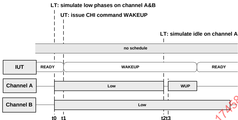
Figure 92 — Wakeup listen and permanent noise on available channel(s) longer than t_{\text{WakeupNoise}} - DC , p_{\text{WakeupChannel}} = A
