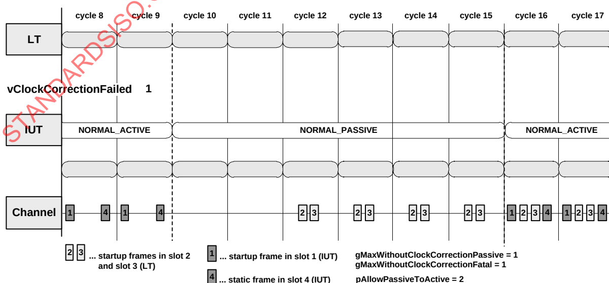
Figure 61 — Additional verification for resynchronization after resumption of sync frame simulation
