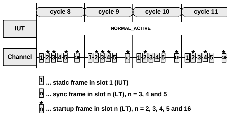
Figure 15 — Startup frame status for integrating node
