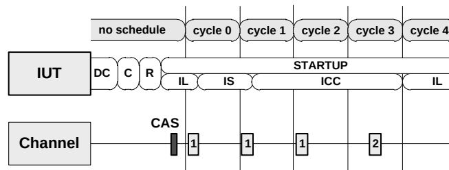
Figure 152 — Startup frame missing in reference slot in POC:integration consistency check
