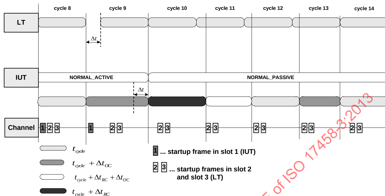
Figure 75 — Resynchronization (transition to POC:normal active not allowed)
