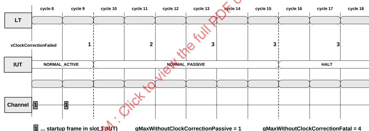
Figure 44 — Missing sync frames (sync node, halt allowed) – gMaxWithoutClockCorrectionPassive = 1 , gMaxWithoutClockCorrectionFatal = 4
