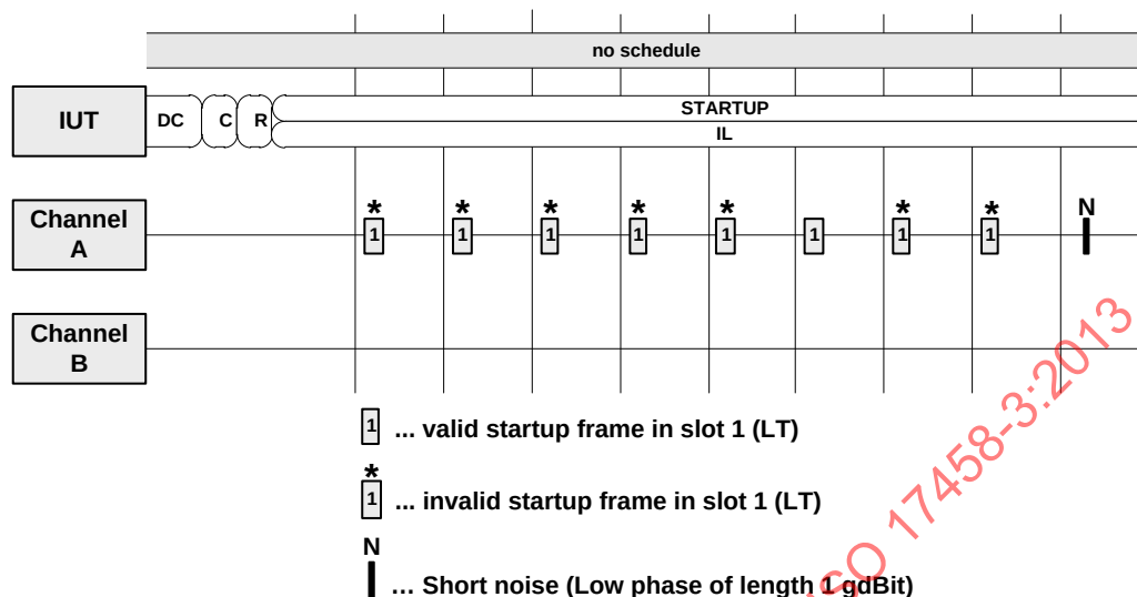
Figure 130 — Invalid startup frame reception in POC:integration listen – invalid startup frames on channel A
