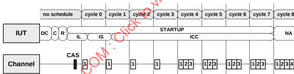
Figure 150 — Integration into starting cluster in POC:integration consistency check
