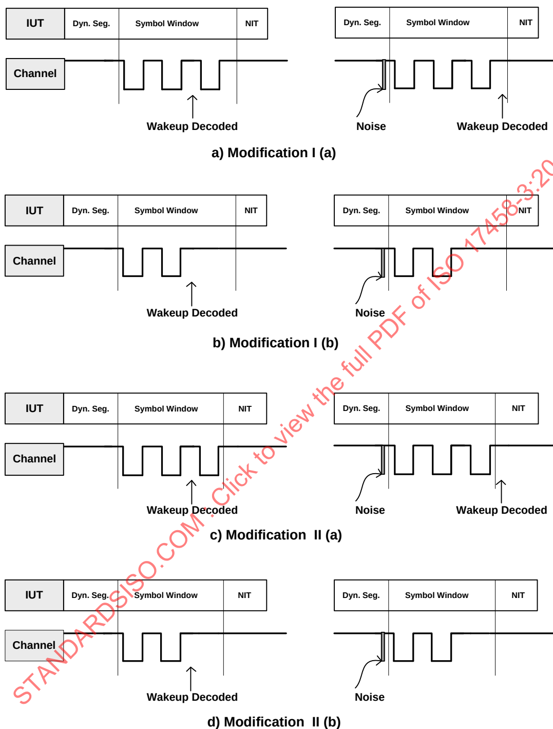
Figure 19 — WUDOP reception – different scenarios of WUDOP reception with and without noise
