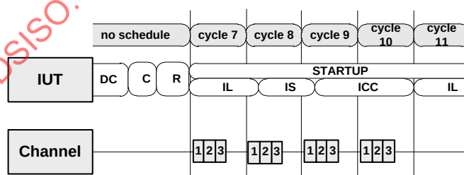
Figure 148 — Sync frames in POC:integration consistency check
