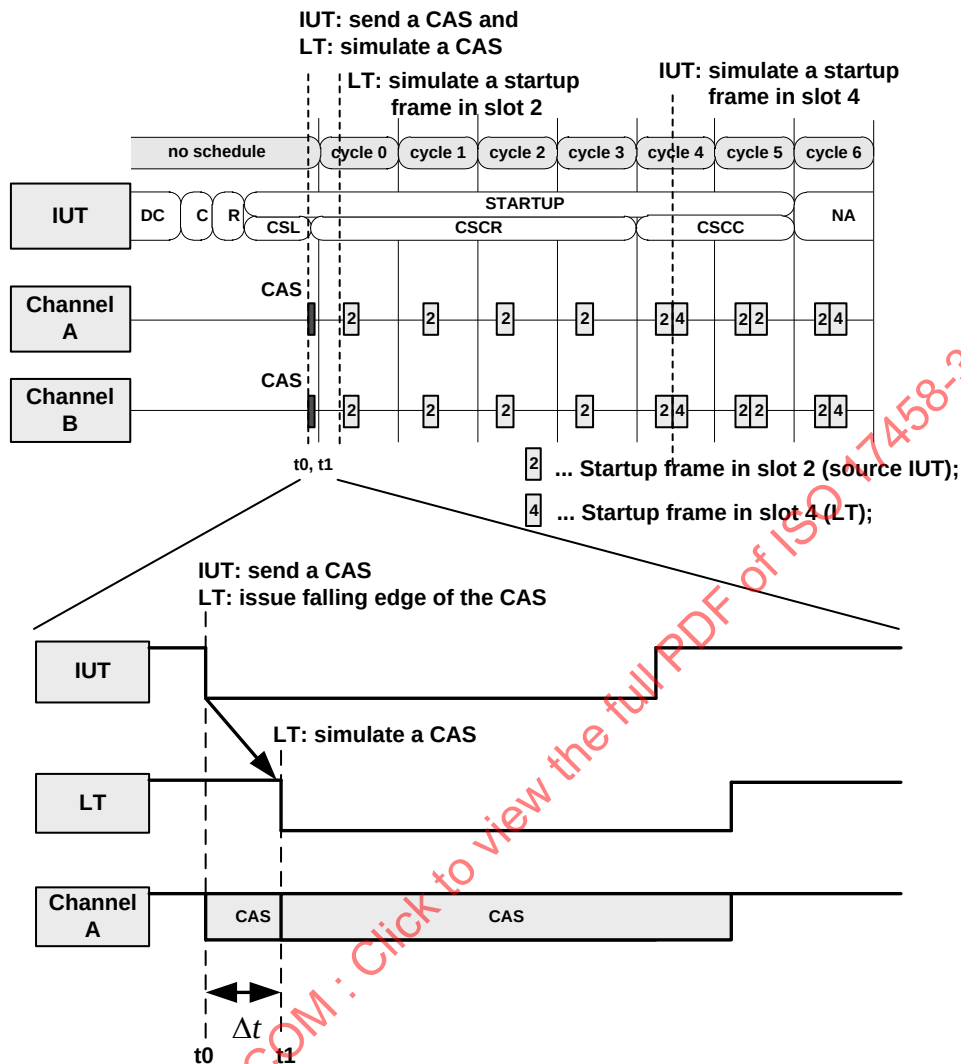
Figure 116 – Parallel startup (CAS collision) IUT as leading coldstarter – \Delta t = (2 \pm 2) * \text{gdBit} / \text{pdMicrotick } \mu\text{T}
