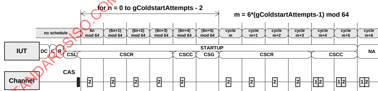
Figure 118 — Channel idle until last coldstart attempt in POC:coldstart consistency check
