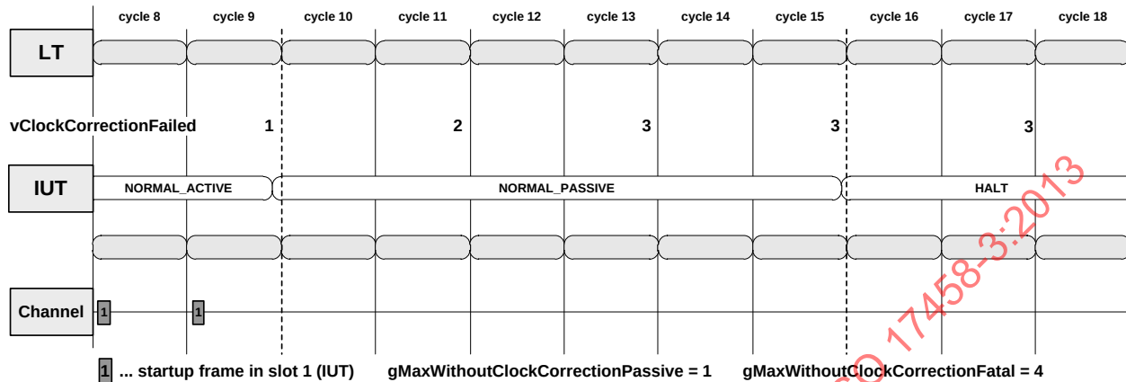
Figure 51 — Missing sync frames (sync node, halt allowed, even cycle)
