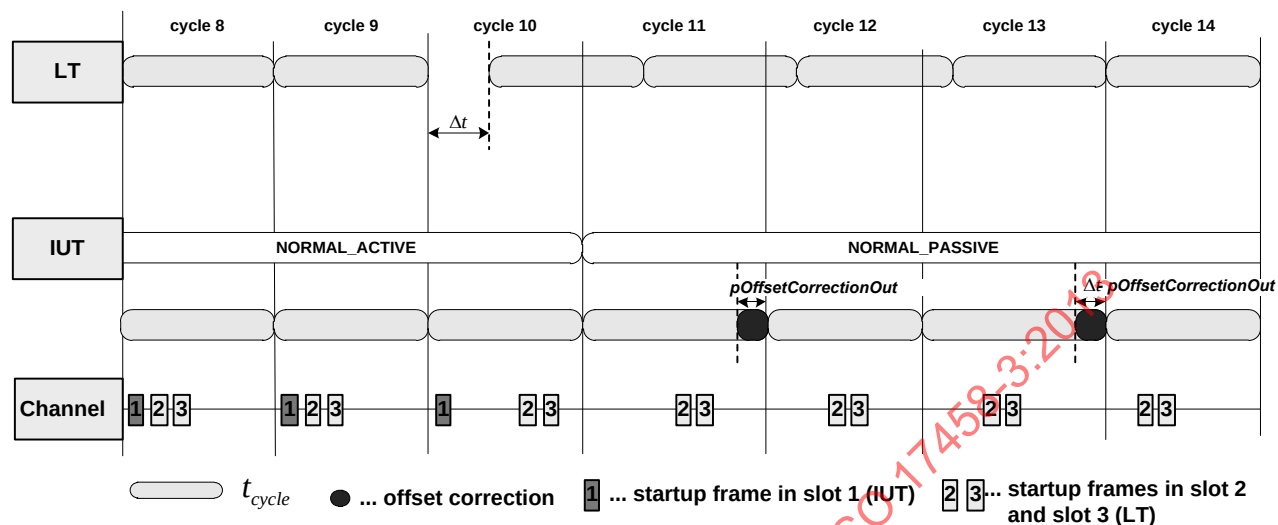
Figure 56 — Resynchronization (transition to POC:normal active not allowed ) – pAllowPassiveToActive = 0
