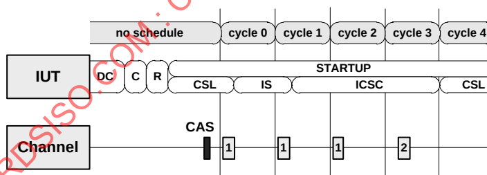
Figure 139 — Startup frame missing in reference slot in POC:integration coldstart check
