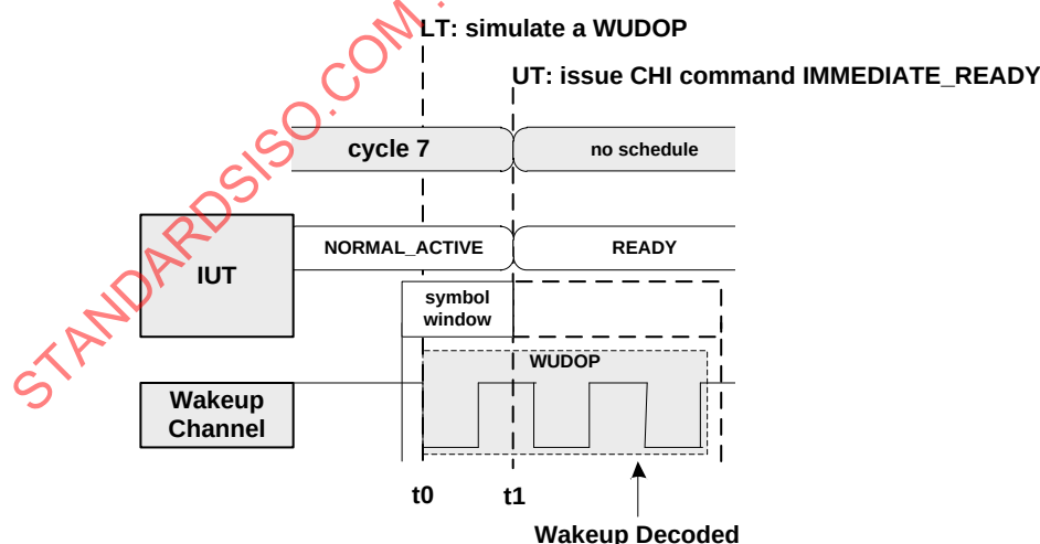
Figure 32 — Command IMMEDIATE_READY and received WUDOP – command issued in POC:normal active
