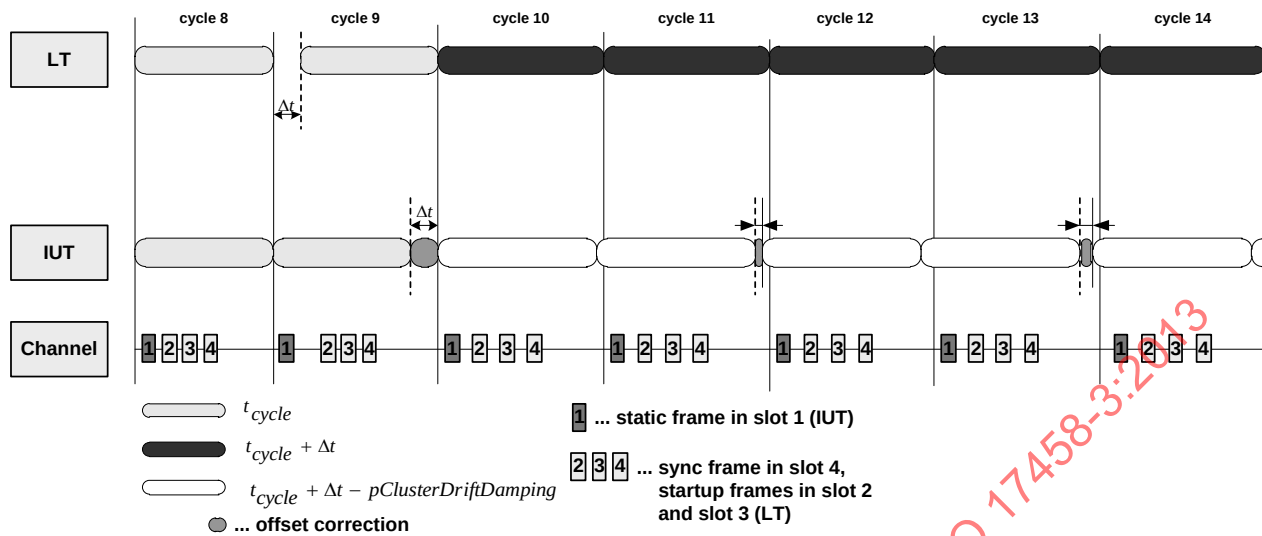
Figure 65 — Cluster drift damping; \Delta t > 0
