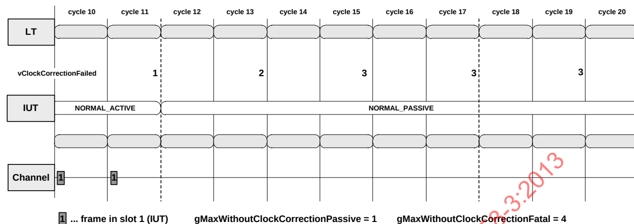
Figure 47 — Missing sync frames (no sync node, halt not allowed)
