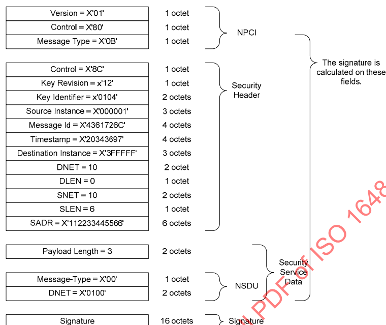
Figure 24-2. An example secured NPDU (Who-Is-Router-To-Network). Securing BVLL Messages
