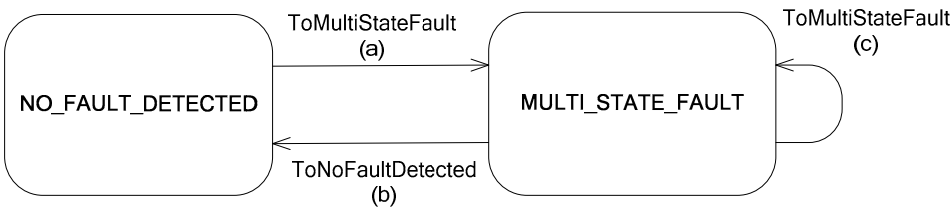
Figure 13-30. Transitions indicated by FAULT_STATE algorithm
