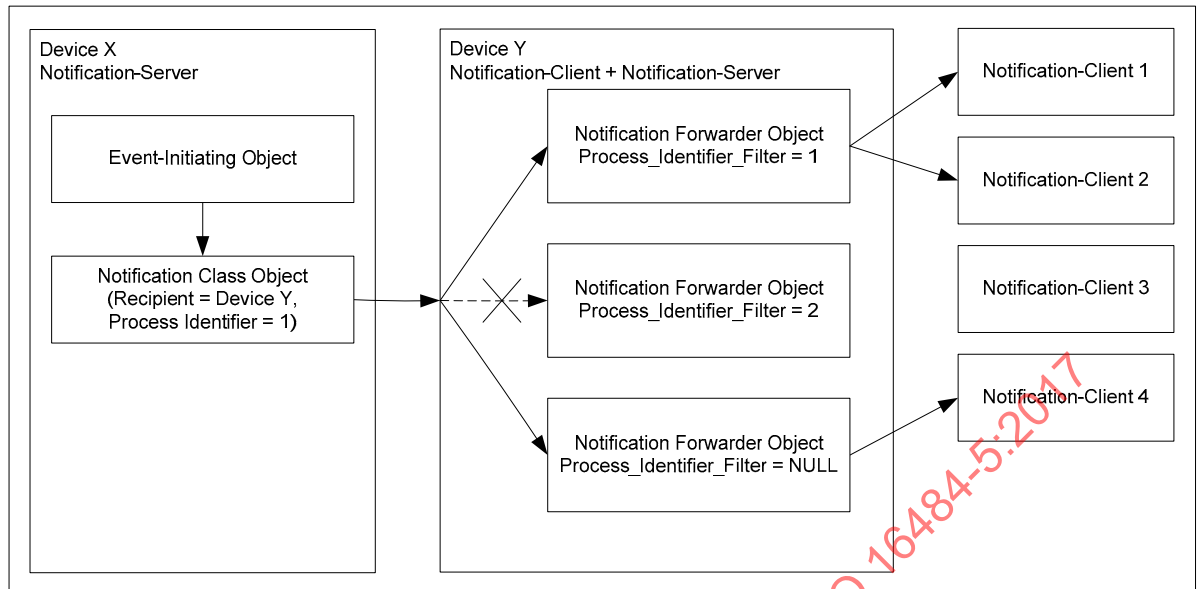
Figure 12-8. Example of Forwarding a Single-Event Notification.
