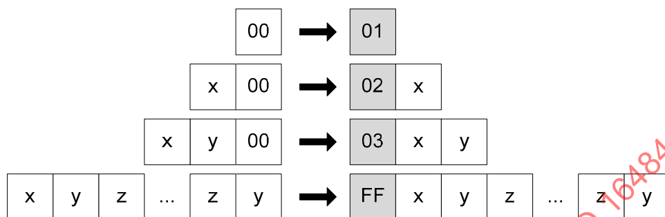
Figure 9-6. COBS Encoding of Chunks into Code Blocks
