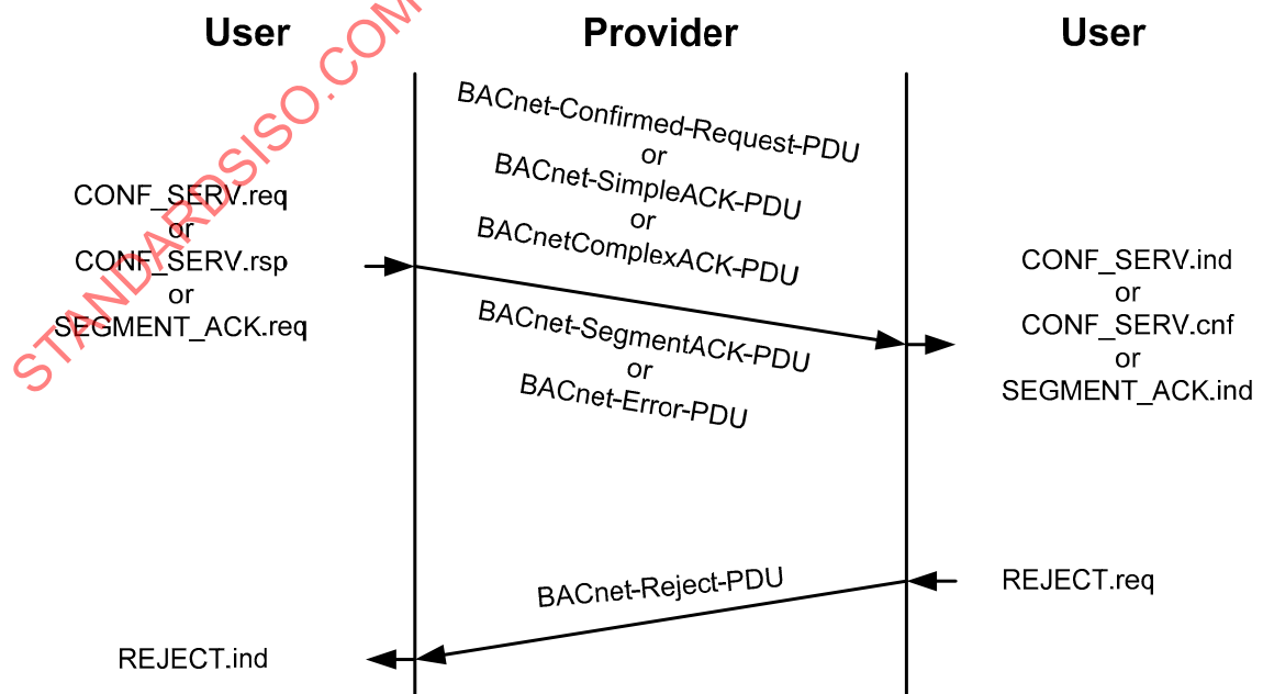
Figure 5-13. Time sequence diagram for an abnormal service request or response with a protocol error.
