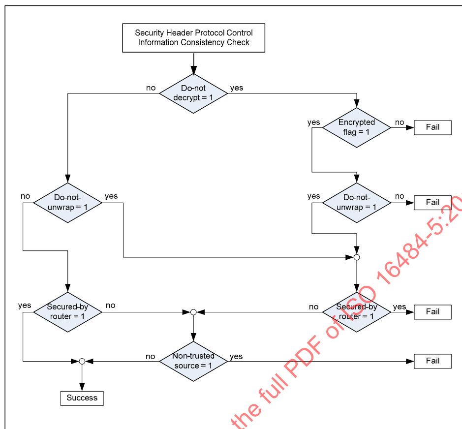
Figure 24-8: Security Header Protocol Control Information Consistency Check
