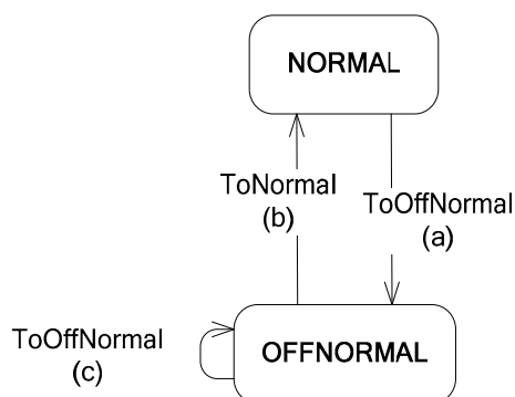
Figure 13-24. Transitions indicated by CHANGE_OF_CHARACTERSTRING algorithm
