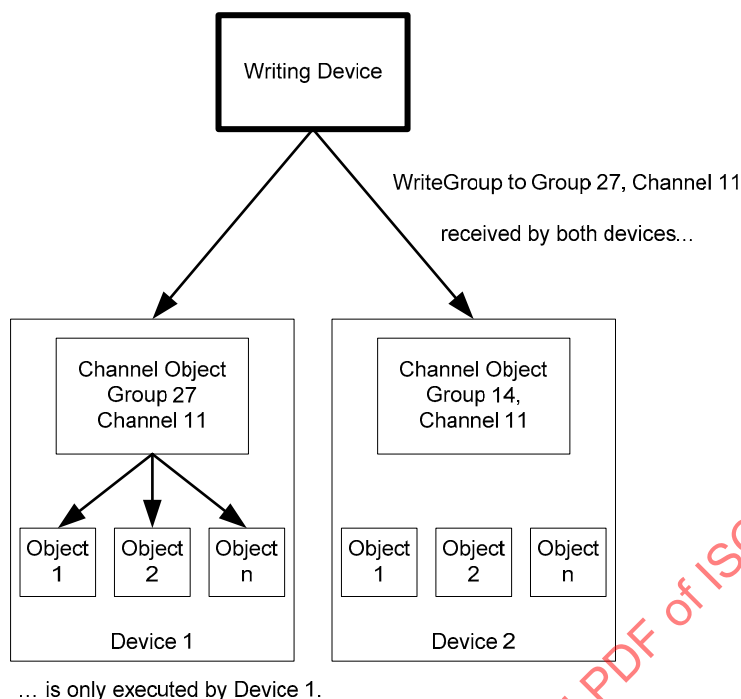
Figure 12-11. Control Groups Limit WriteGroup Effect to Specific Channel Objects Across Many Devices
