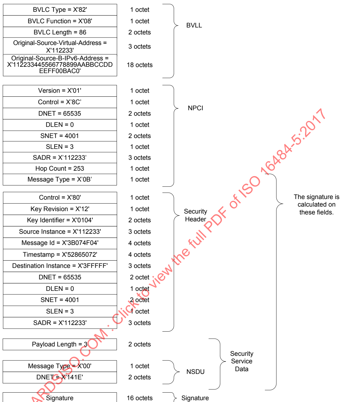
Figure 24-6. An example B/IPv6 BVLL containing a Secured NPDU (Who-Is-Router-To-Network).
