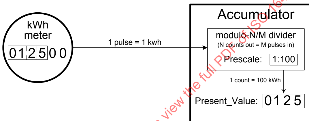
Figure 12-25. Example of an Accumulator object
