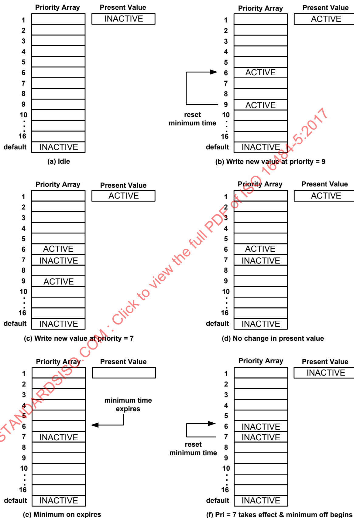
Figure I-1. Example of minimum on and off times.
