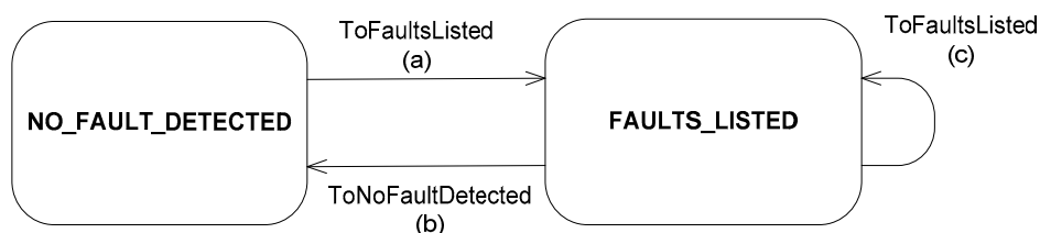
Figure 13-33. Transitions indicated by the FAULT_LISTED algorithm
