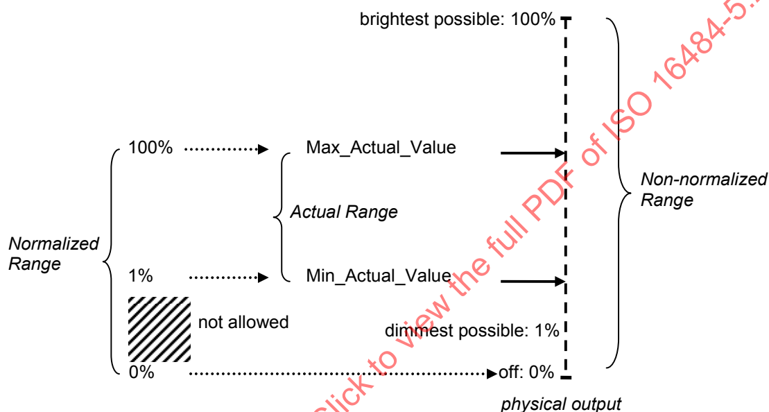
Figure 12-13. Normalized Range of the Lighting Output
