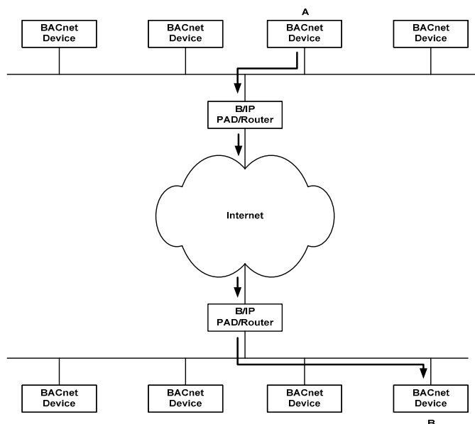
Figure H-2. IP tunneling implemented with a B/IP PAD router.
