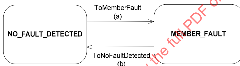
Figure 13-31. Transitions indicated by FAULT_STATUS_FLAGS algorithm
