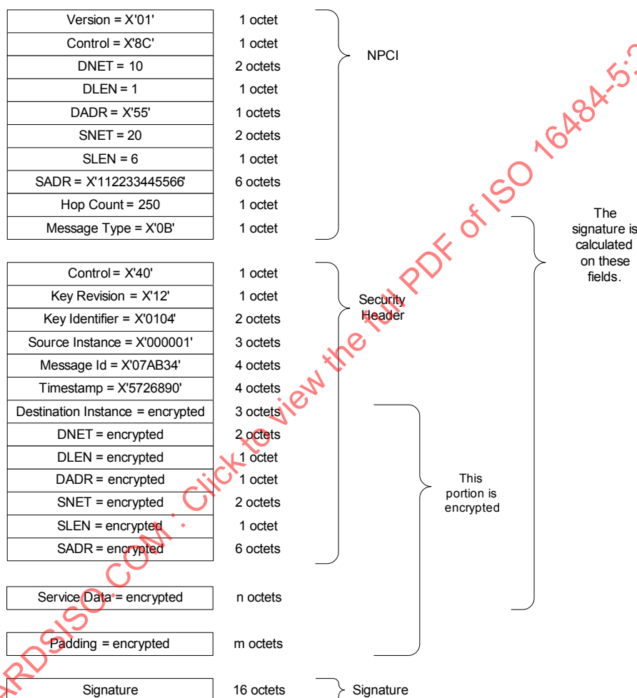
Figure 24-7. An example encrypted message.
