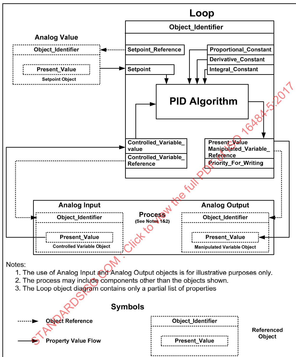
Figure 12-2. Loop Object Structure with its Referenced Objects.
