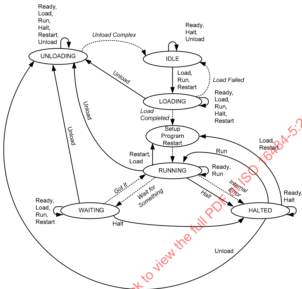
Figure 12-3. State Transitions for the program object.
