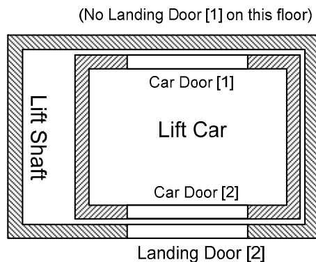
Figure 12-23. Example Two Door Lift Car
