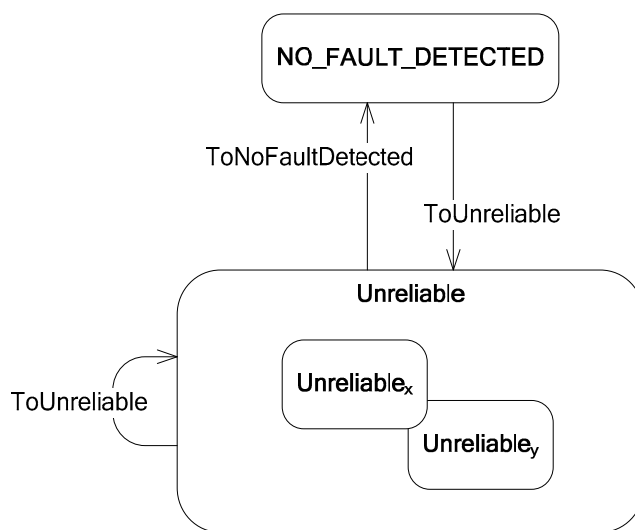
Figure 13-28. Transitions indicated by FAULT_EXTENDED algorithm
