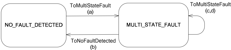
Figure 13-29. Transitions indicated by FAULT_LIFE_SAFETY algorithm
