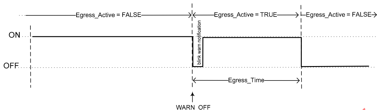
Figure 12-17. Blink-warn and Egress Time
