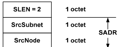
Figure 6-3. Encoding of the SLEN and SADR for NPDU's originating from LonTalk devices being routed through BACnet.
