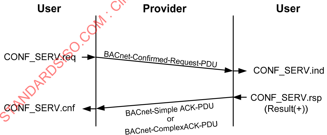
Figure 5-6. Time sequence diagram for normal confirmed services.
