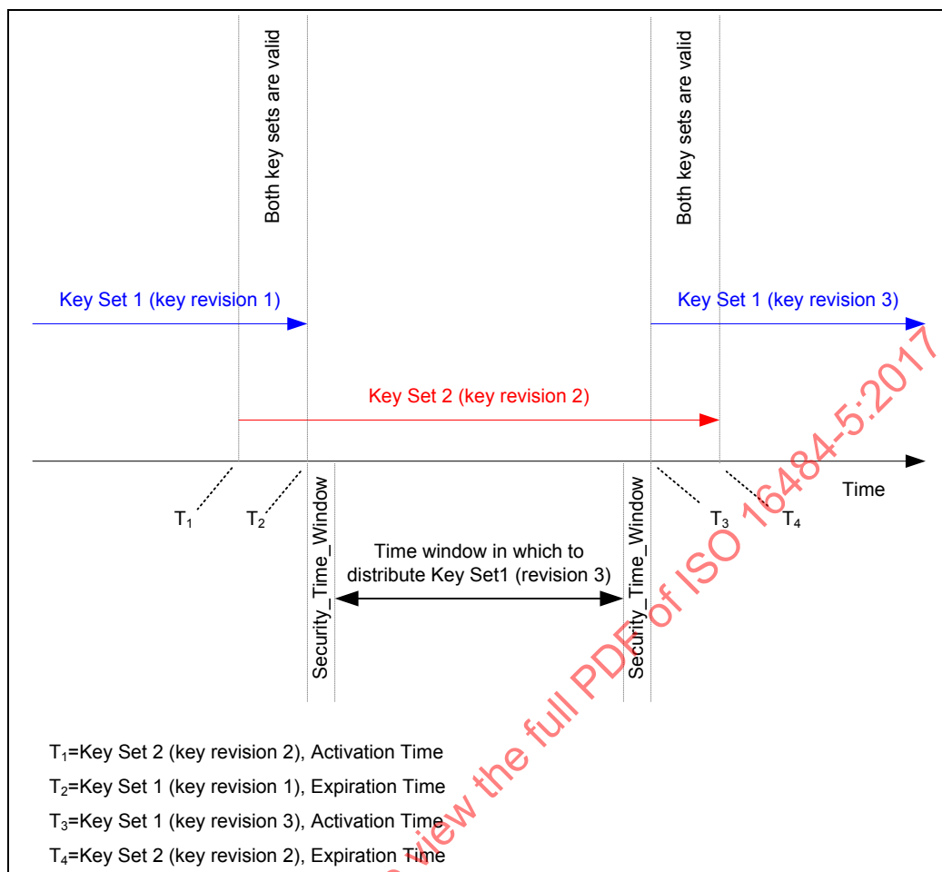
Figure 24-9: Key Set lifetimes.
