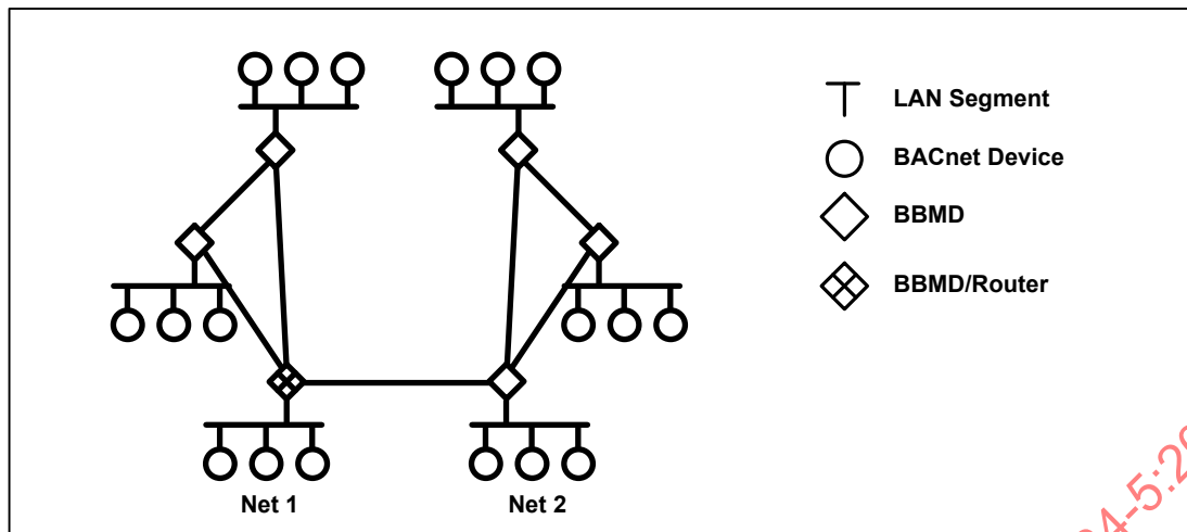
Figure J-6. An alternative to the architecture depicted in Figure J-5 is to combine both BBMD and router functionality in the same physical device as explicitly permitted in Clause J.7.1.
