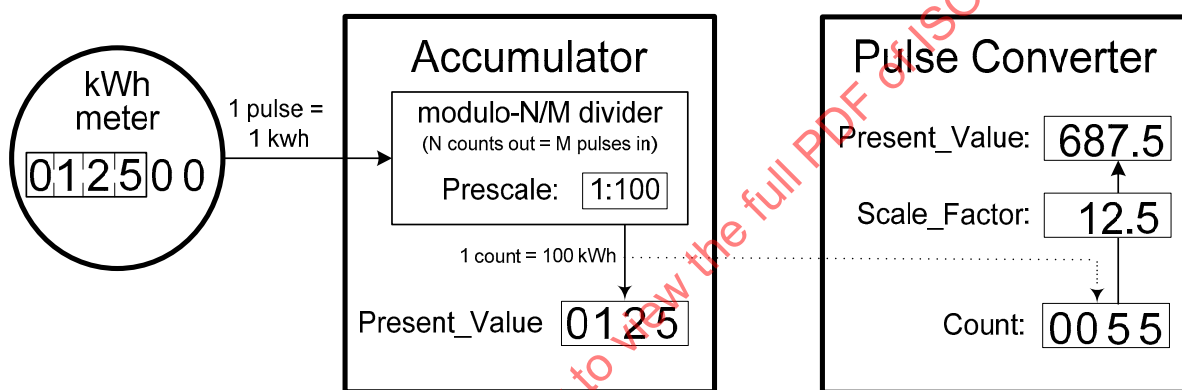
Figure 12-4. Relationship between the Pulse Converter and Accumulator objects.
