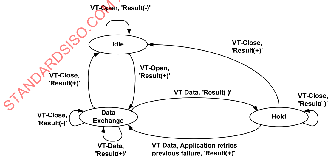
Figure 17-4. Virtual terminal services state diagram.
