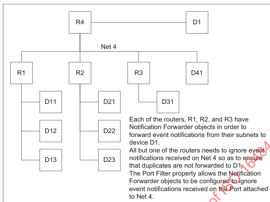
Figure 12-6. General Use Case for the Port Filter property.
