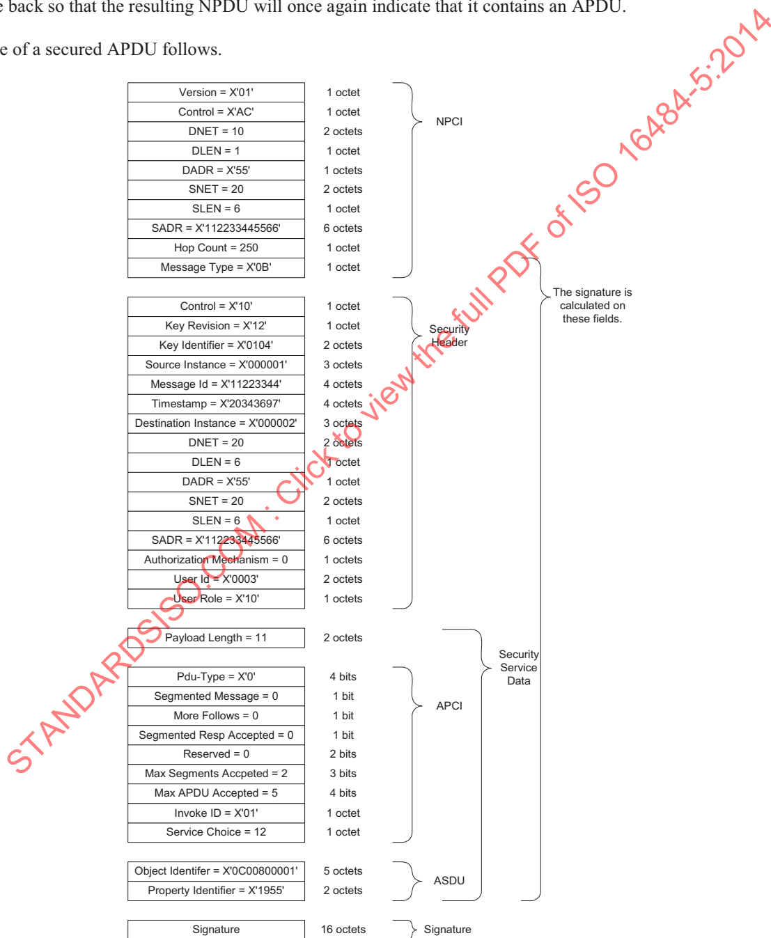
Figure 24-1. An example secured APDU (Read-Property).
