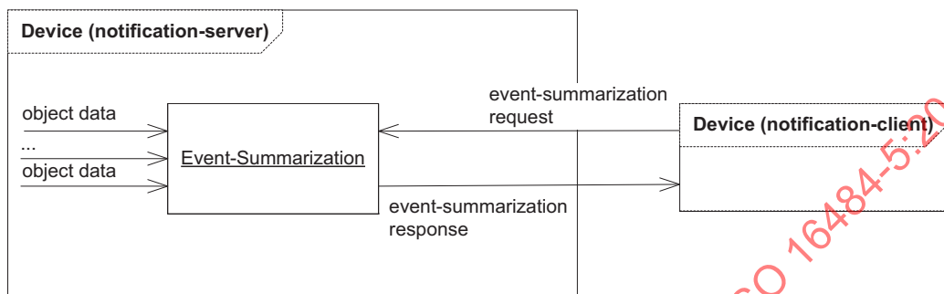
Figure 13-6. Event-Summarization
