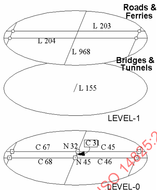
Figure 209 — Structure as a Line Feature
