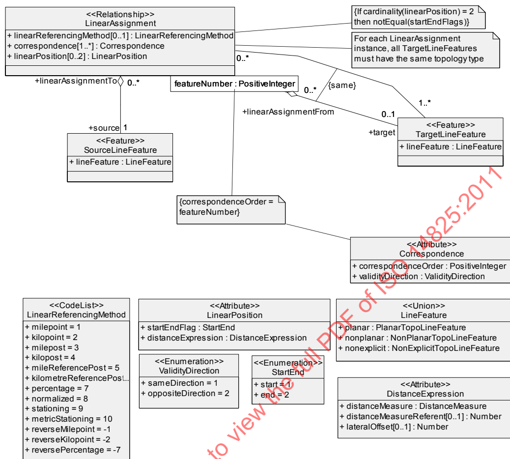
Figure 173 —The Conceptual Data Model for the Linear Assignment Relationship
