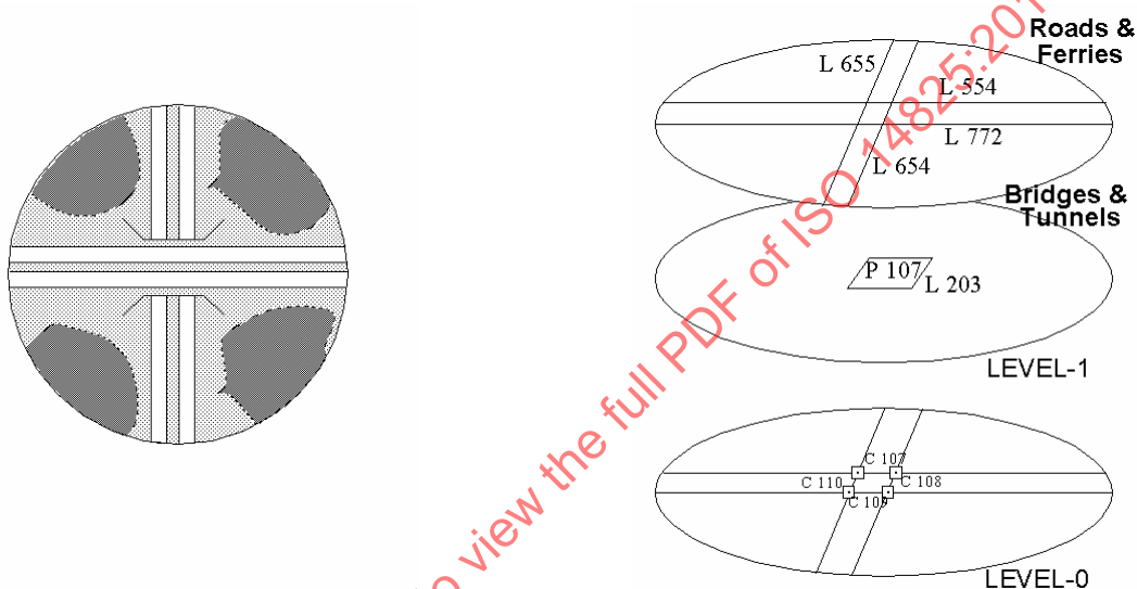
Figure 212 — A structure at the crossing of 2 dual carriageways
