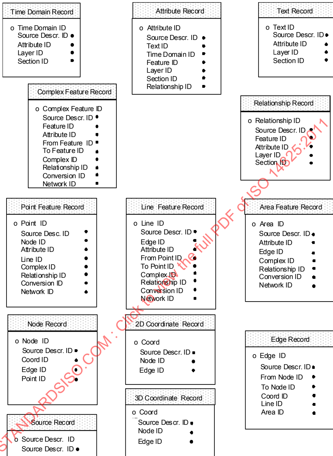
Figure 222 — Pointer fields and their role in the records (connectivity rendering of non-planar topology)
