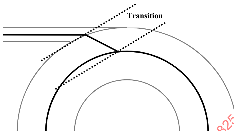
Figure 142 – Schematic example of road centreline transition at a curve/roundabout circle
