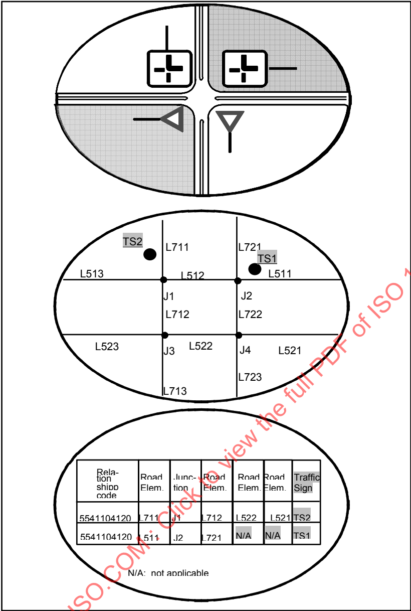
Figure 179 — Example of Right of Way Regulation
