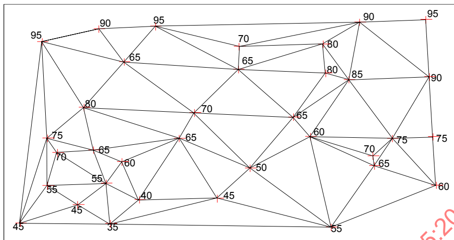
Figure 77 – Example of (full) TIN terrain elevation representation
