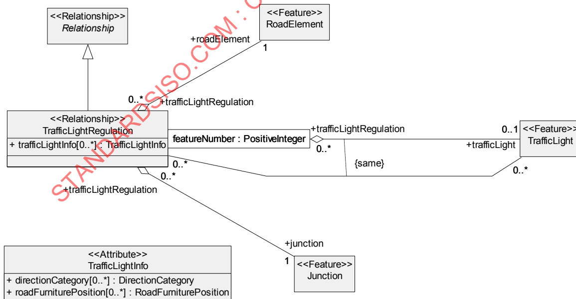
Figure 165 — The Conceptual Data Model for the Overhead Structure along Road Element Relationship
