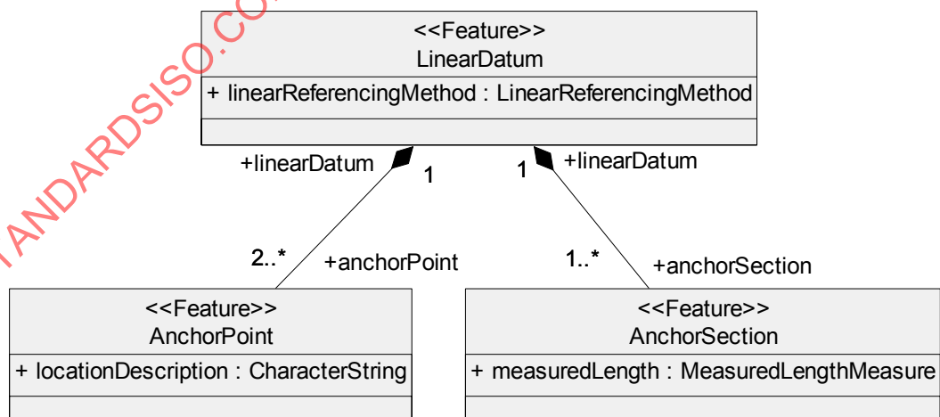
Figure 124 — The Conceptual Data Model for Attributes of Linear Datum Features
