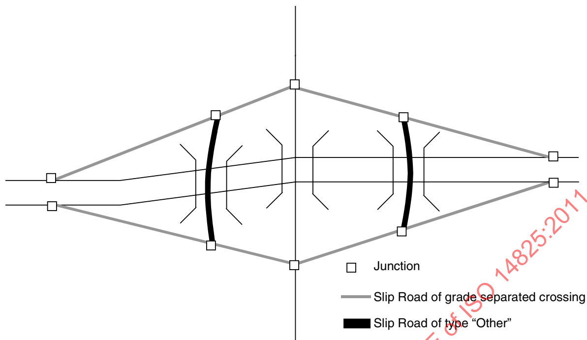
Figure 139 — Example of a Slip Road of type “Slip Road of Grade Separated Crossing” and of type “Other”
