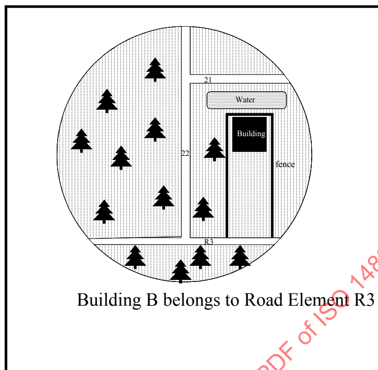
Figure 176 — Example of a Building along Road Element
