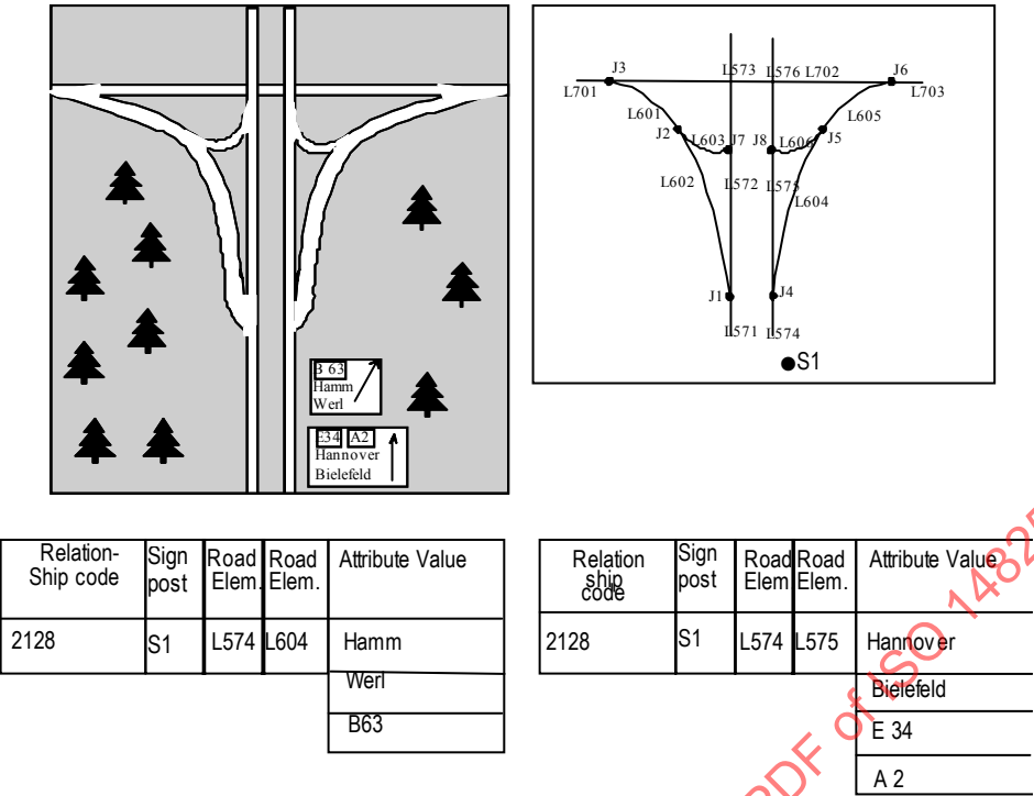
Figure 183 — Example of Signpost Information
