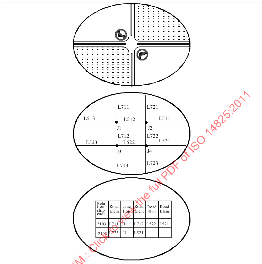
Figure 182 — Representation of a Prohibited Manoeuvre
