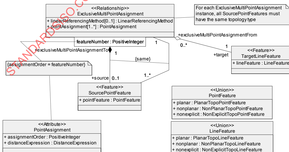
Figure 174 — The Conceptual Data Model for the Exclusive Multi-Point Assignment Relationship
