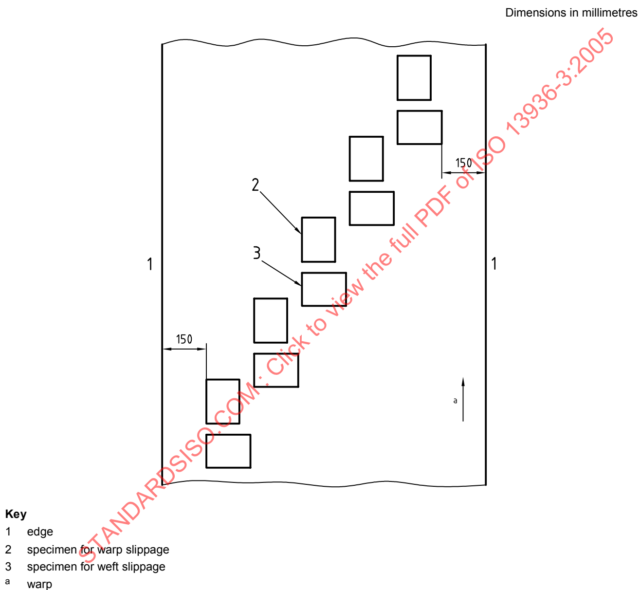
Figure B.1 — Pattern for cutting test specimens
