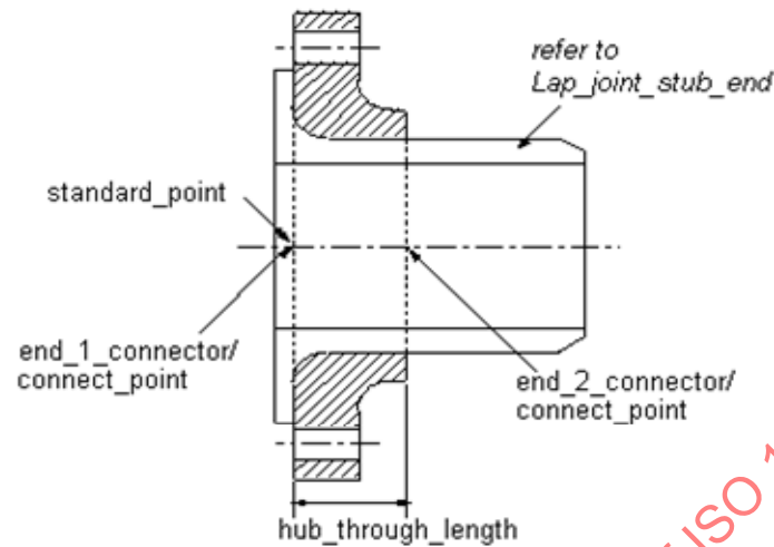
Figure 40 — Lap_joint_flange
