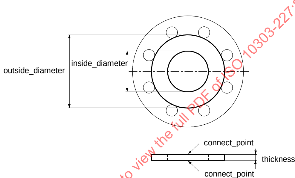
Figure 60 — Ring_spacer
