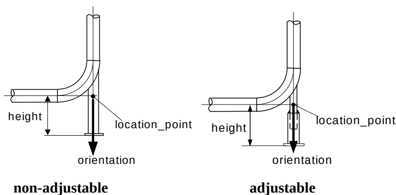
Figure 3 — Base_elbow_support
