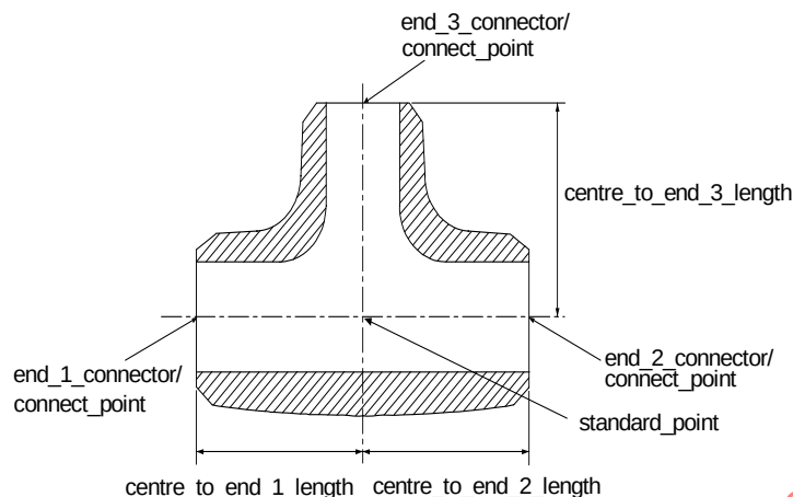
Figure 71 — Tee
