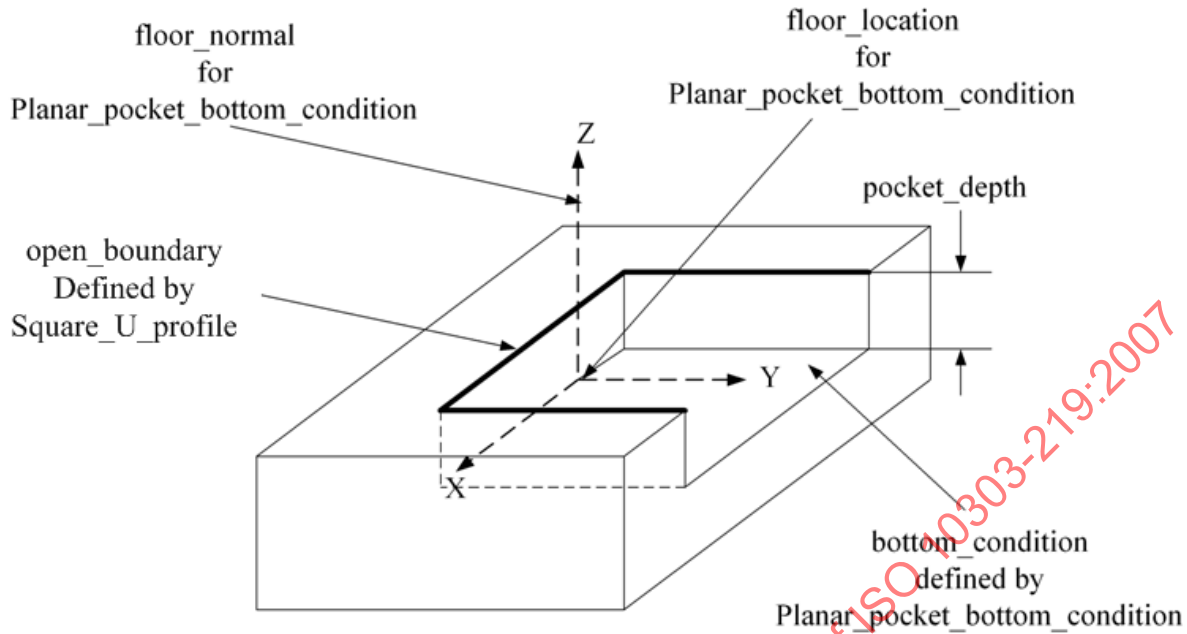
Figure 118 — Rectangular_open_pocket
