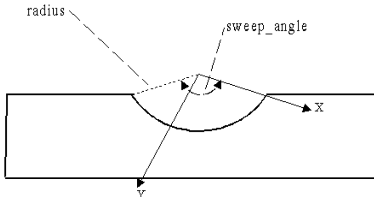
Figure 103 — Partial_circular_profile
