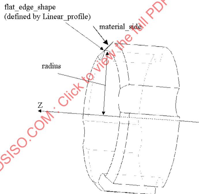
Figure 120 — Revolved_flat
