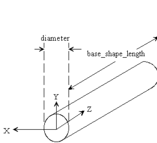
Figure 35 — Cylindrical_base_shape
