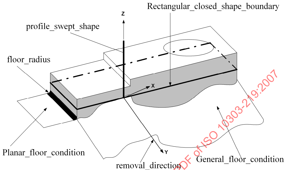
Figure 126 — Shape_profile
