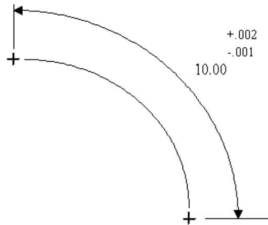
Figure 43 — Distance_along_curve_tolerance
