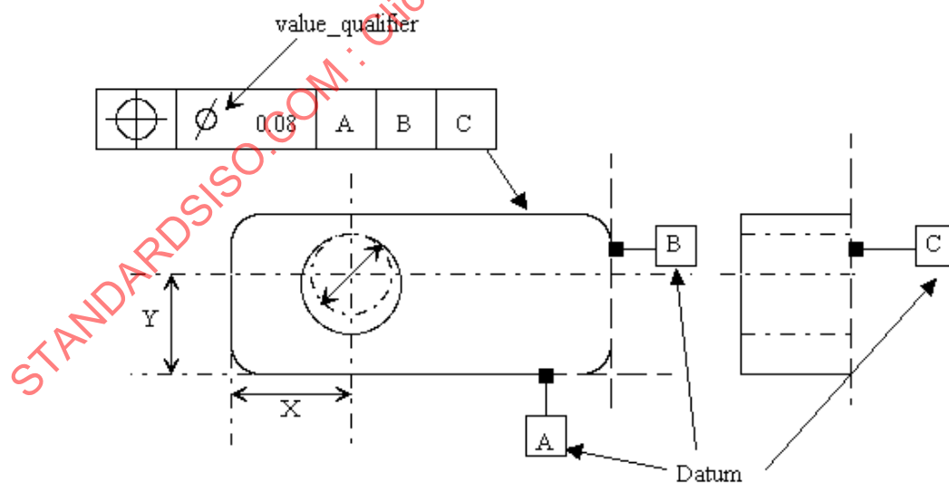
Figure 108 — Position_tolerance
