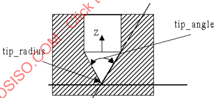
Figure 28 — Conical_hole_bottom
