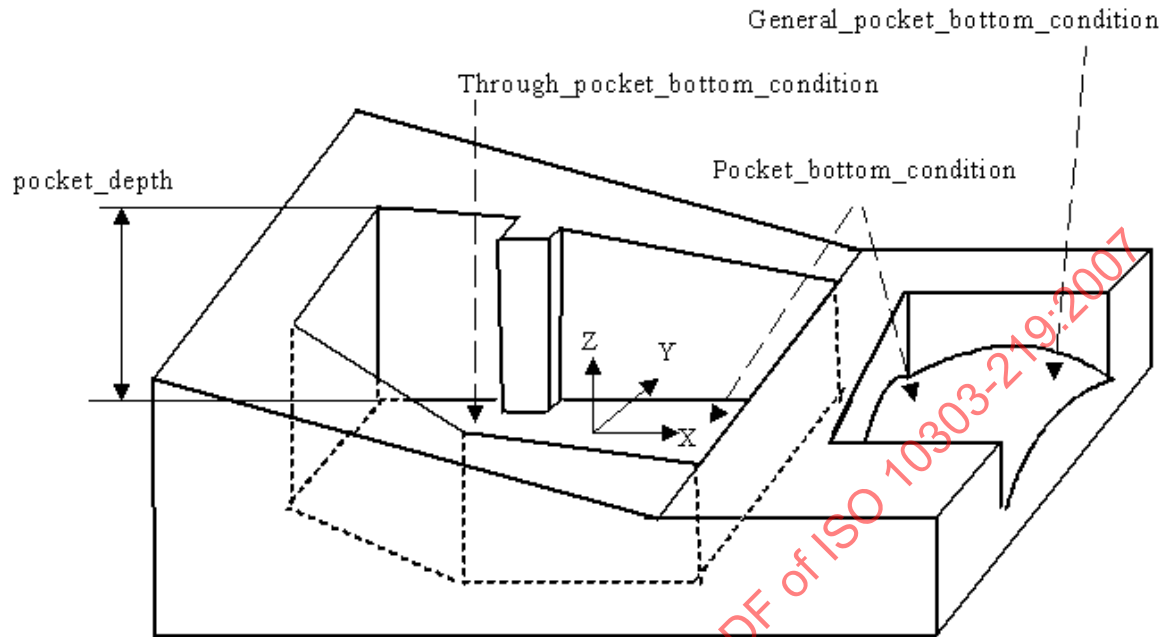
Figure 81 — General_pocket
