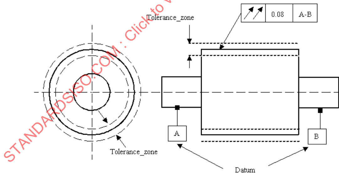
Figure 140 — Total_runout_tolerance
