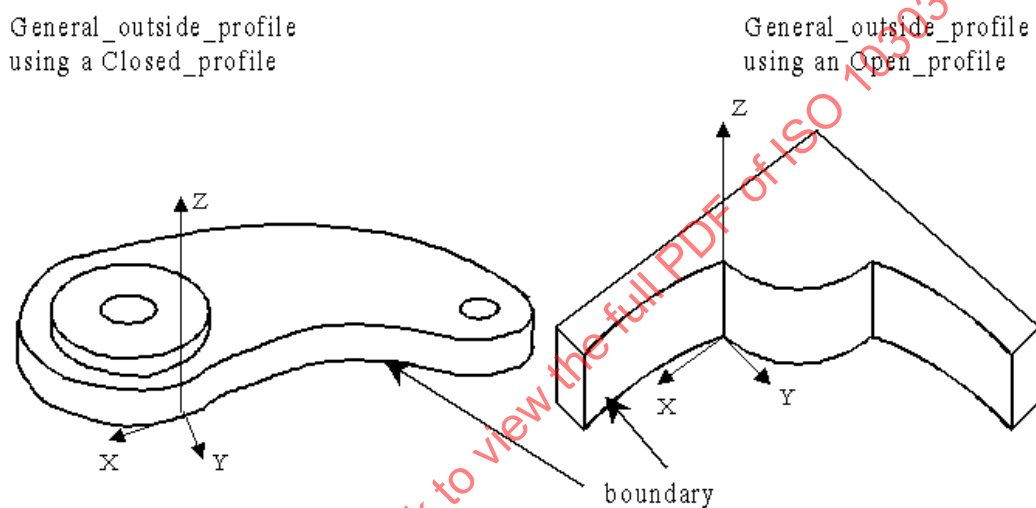
Figure 78 — General_outside_profile
