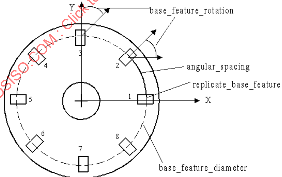
Figure 22 — Circular_pattern with rotation of a base feature
