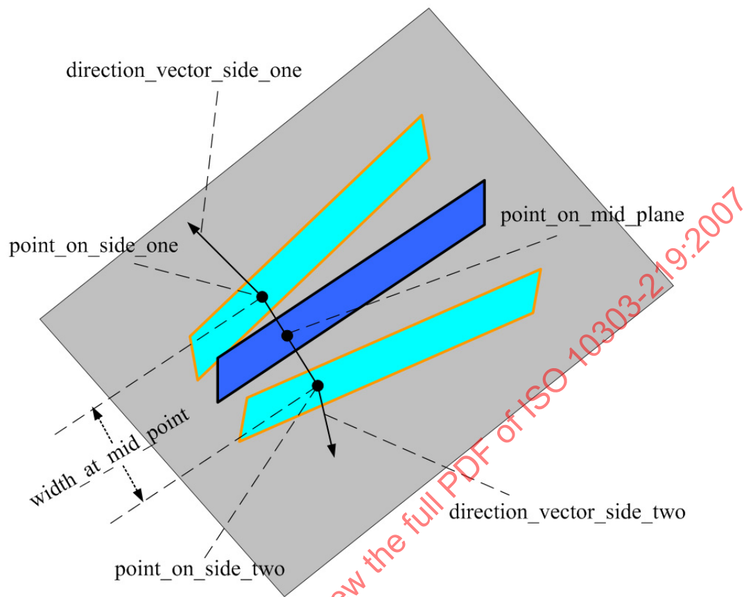
Figure 59 — Dmf_plane_symmetric
