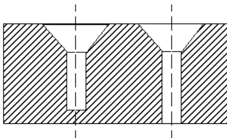
Figure 32 — Countersunk_hole
