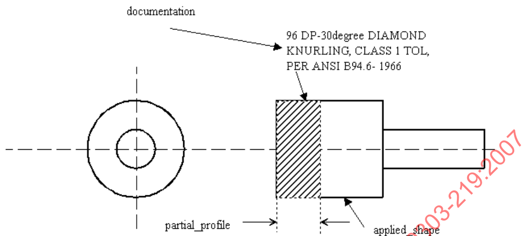
Figure 12 — Catalogue_knurl
