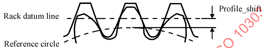
Figure 71 — Gear profile_shift
