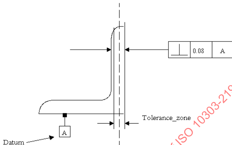
Figure 104 — Perpendicularity_tolerance
