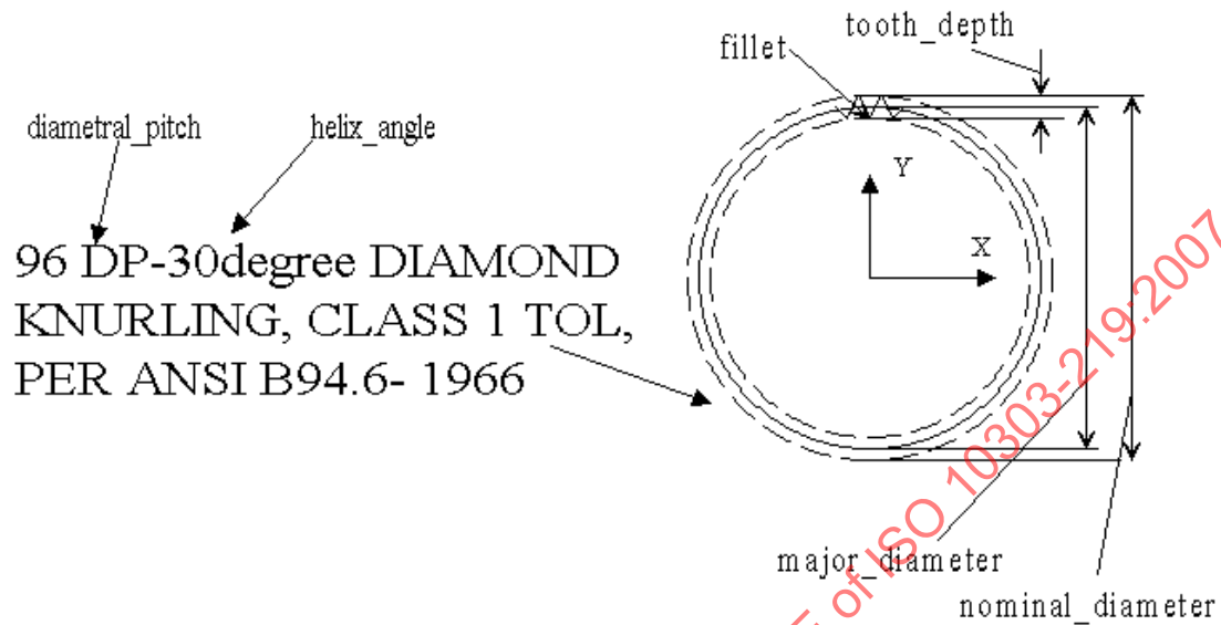
Figure 141 — Turned knurl
