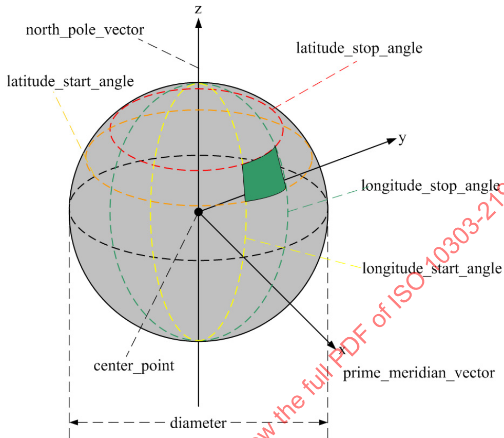
Figure 61 — Dmf_sphere
