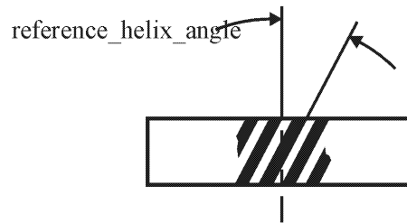
Figure 88 — Helical_gear reference_helix_angle
