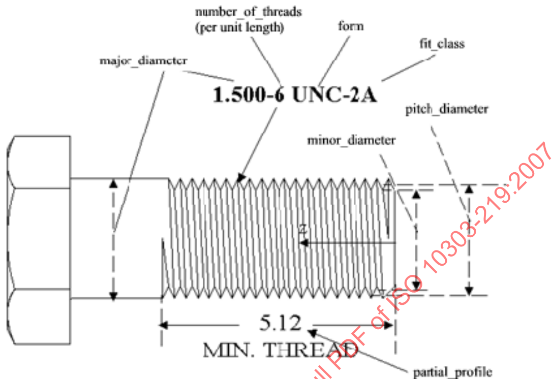
Figure 38 — Defined_thread
