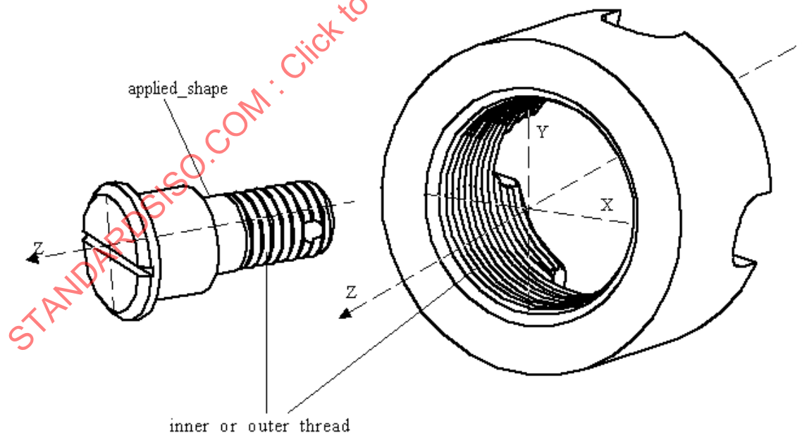
Figure 138 — Thread
