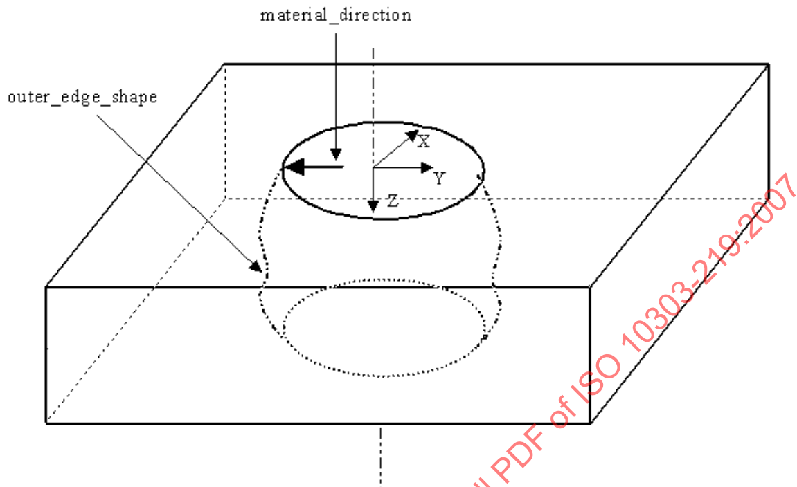
Figure 84 — General_revolution for volume removal
