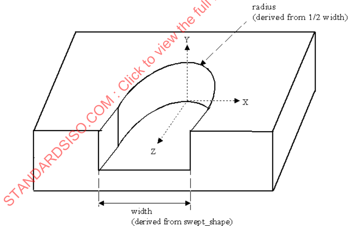
Figure 111 — Radiused_slot_end_type
