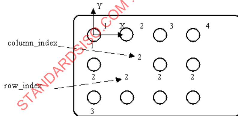
Figure 117 — Rectangular_omit_pattern
