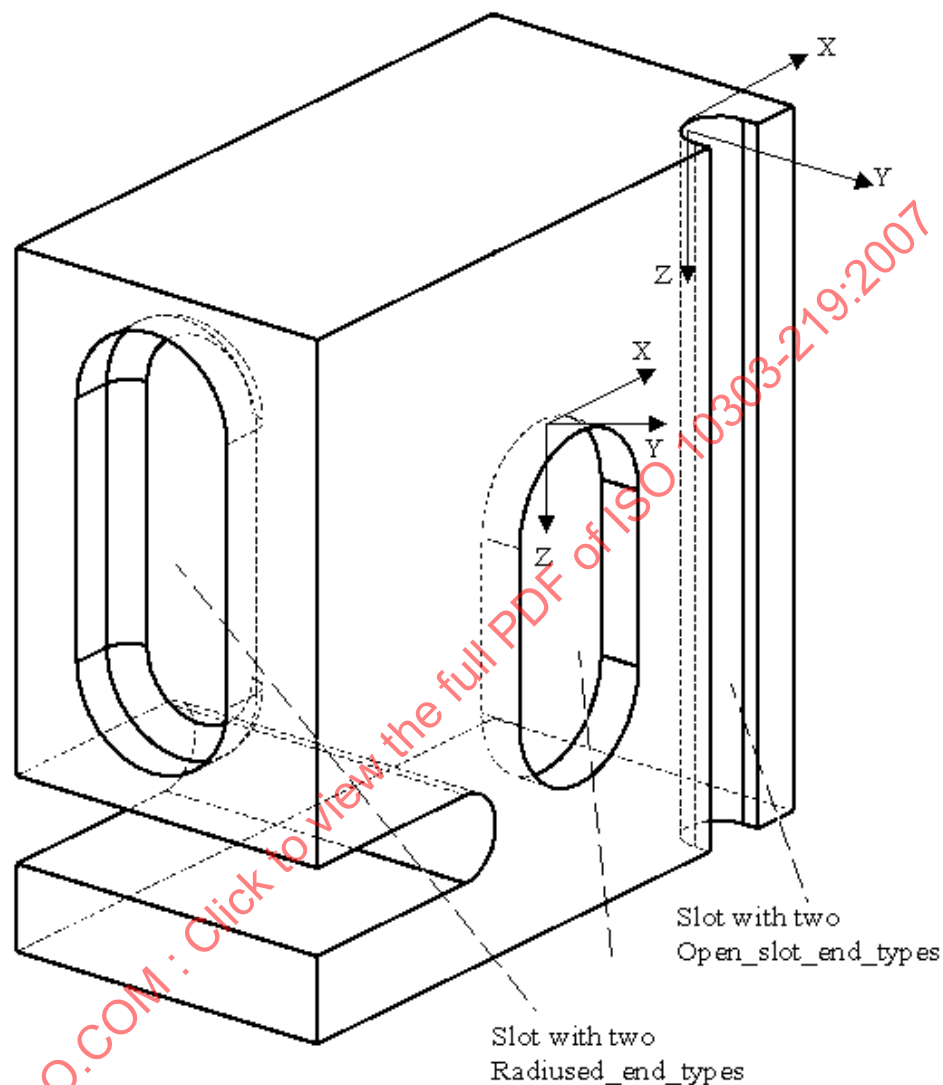
Figure 127 — Slot
