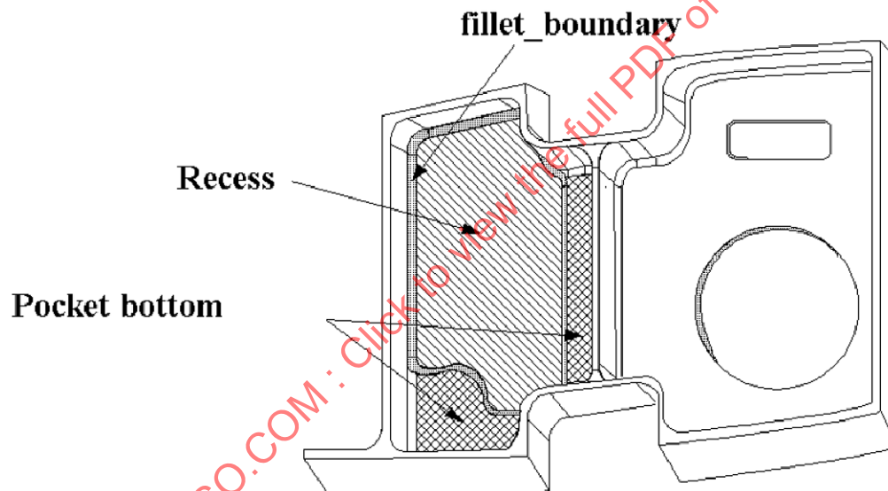
Figure 112 — Recess
