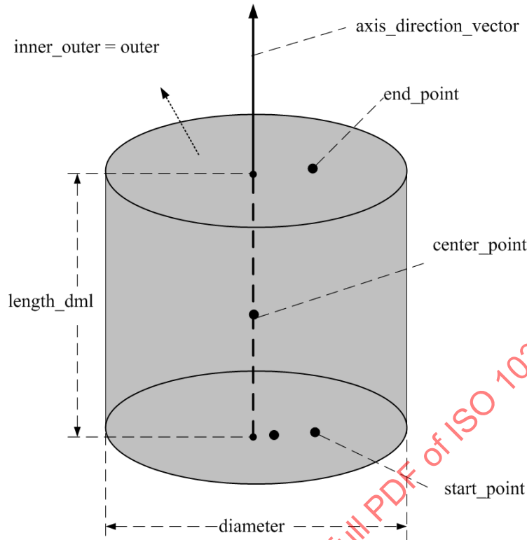
Figure 47 — Dmf_cylinder
