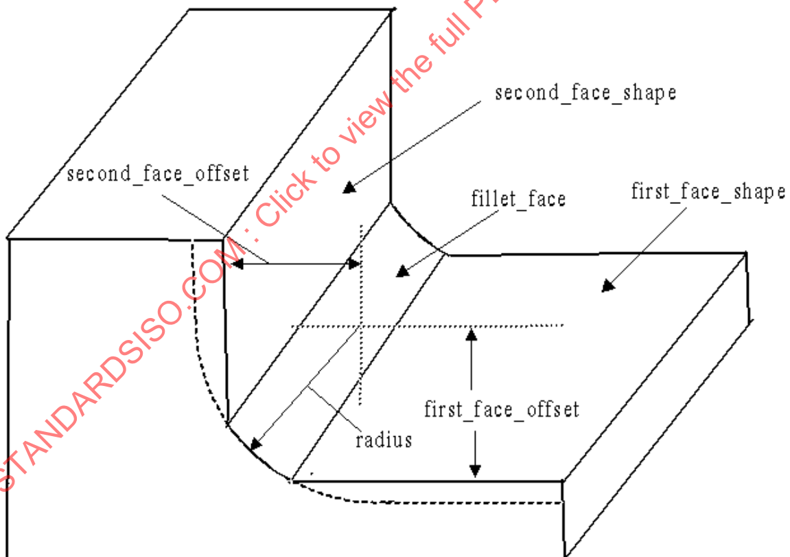
Figure 30 — Constant_radius_fillet
