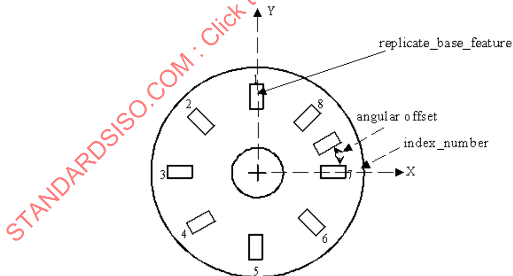
Figure 19 — Circular_offset_pattern
