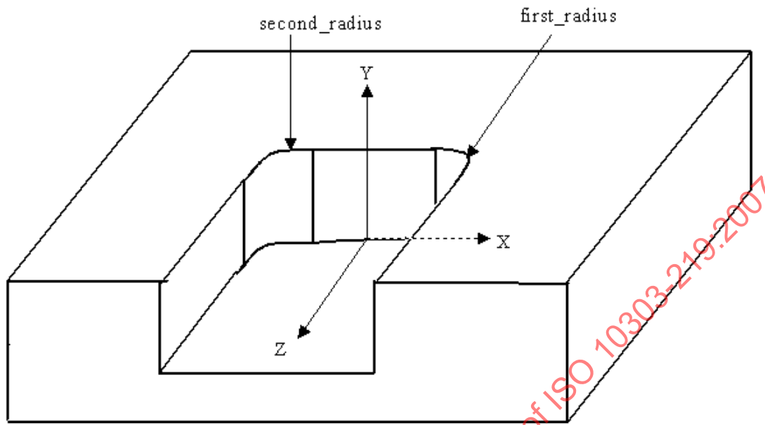
Figure 67 — Flat_slot_end_type
