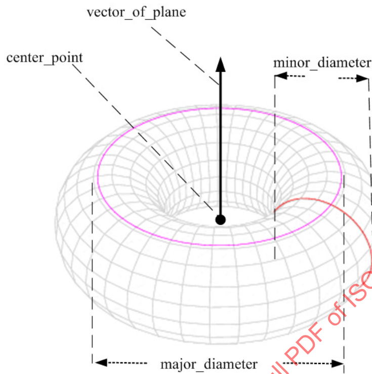
Figure 63 — Dmf_torus
