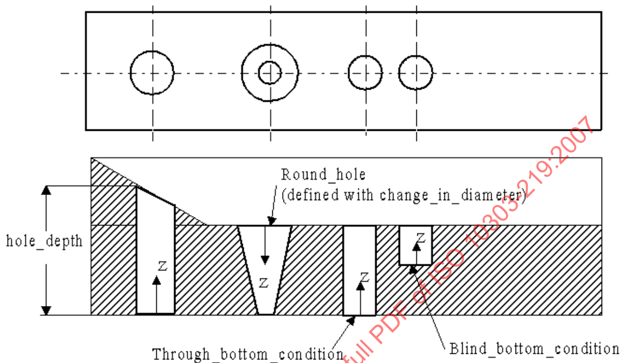
Figure 123 — Round_hole
