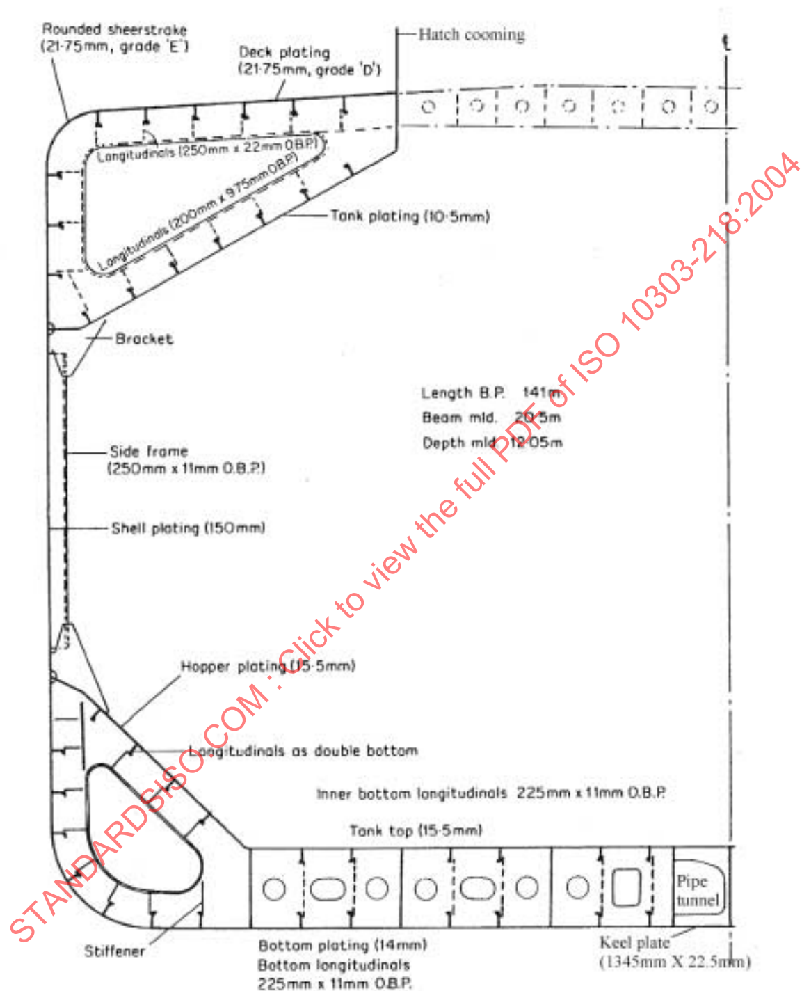
Figure 26 — Hull cross section of a bulk carrier
