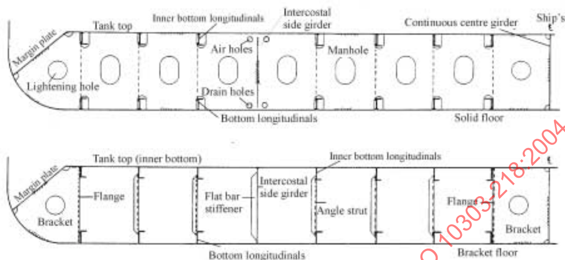
Figure 56 — Longitudinal girder
