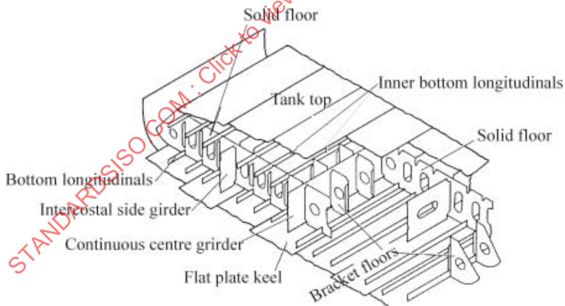
Figure 46 — Double bottom
