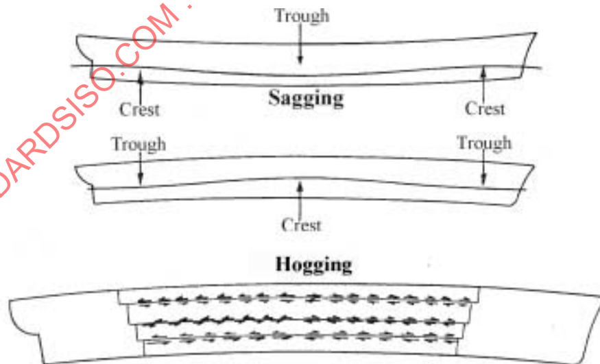
Figure 5 — Bending moment
