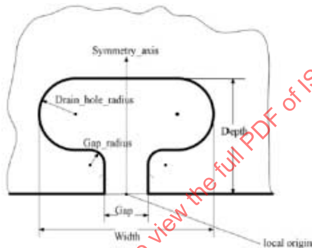
Figure 17 — Drain_hole_cutout
