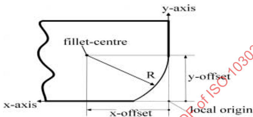
Figure 29 — Outward_round_corner_cutout
