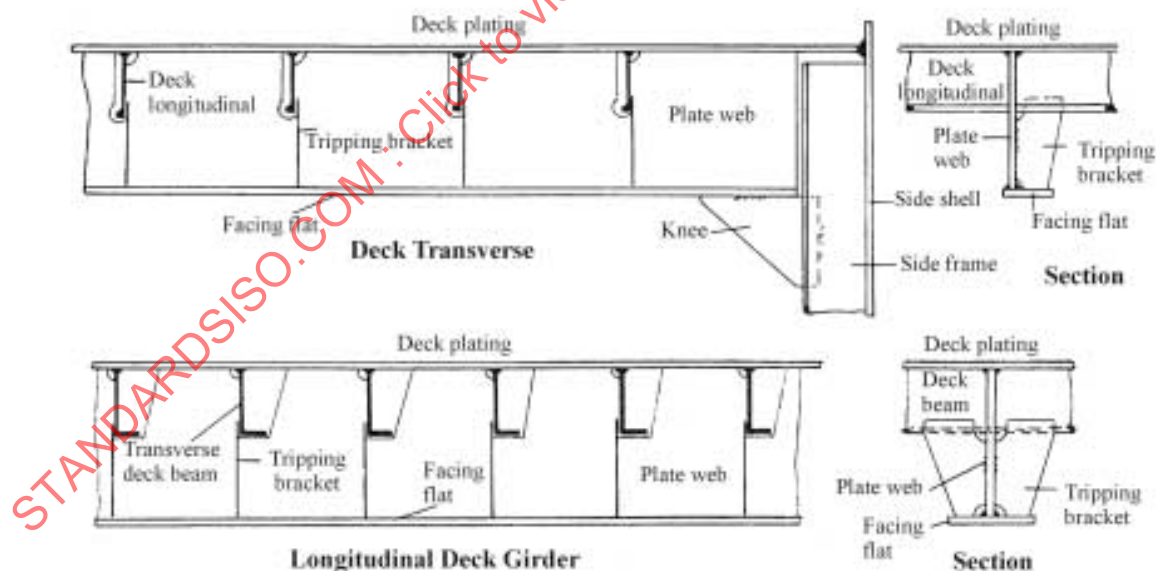
Figure 43 — Deck
