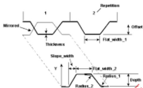
Figure 13 — Corrugated part parameters
