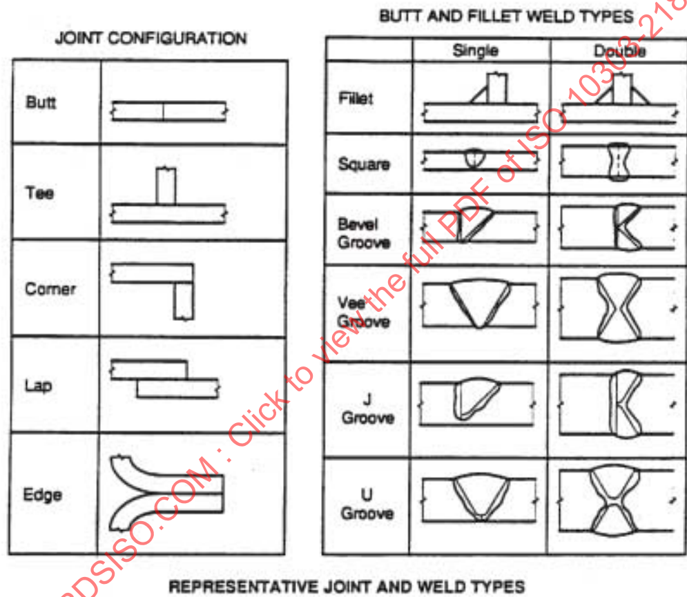
Figure 65 — Weld types
