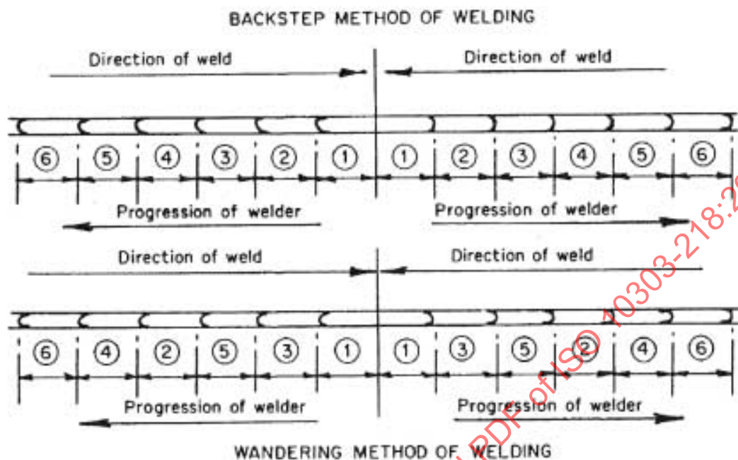
Figure 63 — Weld methods
