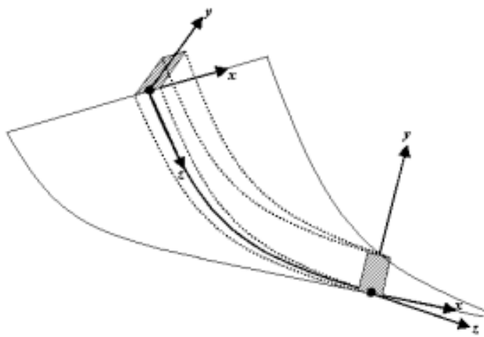
Figure 34 — Profile design using curve_on_surface geometry for trace line
