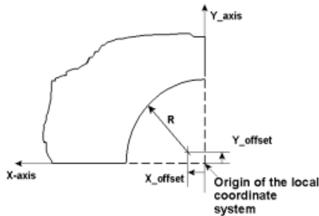
Figure 27 — Inward_round_corner_cutout
