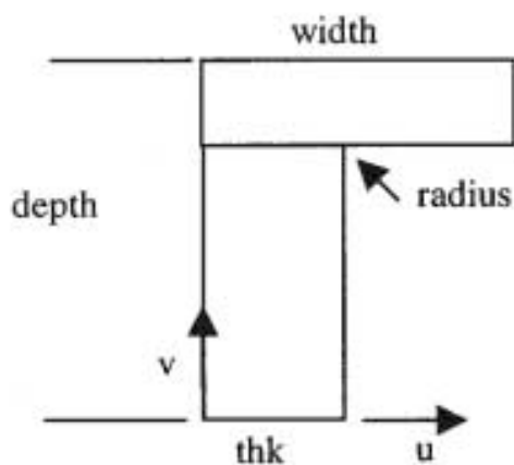
Figure 3 — Angle_bar_cross_section
