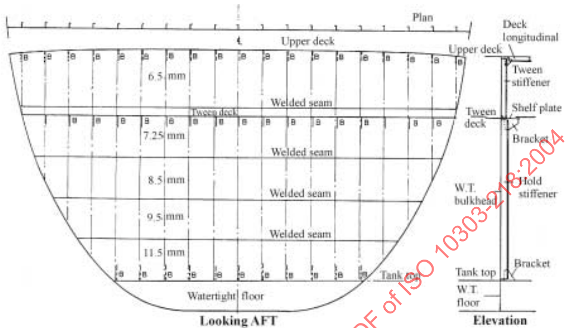
Figure 44 — Bulkhead
