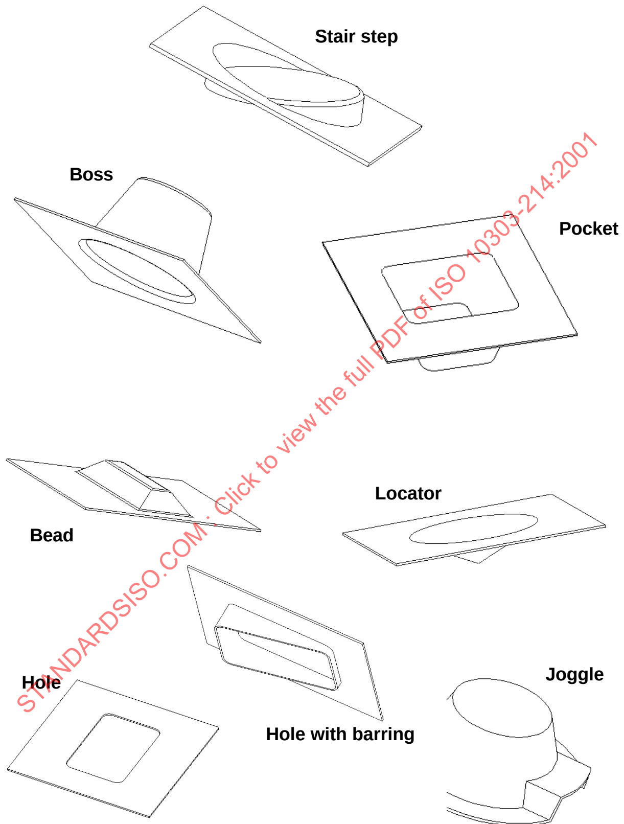
Figure 4 – Features for sheet-type parts
