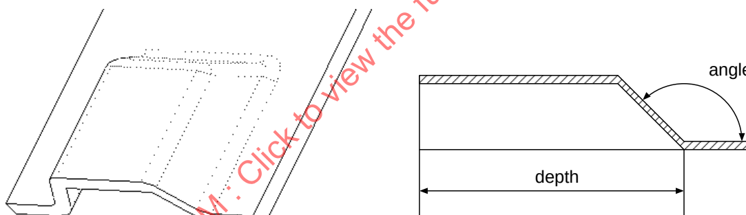
Figure 76 – Value terminated joggle feature
