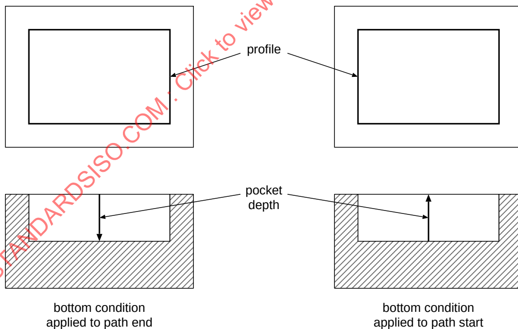
Figure 54 – Sweep path for pocket features
