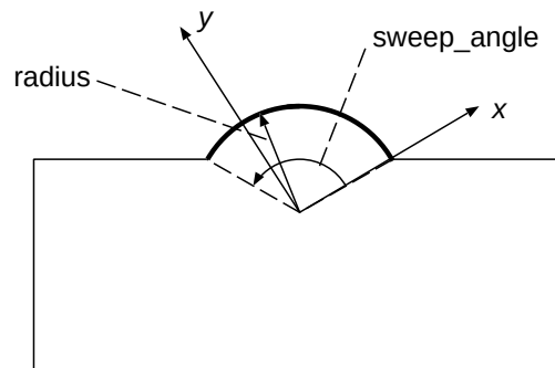
Figure 53 – Definition of a Partial_circular_profile
