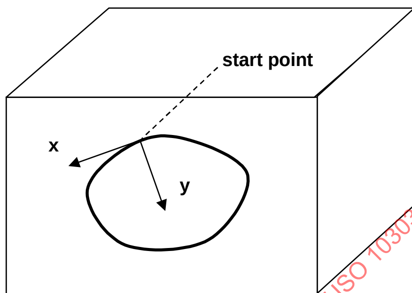
Figure 36 – Definition of a General closed_profile
