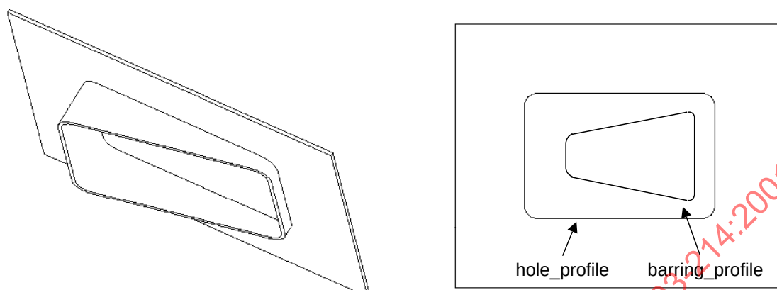
Figure 51 – Parameters defining a Panel_hole_with_barring
