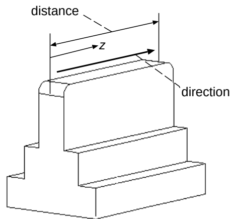
Figure 48 – Definition of a Linear_path
