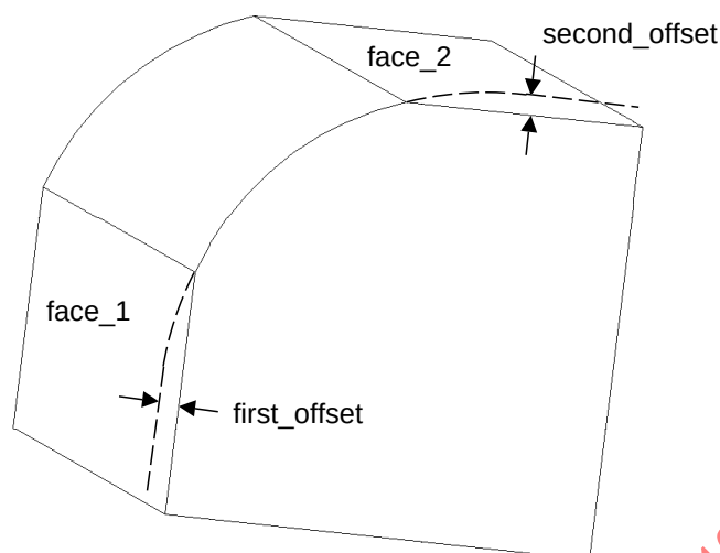
Figure 22 – Parameters defining an edge round with constant radius by offsets
