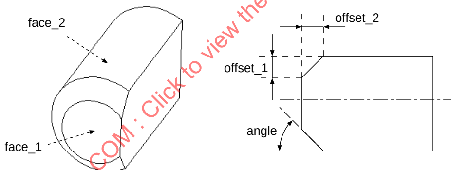
Figure 13 – Parameters defining a Chamfer
