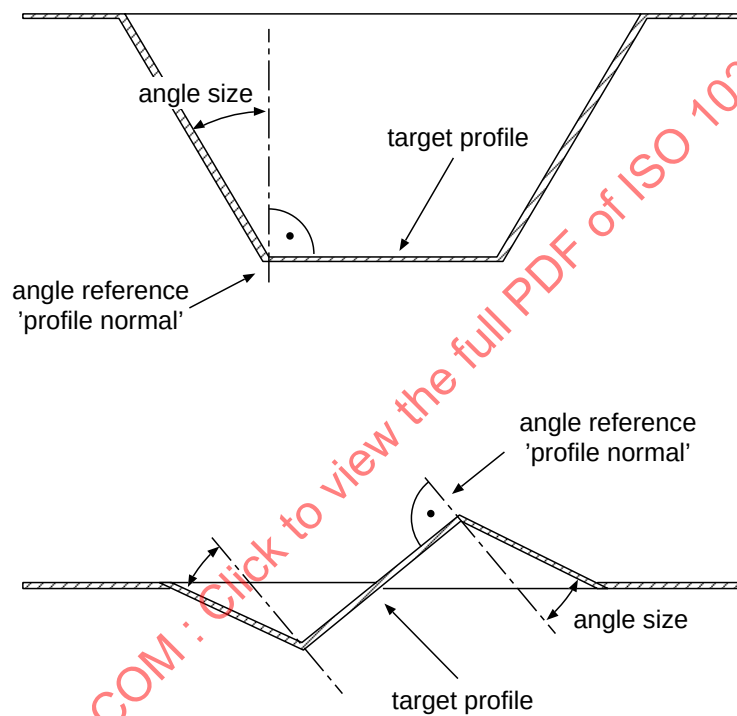
Figure 7 – Form features in panel defined by target boundaries and wall angles
