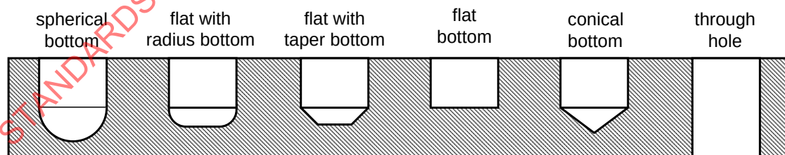
Figure 45 – Cross sections of holes
