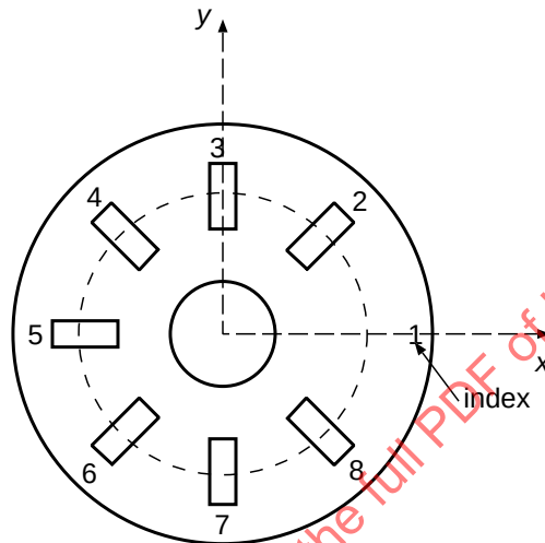
Figure 17 – Parameters defining an omission in a circular pattern
