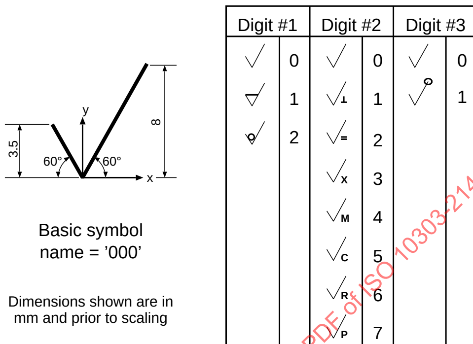
Figure 70 – Pre-defined surface condition symbols
