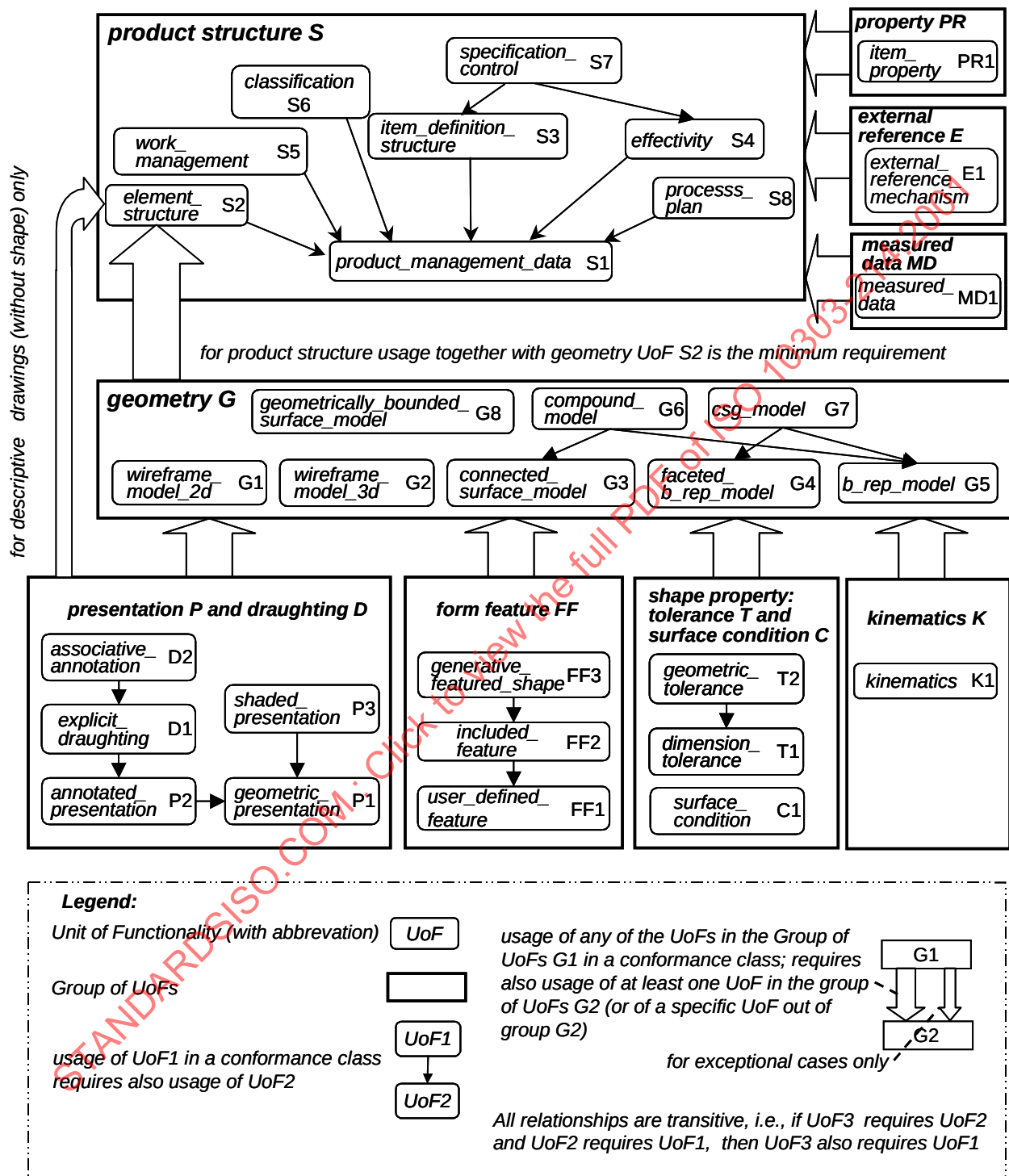
Figure 85 – Interdependencies among UoFs
