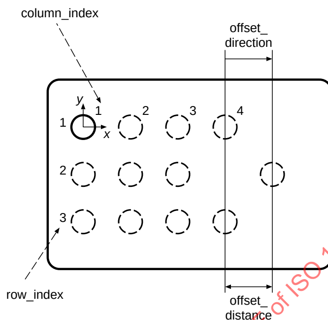
Figure 61 – Parameters defining an offset in a rectangular pattern
