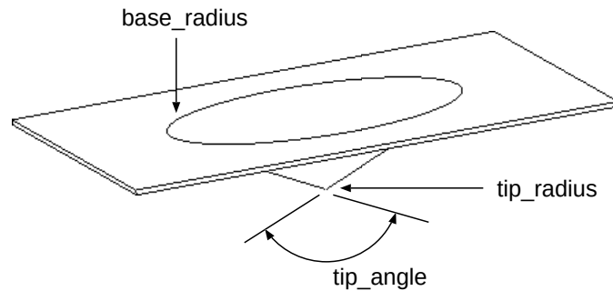
Figure 49 – Parameters defining a Locator_feature
