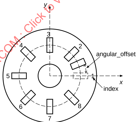
Figure 16 – Parameters defining an offset in a circular pattern
