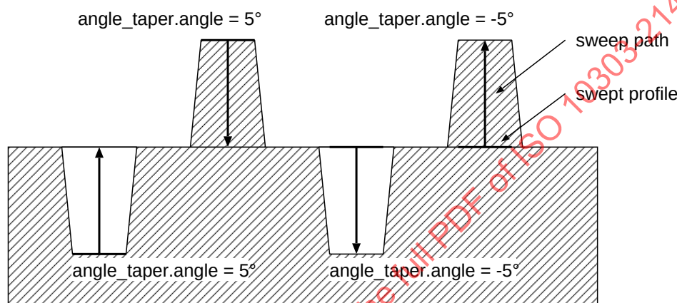
Figure 8 – Parameters defining an Angle_taper
