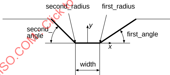
Figure 69 – Definition of a Square_u_profile
