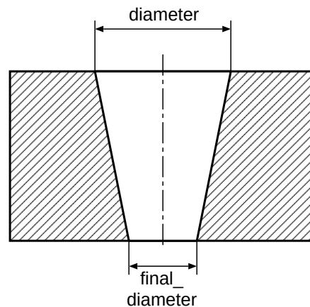
Figure 28 – Definition of a taper by two diameters
