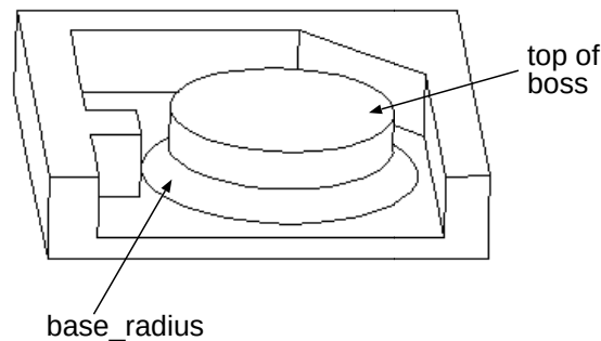
Figure 14 – Parameters defining a Circular_boss
