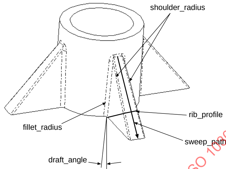
Figure 63 – Parameters defining a Rib_feature
