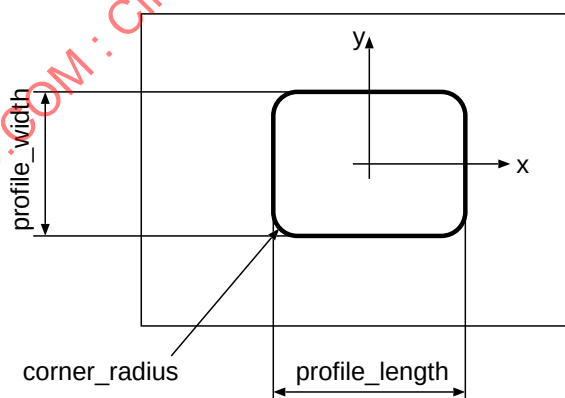
Figure 60 – Definition of a Rectangular_closed_profile
