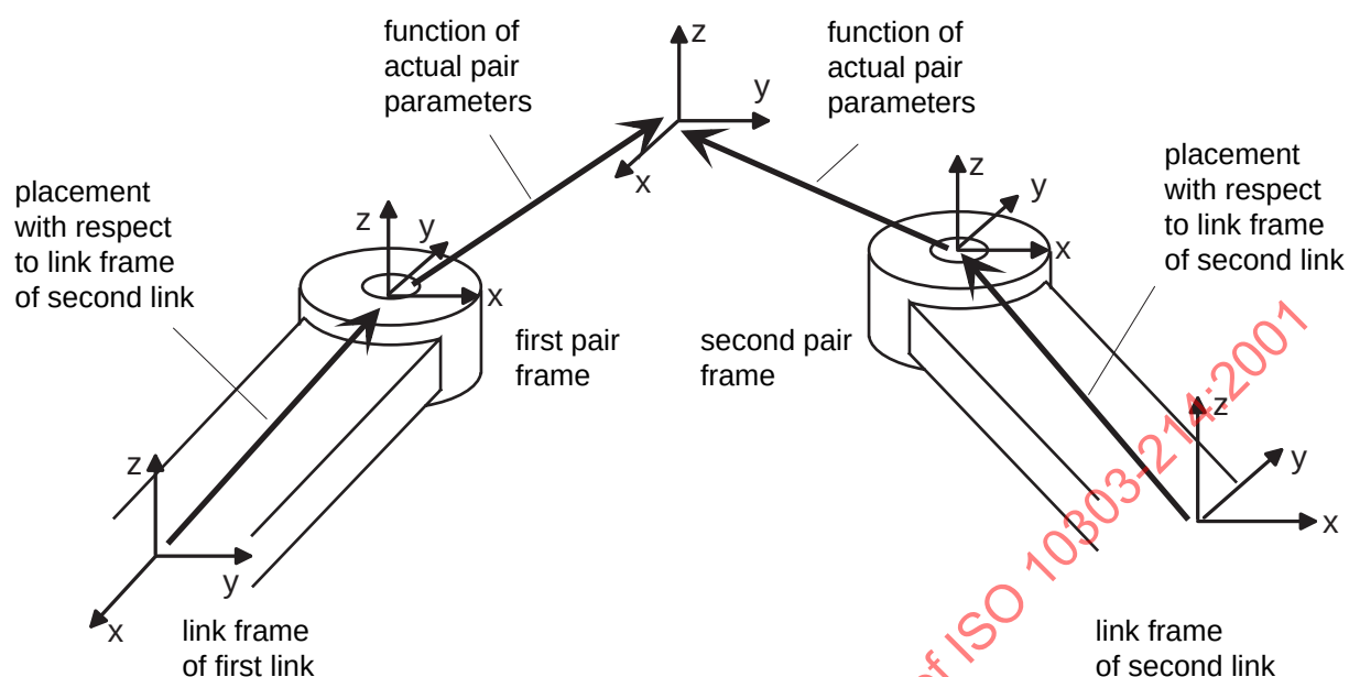
Figure 47 – Placement relationships kinematic pair frames and mating links
