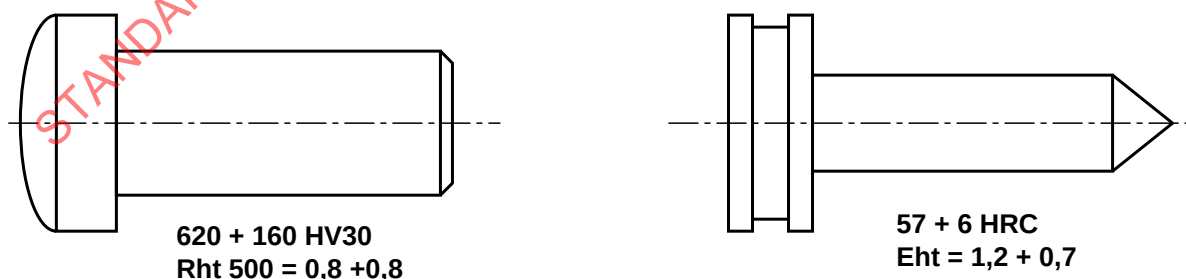
Figure 44 – Hardness
