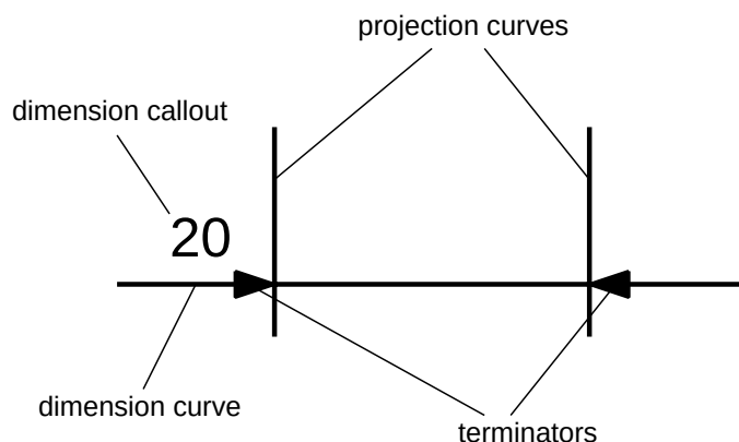
Figure 29 – Components of a dimension in a drawing
