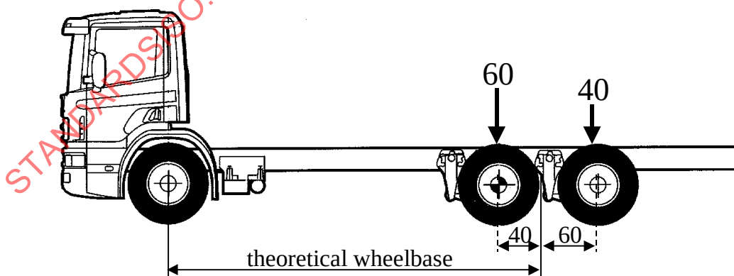
Figure 40 – Theoretical wheelbase of a truck
