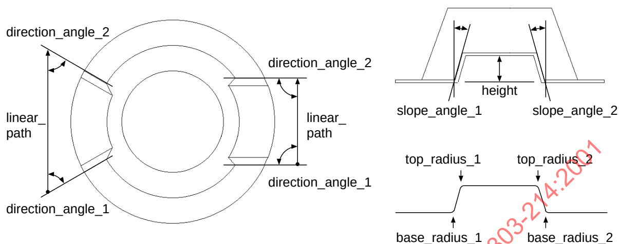
Figure 46 – Parameters defining a Joggle feature
