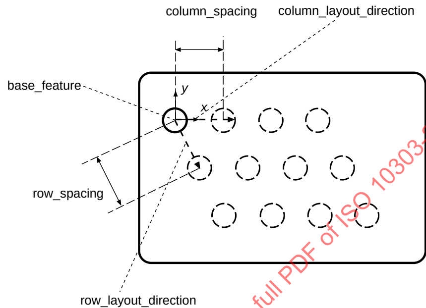
Figure 62 – Parameters defining a Rectangular_pattern
