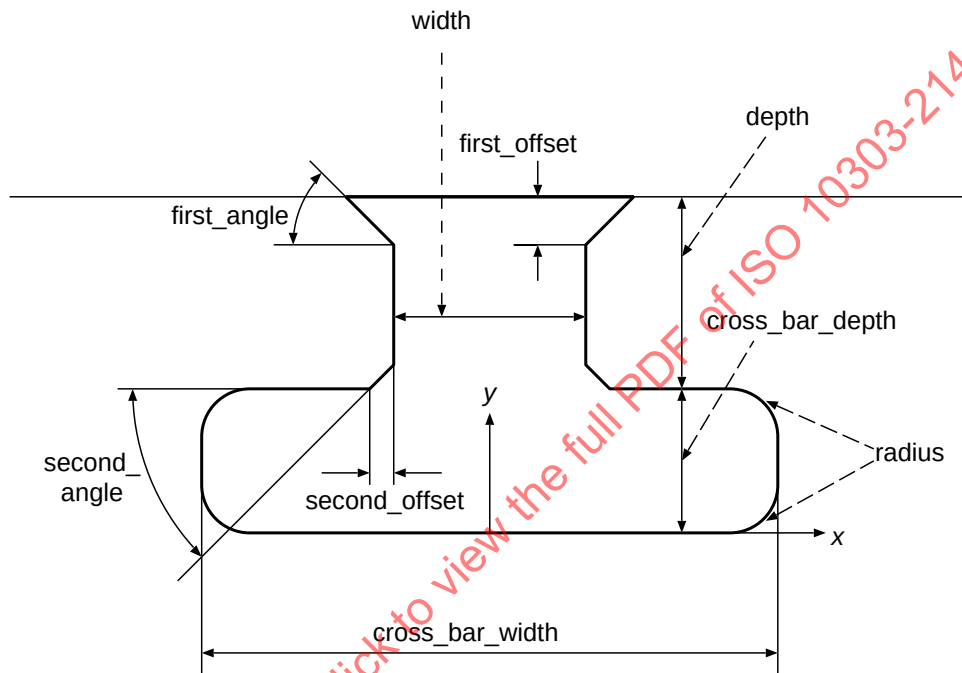
Figure 71 – Definition of a Tee_profile
