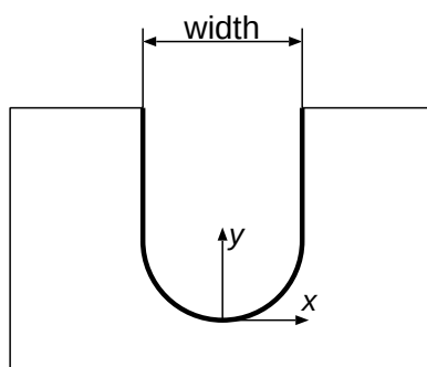
Figure 65 – Definition of a Rounded_u_profile
