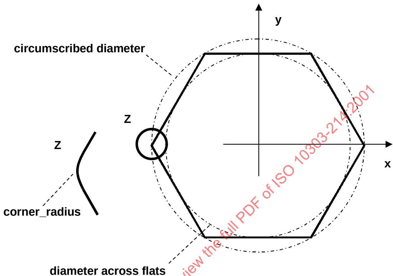
Figure 50 – Definition of a Ngon_profile
