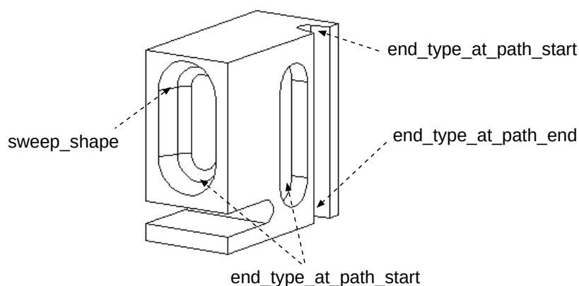
Figure 68 – various shapes of slots
