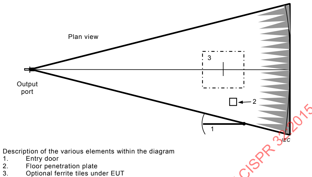
Figure I.2 – Typical GTEM plan sectional view showing floor layout
