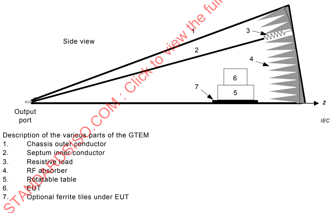
Figure I.1 – Typical GTEM side sectional view showing some basic parts
