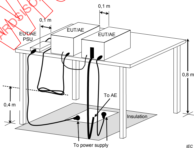
Figure D.8 – Example measurement arrangement for table-top EUT (Radiated emission measurement)
