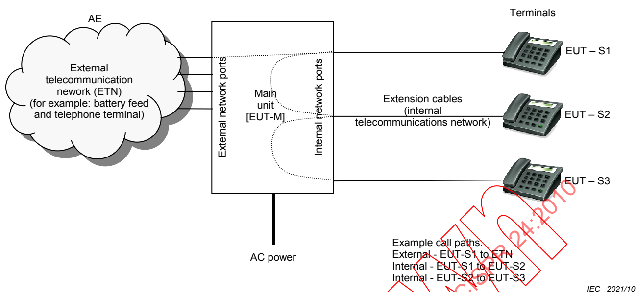
Figure A.5 – Example of typical small key telephone system or PABX
