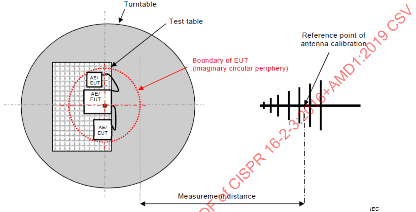
Figure 8 – Measurement distance
