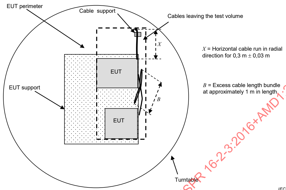
Figure 19 – Test set-up for floor-standing equipment – Top view
