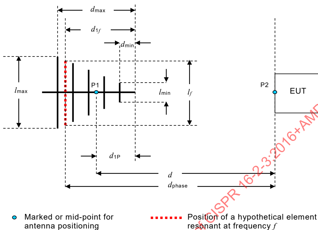
Figure 9 – Separation distance relative to the phase centre of an LPDA antenna
