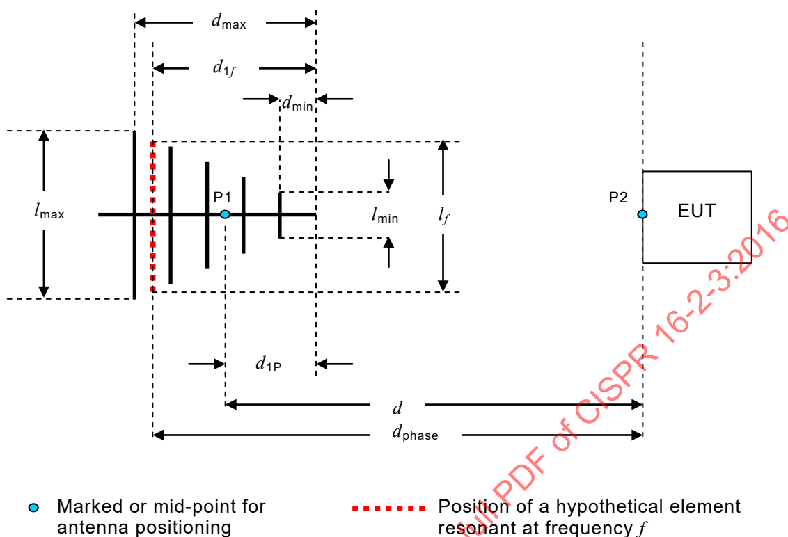
Figure 9 – Separation distance relative to the phase centre of an LPDA antenna
