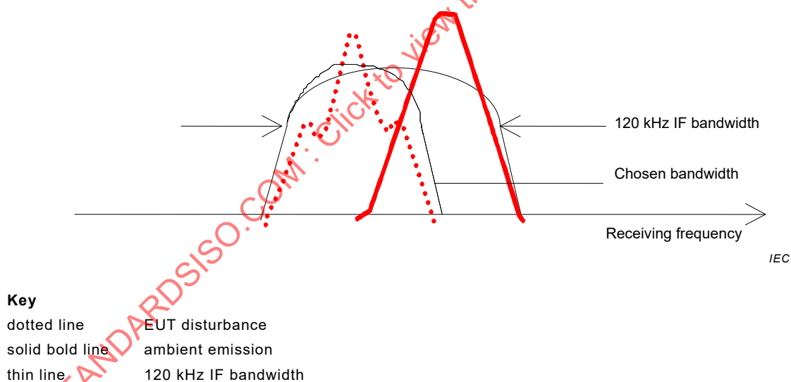
Figure A.4 – Disturbance by an amplitude-modulated signal (dotted line)
