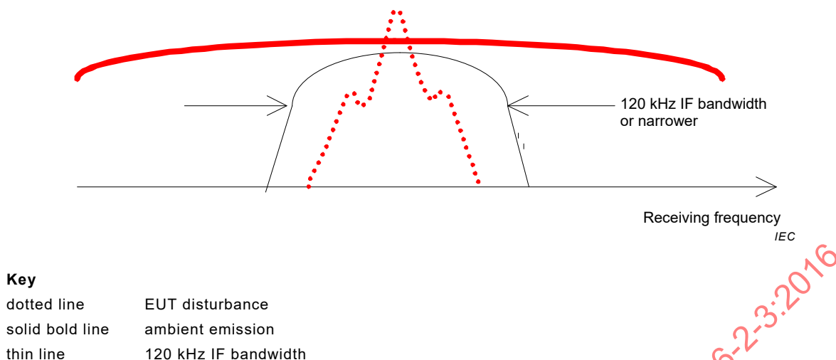
Figure A.9 – Amplitude-modulated EUT disturbance (dotted line)
