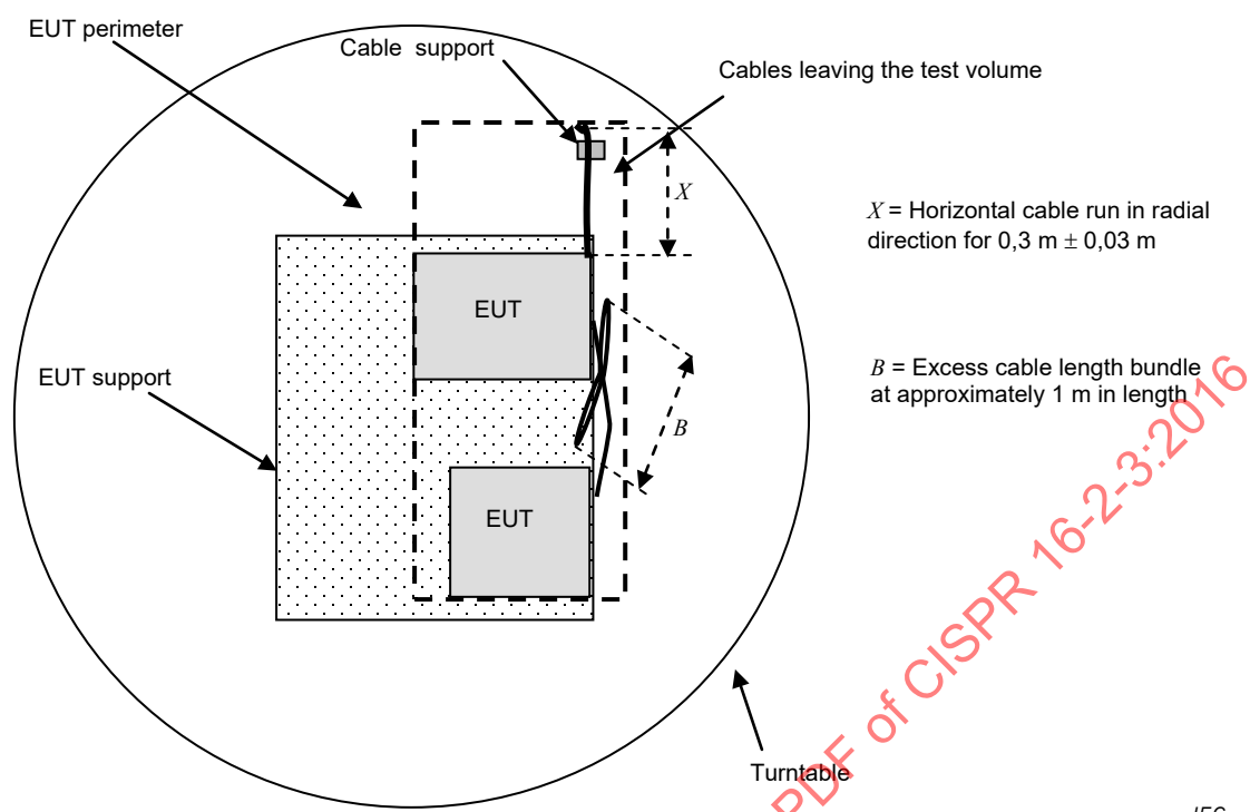
Figure 19 – Test set-up for floor-standing equipment – Top view
