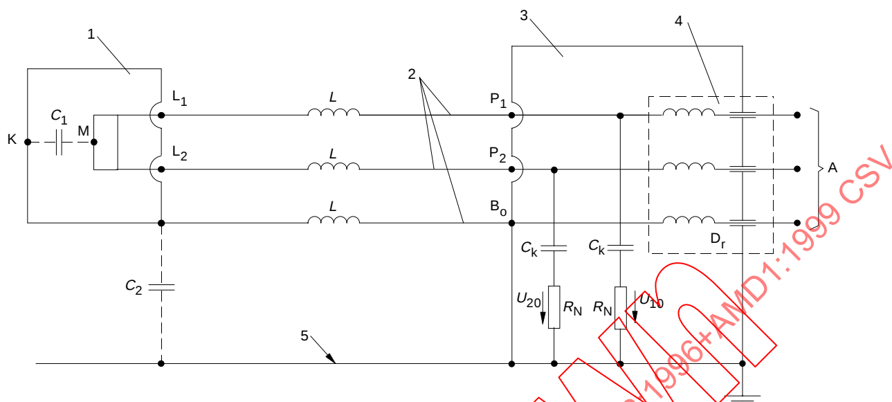
Figure 6a – Schematic for measurement and power circuit
