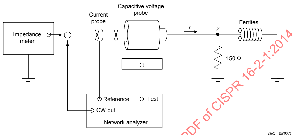
Figure G.4 – Basic test set-up to measure combined impedance of the 150 Ω and ferrites
