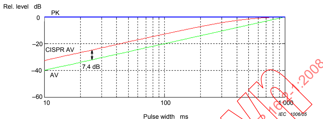
Figure D.3 – Example of weighting functions (of a 1 Hz pulse) for peak (“PK”) and average detections as a function of pulse width: meter time constant 160 ms
