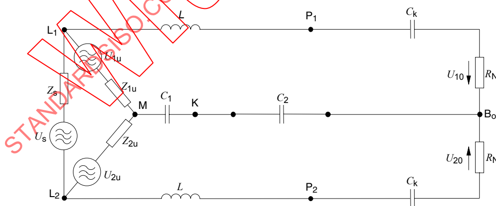
Figure 13b – Equivalent RFI source and measurement circuit
