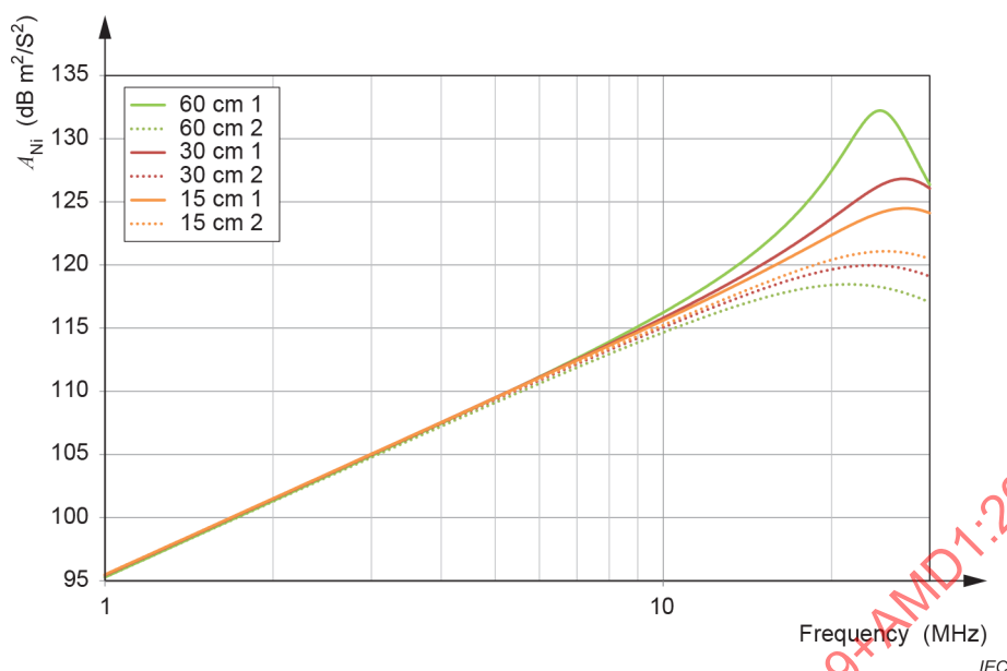
Figure J.3 – Variation of NSIL values for various set-ups, for a distance of 3 m, h = 1,3 m
