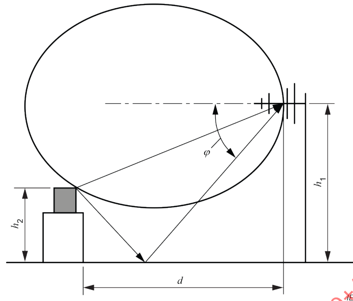
Figure 1 – Schematic of radiation from EUT reaching an LPDA antenna directly and via ground reflection at a 3 m site, showing the beamwidth half-angle, \phi , at the reflected ray
