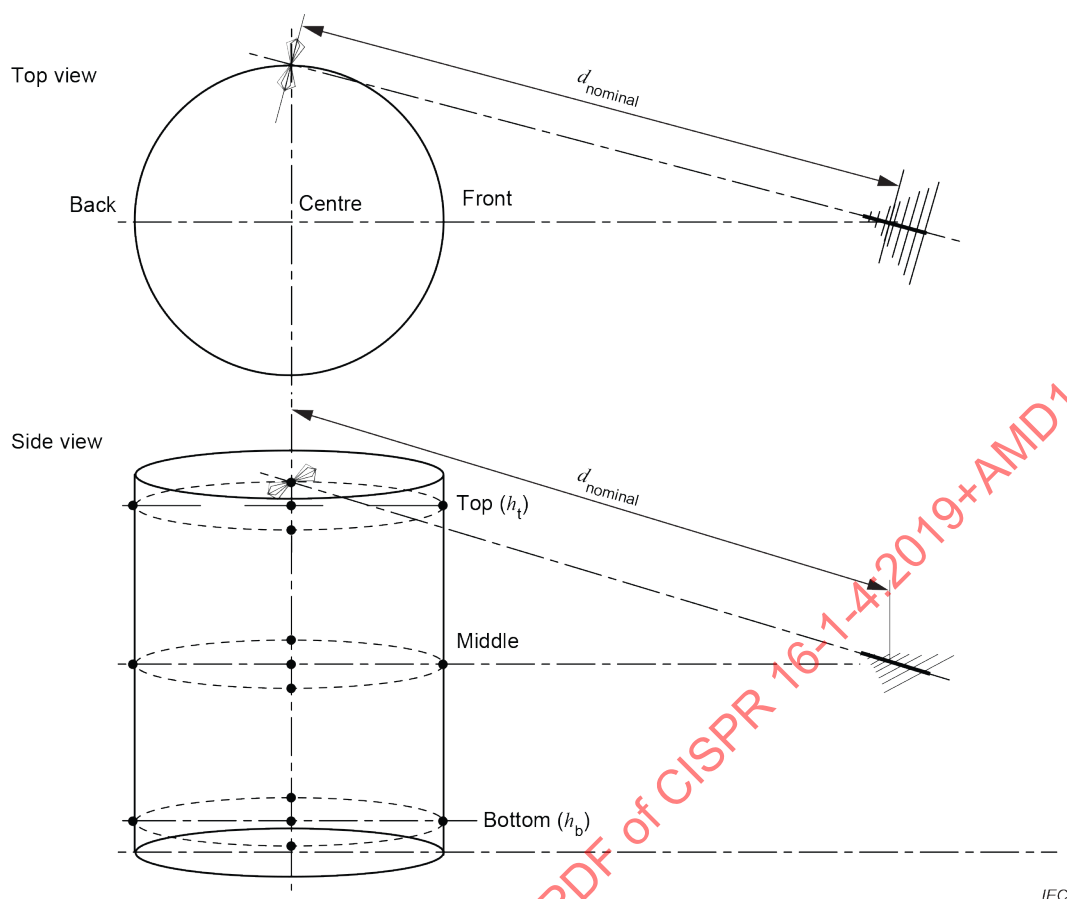
Figure 16 – Example of one measurement position and antenna tilt for FAR site validation
