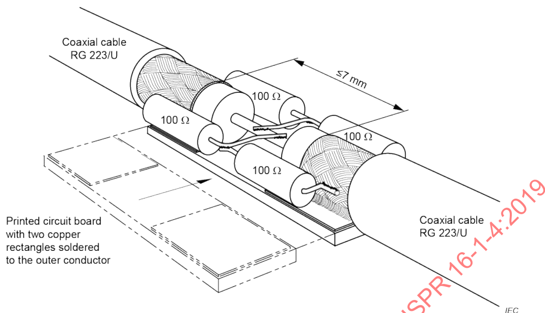
Figure C.4 – Example of an LLA slit construction using a strap of printed circuit board to obtain a rigid construction
