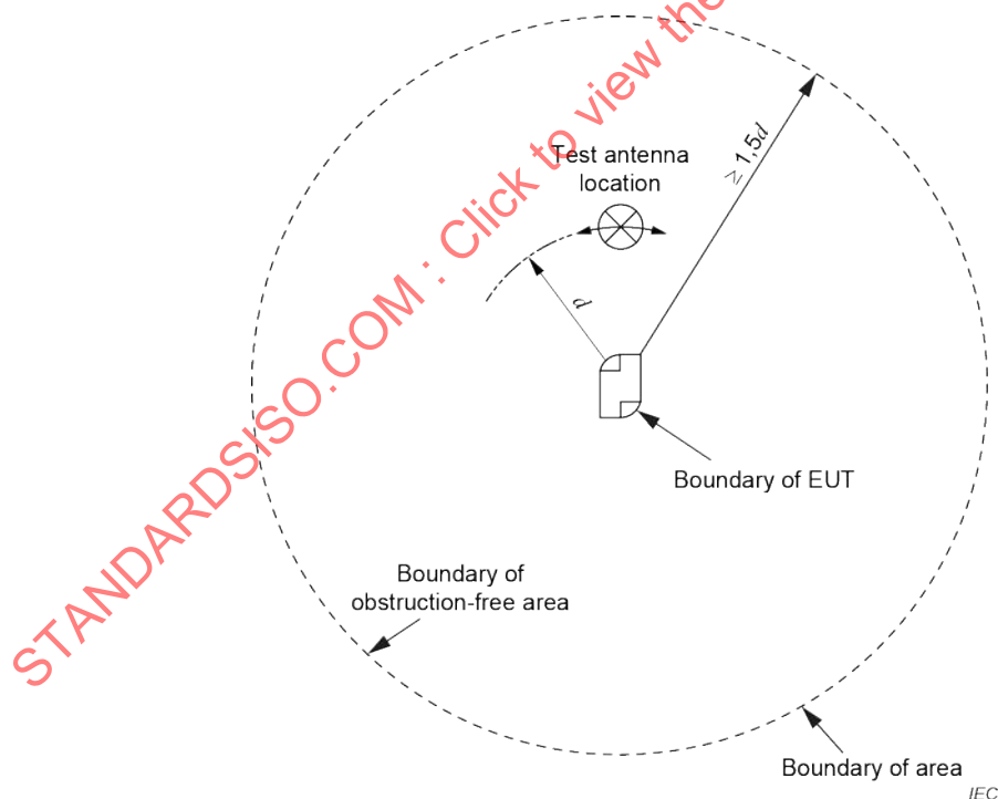
Figure 6 – Obstruction-free area with stationary EUT
