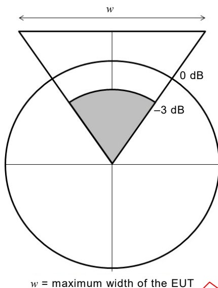
Figure 44 – Determination of maximum useable EUT width using half power beam-width
