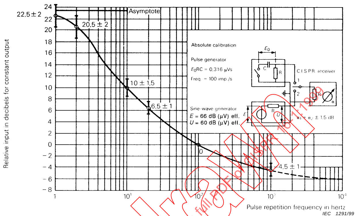
Figure 1b – Pulse response curve (see 4.1.4.2) (Band B)
