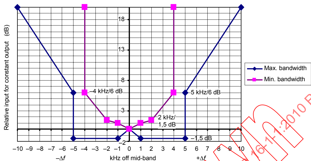
Figure 2b) – Limits of overall selectivity – Pass band (see 4.5.1, 6.55.6, 6.56.6, 7.6) (Band B)
