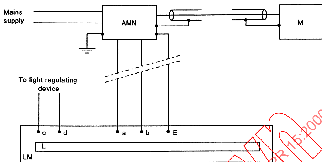
Figure 6a – Luminaires
