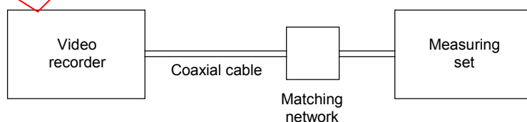
Figure 9 – Circuit arrangement for the measurement of the wanted signal and disturbance voltage at the RF output of video recorders (see 5.5.2)
