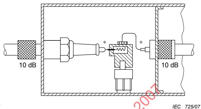
Figure E.10 – Noise suppression distributor rotor
