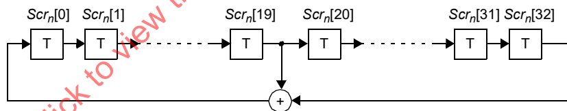
Figure 146–8—A realization of side-stream scramblers by linear feedback shift registers
