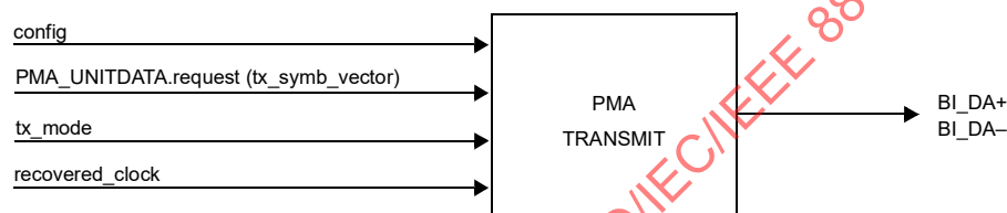
Figure 146–13—PMA Transmit
