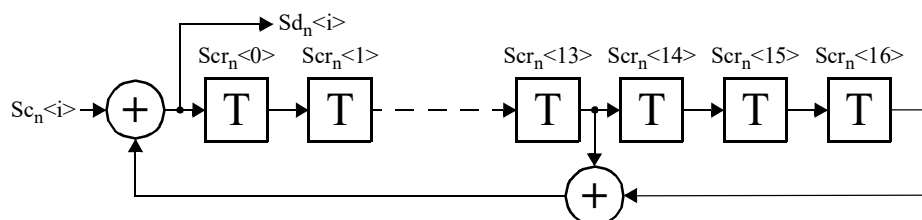
Figure 147-6—Self-synchronizing scrambler
