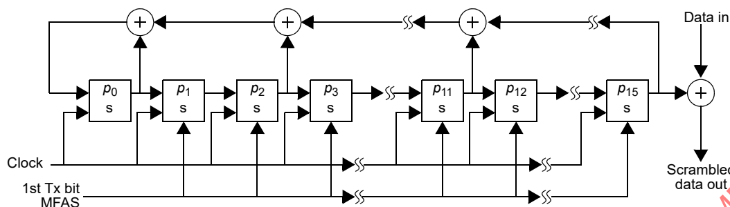
Figure 153-5—Frame synchronous scrambler
