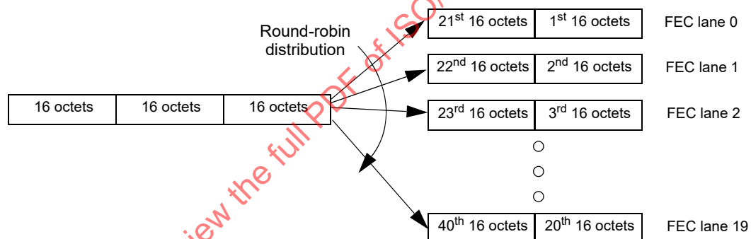
Figure 153-6—Lane distribution
