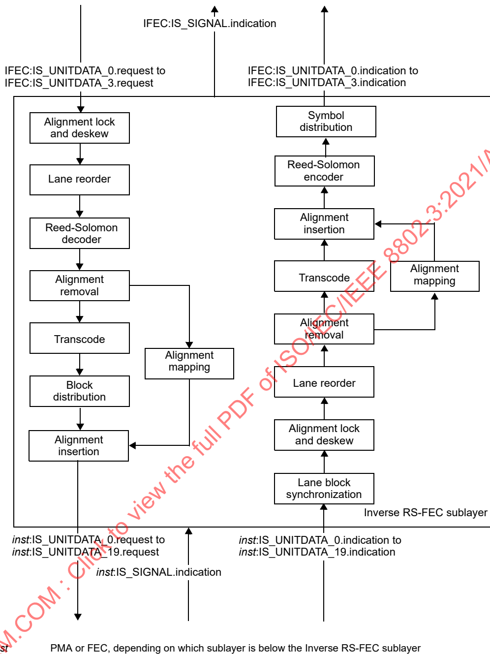
Figure 152-2—Inverse RS-FEC sublayer functional block diagram
